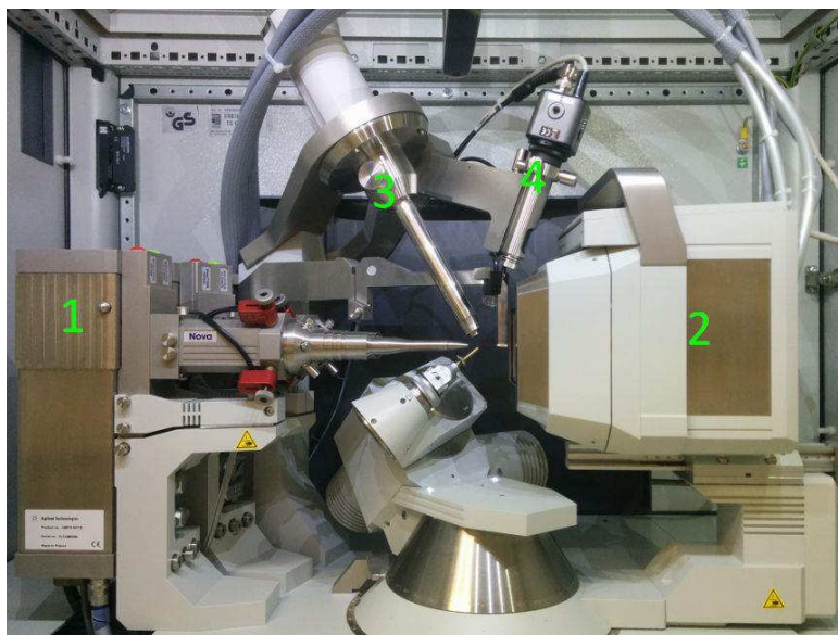
Figure 2.5: The inside chamber of the SuperNova (Agilent) diffractometer. 1) Sources of radiation - Copper X-ray tube (high intensity, large absorption by heavy atoms; suitable for organic compounds); Molybdenum X-ray tube (low intensity, low absorption by heavy atoms; suitable for actinide compounds). 2) Detector - CCD area detector. 3) Temperature control system - temperature ranges from 100 K (liquid nitrogen) to 500 K. 4) Camera.
