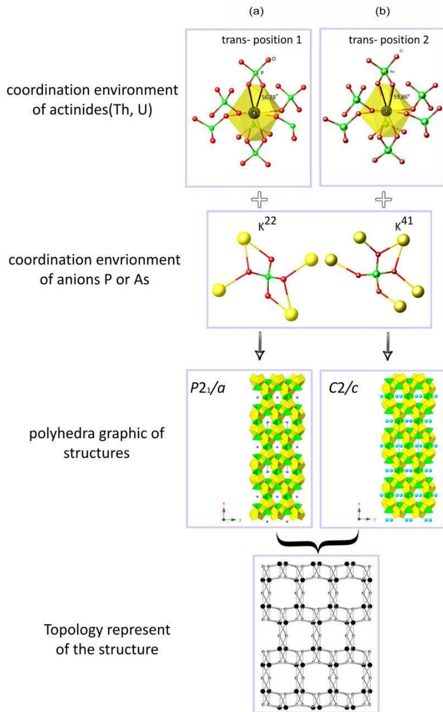
Figure 7.6: The comparison of the structure of (a) LiTh_2(PO_4)_3 (b) ATh_2(AsO_4)_3 ( A = K, Rb, Cs, Ag ) and BU^{IV}_2(PO_4)_3 ( B = Rb, Cs ). ThO_8 , As(P)O_4 coordination polyhedra are yellow and green, respectively, and O atoms are red; black dot is U atom, white dot is As(P) atom.
