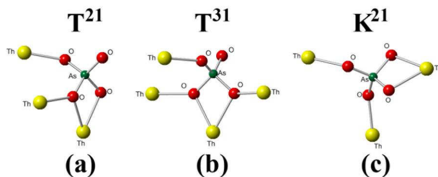
Figure 4.8: Coordination types of arsenate-anions in the crystal structures of \text{A}_2\text{Th}(\text{AsO}_4)_2 ( \text{A} = \text{Li}, \text{K}, \text{Rb}, \text{and Cs} ).
