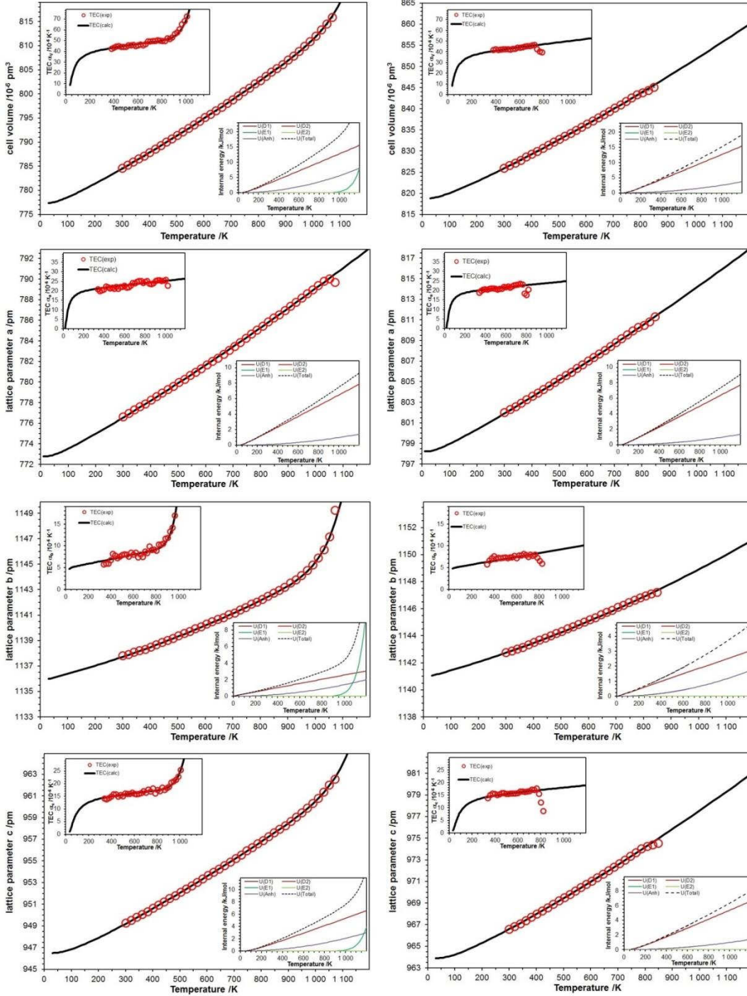
Figure 4.14: Temperature-dependent metric parameters and thermal expansion coefficients (TEC, inset top) together with the respective DEA fit results and single energy term contribution (insert bottom) for the X-ray powder data of room-temperature phases of K_2Th(AsO_4)_2 (left) and Rb_2Th(AsO_4)_2 (right).
