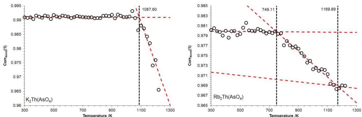
Figure 4.13: Temperature-dependent development of the autocorrelation parameter of K_2Th(AsO_4)_2 (left) and Rb_2Th(AsO_4)_2 (right) together with the respective evaluation of transition temperatures.
