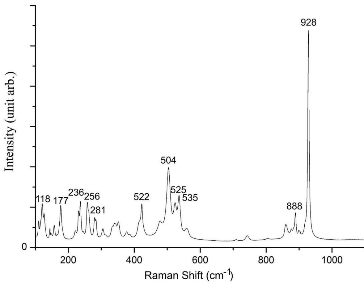
Figure 7.5: The Raman spectra of Raman spectrum of \text{Th}(\text{As}^{\text{III}}_4\text{As}^{\text{V}}_4\text{O}_{18}) .
