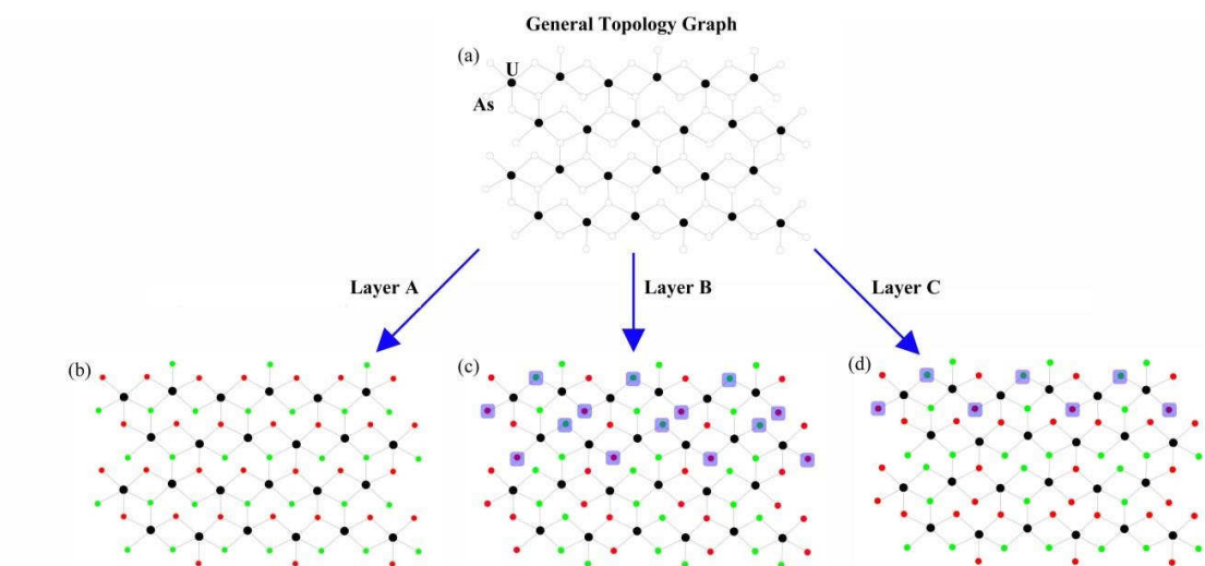
Figure 3.7: (a) Black-and-white graph of the [\text{UO}_2(\text{AsO}_3\text{OH})(\text{AsO}_2(\text{OH})_2)]^- layer. Colored graph of (b) A-layers, (c) B-layer and (c) C-layer. U sites are black circles, As sites are white circles on (a). Green circles are “up” and red are “down” As tetrahedra sites (see text for details). During the topotactic dehydration of RbUAs-1 and RbUAs-2 , the marked As tetrahedra in layers B and C have to change their orientation.
