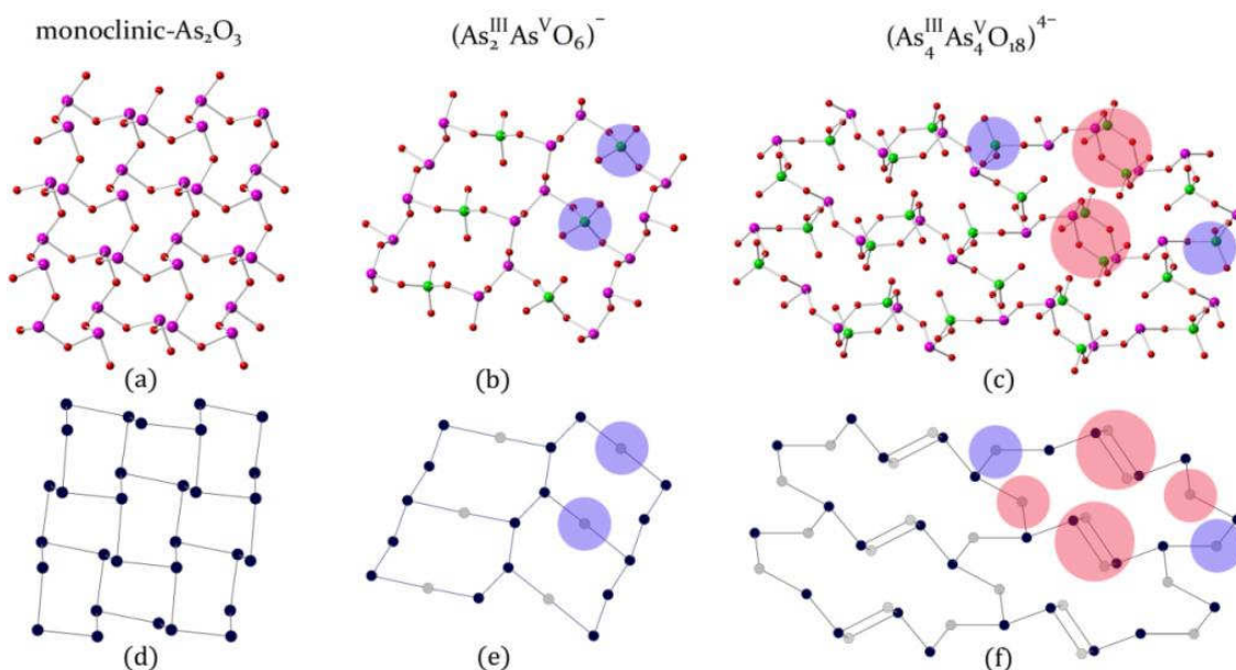
Figure 7.4: The arsenic layers (a–c) and their graph representation (d–f) in the crystal structures of monoclinic- \text{As}_2\text{O}_3 , \text{As}_2^{\text{III}}\text{As}^{\text{V}}\text{O}_5(\text{OH}) , and \text{Th}(\text{As}_4^{\text{III}}\text{As}_4^{\text{V}}\text{O}_{18}) . The color scheme is the same as in Fig. 7.3. Blue and red transparent circles marks nodes and corresponding \text{AsO}_4 tetrahedra and \text{As}_2^{\text{III}}\text{As}^{\text{V}}\text{O}_9 ring fragments that are implemented in the edges of initial \text{As}_2\text{O}_3 layer on each step in the (d) – (e) – (f) series.
