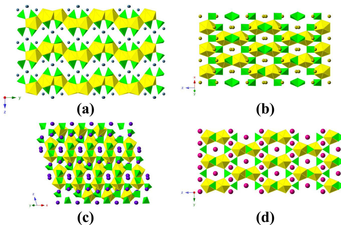
Figure 4.7: Polyhedra representation of the crystal structures of \text{Li}_2\text{Th}(\text{AsO}_4)_2 (a), \text{Na}_2\text{Th}(\text{AsO}_4)_2 (b), \text{K}_2\text{Th}(\text{AsO}_4)_2 (c), and \text{Cs}_2\text{Th}(\text{AsO}_4)_2 (d). \text{Rb}_2\text{Th}(\text{AsO}_4)_2 is isostructural with \text{K}_2\text{Th}(\text{AsO}_4)_2 . Th and As polyhedra are shown in yellow and green, respectively, alkaline atoms as colored spheres.
