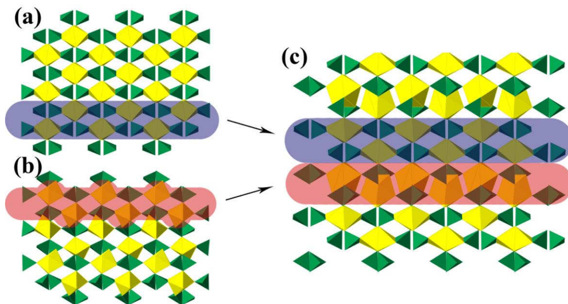
Figure 4.10: Comparison of the crystal structures of \text{Na}_2\text{Th}(\text{PO}_4)_2 (c) and \text{A}_2\text{Th}(\text{AsO}_4)_2 ( \text{A} = \text{Na}, \text{K} ) (a, b, respectively) along [100] . Th and As polyhedra are shown in yellow and green, respectively.
