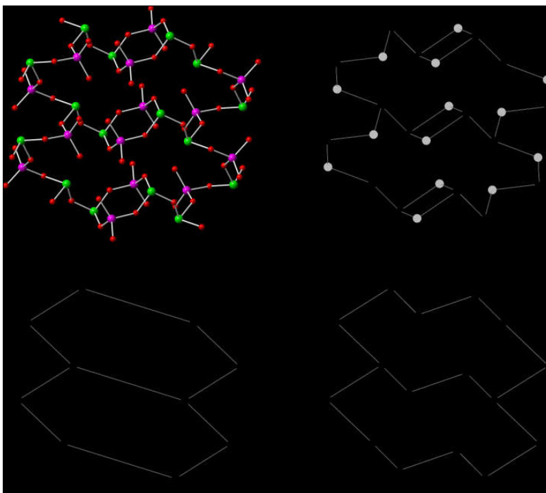
Figure 7.3: The simplification procedure applied to the (\text{As}^{\text{III}}_4\text{As}^{\text{V}}_4\text{O}_{18})^{4-} layers. O, \text{As}^{\text{III}} and \text{As}^{\text{V}} atoms are red, green, and magenta, respectively. In graph representation, \text{As}^{\text{III}} and \text{As}^{\text{V}} nodes are black and grey, respectively.
