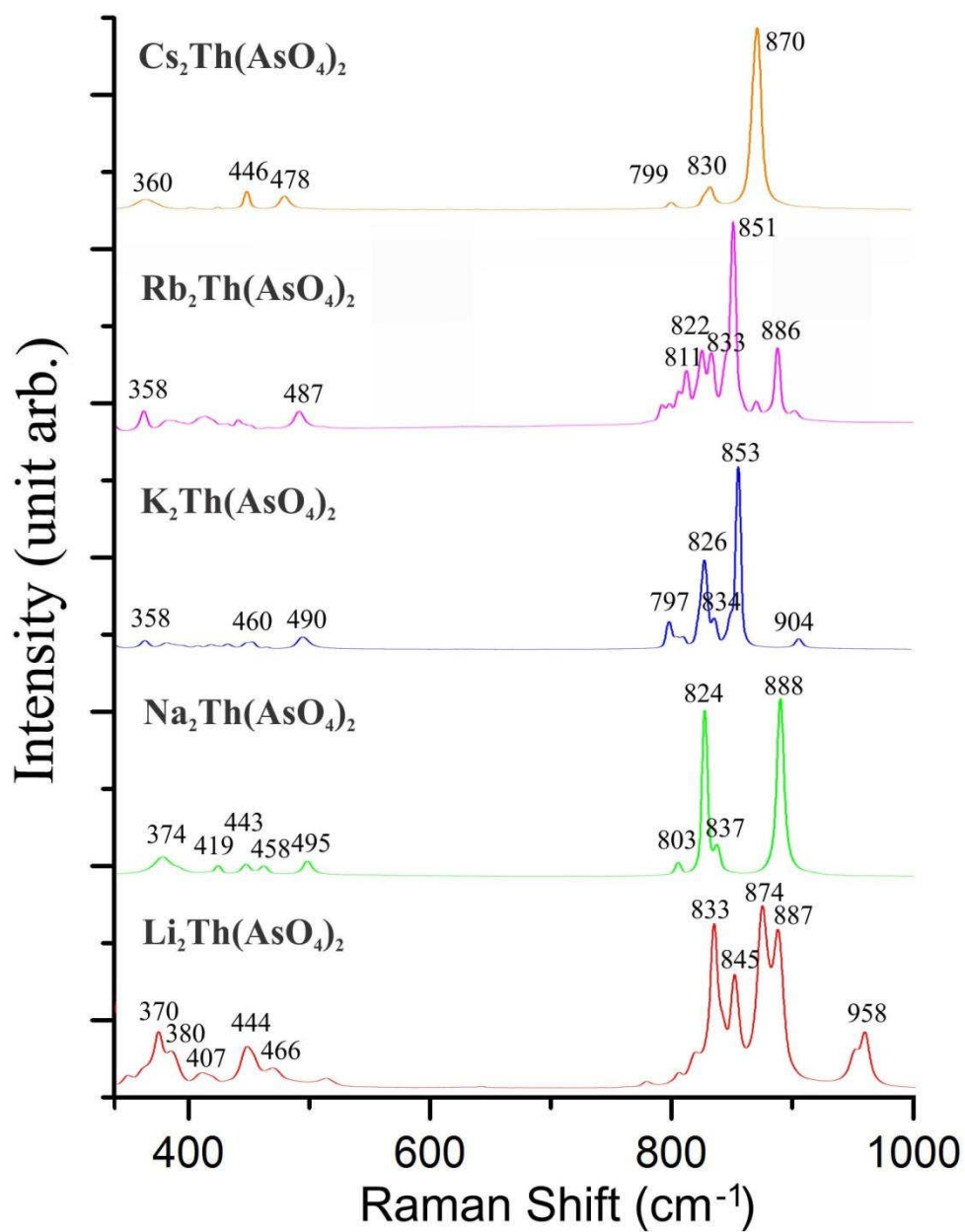
Figure 4.16: Raman spectra of \text{A}_2\text{Th}(\text{AsO}_4)_2 ( \text{A} = \text{Li}, \text{Na}, \text{K}, \text{Rb}, \text{Cs} ).
