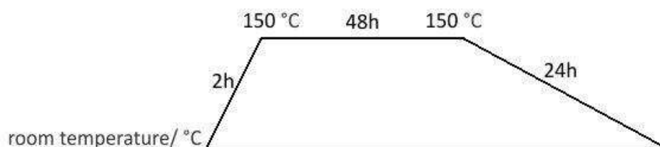
Figure 3.1: The tempering profile of the furnace.
