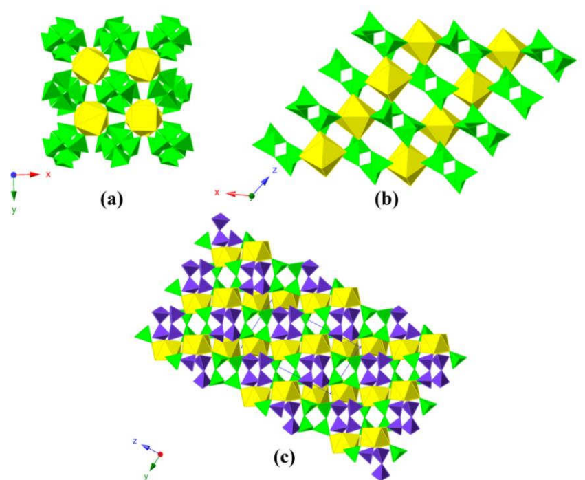
Figure 6.2: Crystal structure of tetragonal U(PO_3)_4 (a), (U_{0.62}Nd_{0.38})(PO_3)_4 (b), and Th(P_4O_{12}) (c). Th(P_4O_{12}) and U(P_4O_{12}) are isostructural. U, U/Nd, and Th sites are yellow. PO_4 polyhedra are green (a and b) or purple. Green or purple (c) PO_4 tetrahedra are to show plain and distorted P_4O_{12} groups, respectively. O atoms omitted for clarity.
