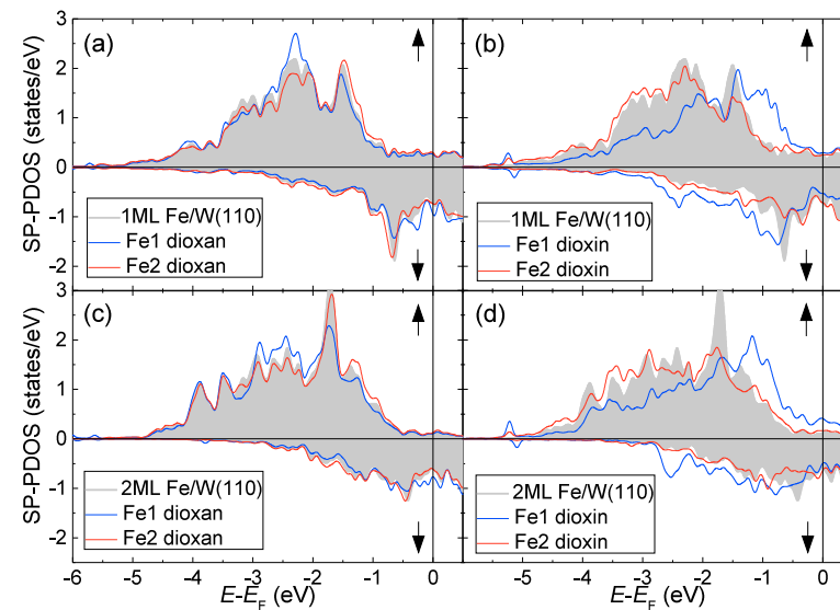
Figure 6.9.: SP-PDOS of the Fe1 and Fe2 d -states for dioxan and dioxin on 1 ML Fe/W(110) (a), (b) and on 2 ML Fe/W(110) (c), (d), respectively. As a reference, also the SP-PDOS of a clean surface Fe atom of the respective surface is given as gray shaded area.
