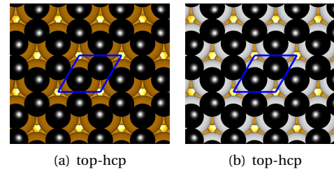
Figure C.1.: Top-hcp adsorption position for Gr on 1 ML Fe (a) or Co (b) on the Cu(111) substrate. The unit cell of each system is marked by the blue parallelogram. Color code of the surface atoms same as in Figs. 5.2, 5.3, 7.2 and B.1.
