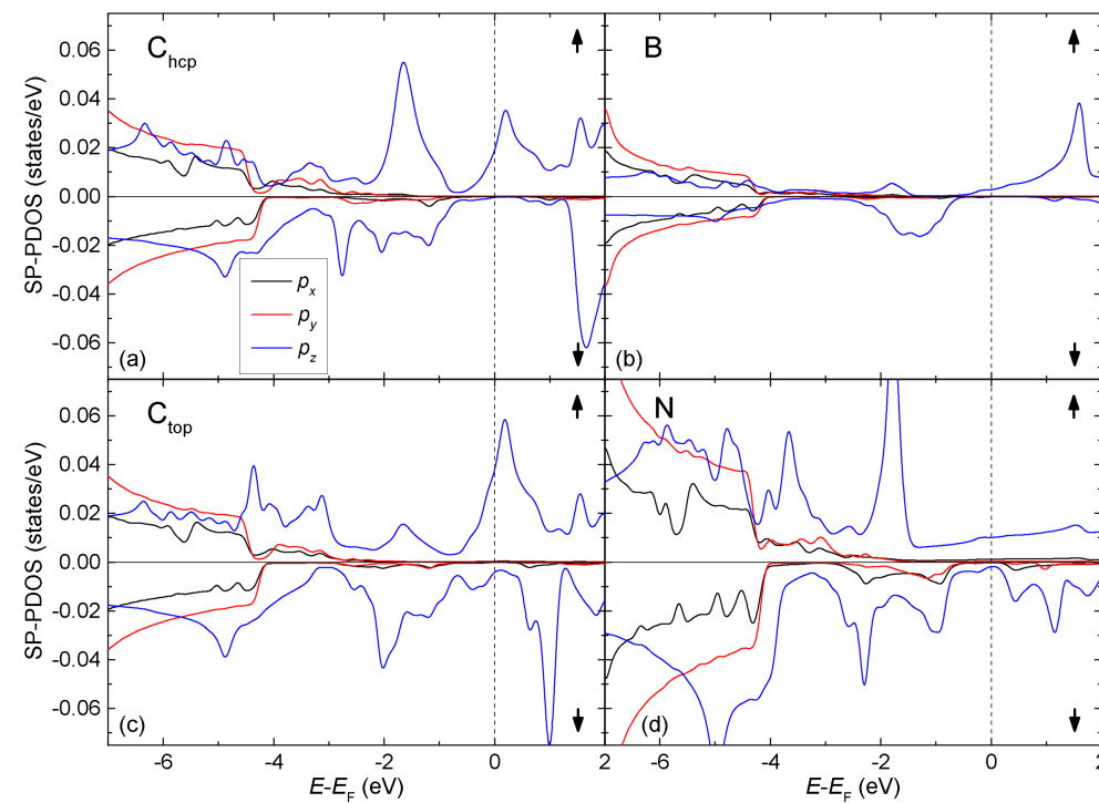
Figure 7.8.: SP-PDOS of the p -states for the C_{\text{hcp}}/\text{B} (a), (b) and C_{\text{top}}/\text{N} (c), (d) atoms for Gr and hBN on Co(111), respectively.
