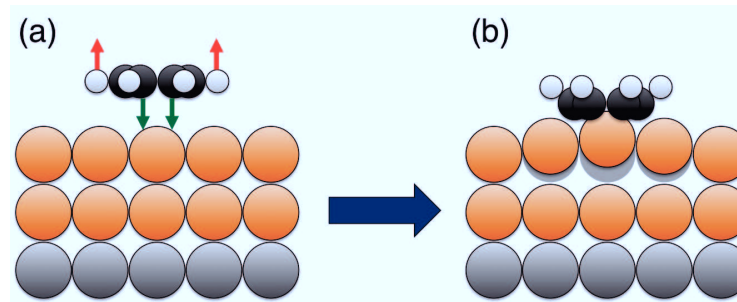
Figure 6.8.: Mechanism of the inter-layer magnetic softening due to the molecular induced skyhook effect. The different parts of the molecule interact differently with the substrate (a): whereas the H atoms are repelled from the substrate, the central part of the molecule is attracted to chemically interact with the surface atoms. This results in a geometric detaching of the first layer Fe atoms below the molecule with respect to the Fe atoms of the second layer leading to a decrease of the inter-layer exchange coupling (b).
