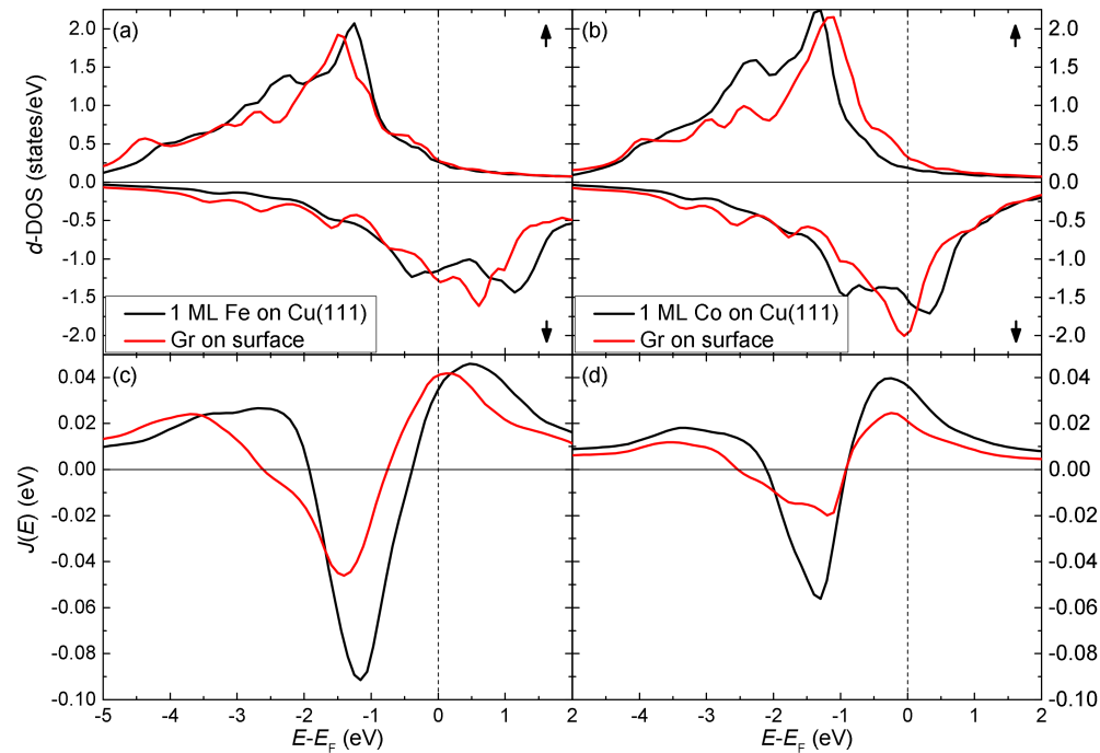
Figure C.3.: d -SP-DOS (a, b) and energy-dependent coupling constants (c, d) for the first layer magnetic atoms for Gr on 1 ML Fe, Co on the Cu(111) substrate, respectively. In addition the respective clean surface reference data are also included.
