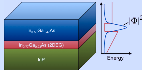
Figure 9.1.: Schematic representation of a III-V quantum-well heterostructure. The 2DEG forms due to a localization of the electron density ( |\Phi|^2 ) within the potential well of the strained In 0.77 Ga 0.23 As layer (based on a figure in Ref. [312]).
