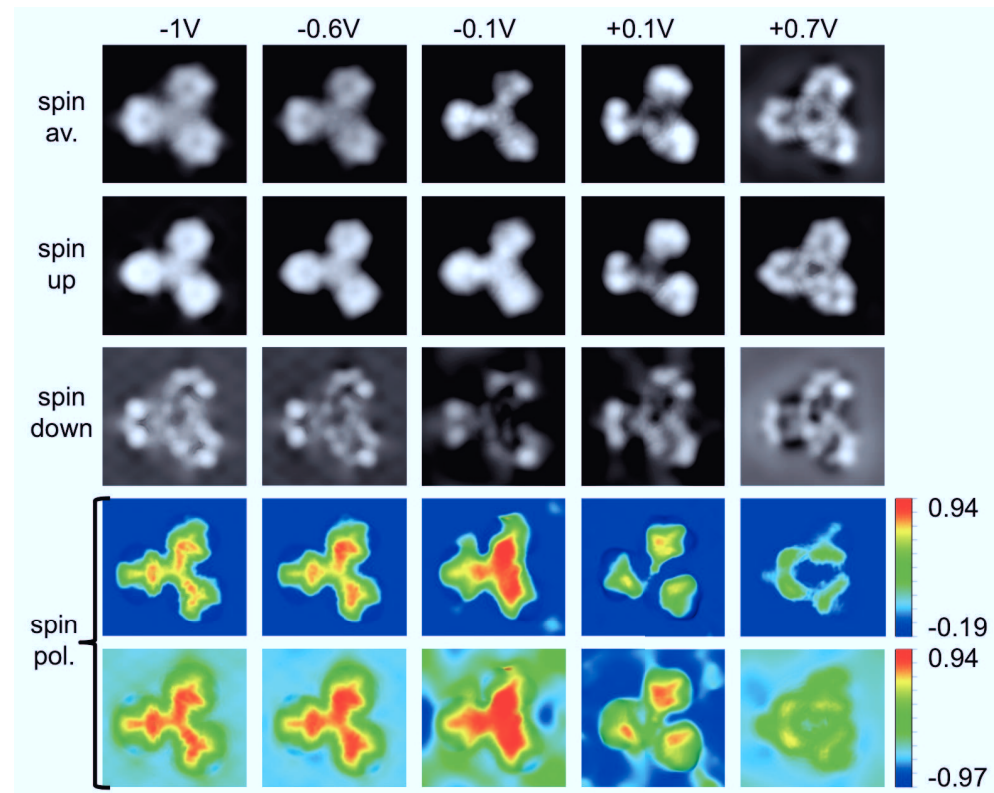
Figure 8.5.: Overview of the simulated STM topography images for TPT on 2 ML Fe/W(110) at different bias voltages. In the first row the spin averaged topography images are presented. In the second and third rows the images for the spin up and spin down channel are given, respectively. The last two rows show the calculated spin polarization according to Equation (4.4) at the different bias voltages for two different ranges of the polarization scale. The spin averaged, spin up and spin down images at -1 V, -0.6 V and +0.7 V are displayed for an isovalue of 3.37 \cdot 10^{-5} e/\text{\AA}^3 , at -0.1 V for 3.37 \cdot 10^{-6} e/\text{\AA}^3 and at +0.1 V for 2.02 \cdot 10^{-6} e/\text{\AA}^3 . All images for the spin polarizations were made for an isovalue of 6.75 \cdot 10^{-6} e/\text{\AA}^3 colored with the degree of spin polarization at each point. The scale bars to the right of the last two rows indicate the respective range of spin polarization. The orientation of the TPT molecule on the surface is in every case the same as in Fig. 8.3(a).
