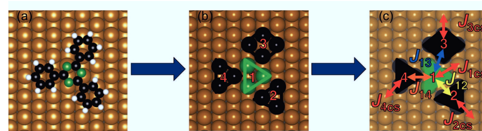
Figure 8.8.: The interaction of TPT with the 2 ML Fe/W(110) surface (a) is confined to the thirteen Fe atoms directly bound to it (b). Below the different rings of the molecule magnetic units are formed which are labeled as 1 to 4. To calculate the magnetic exchange coupling constants for the different units, the couplings between the units and from each unit to the clean surface need to be considered as assigned in (c).
