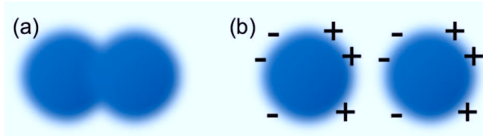
Figure 2.1.: Schematic visualization of overlapping (a) and non-overlapping (b) density distributions. In (b) charge fluctuations can give rise to induced dipole moments contributing to the vdW interaction.
