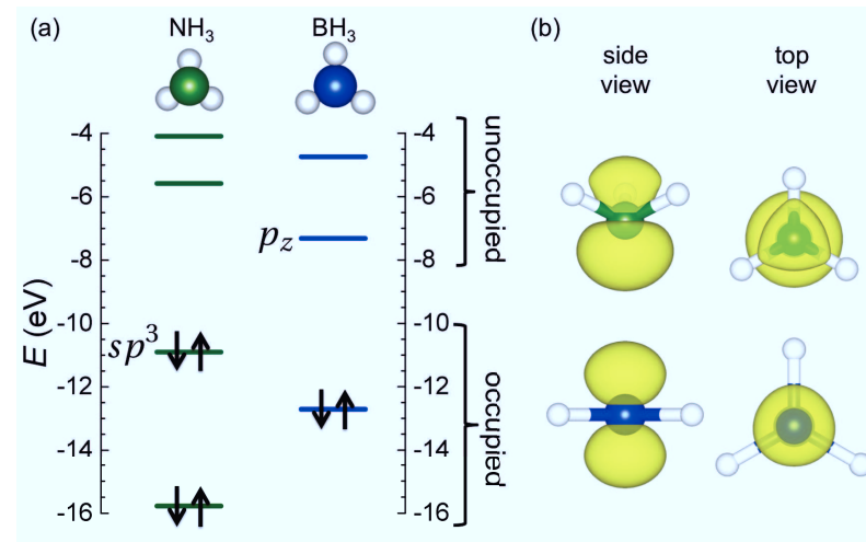
Figure 9.3.: Energy level diagram (a) and isosurface plots of the charge density of the HOMO/LUMO for \text{NH}_3/\text{BH}_3 in side and top view (b). The HOMO of \text{NH}_3 is a free electron pair in an sp^3 -like orbital (upper part in (b)) and the LUMO of \text{BH}_3 is an empty p_z -like state (lower part in (b)). The occupation of the states is marked by arrows. Note that the HOMO of each molecule is aligned at the calculated IP of 10.91 eV and 12.71 eV for \text{NH}_3 and \text{BH}_3 , respectively. The isosurface plots were made for an isovalue of 2.02 \cdot 10^{-1} e/\text{\AA}^3 . Color code for atoms same as in Fig. 5.2.
