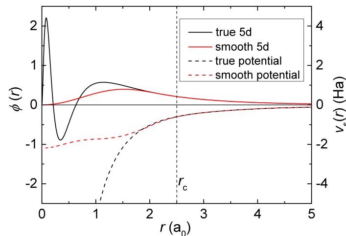
Figure 2.2.: Visualization of the PP approach for the W atom. The true effective potential is singular at the origin whereas the associated smooth potential has a finite value at r = 0 and is much smoother and weaker than the true potential. Consequently, the radial part of the true 5d state of W varies much more rapidly than the corresponding nodeless smooth part. The data was obtained from the GPAW setup for W [126].
