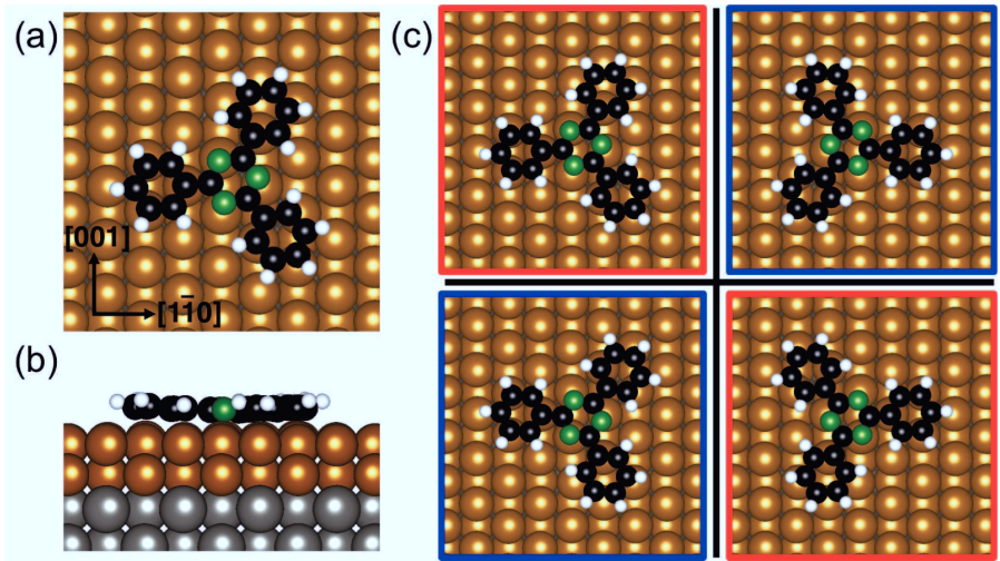
Figure 8.3.: Ground state geometry for TPT on 2 ML Fe/W(110) in top view (a) and side view (b), respectively. In (c) the mirror images of the structure along horizontal and vertical mirror planes are displayed. Only the pairs surrounded by either a red- or blue-frame can be overlaid by a 180° rotation, i. e. they are identical. When comparing red-framed and blue-framed structures it turns out that these geometries are different enantiomers that cannot be superimposed onto one another.
