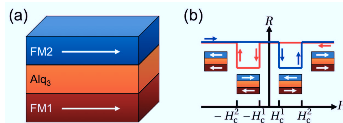
Figure 4.6.: Schematic picture of a vertical spin-valve device with an organic spacer as used in Ref. [22] (a). When the two ferromagnetic materials have different coercive fields H_c^1 and H_c^2 a characteristic resistance change with applied magnetic field H is typical for spin-valve behavior (b). In the initial state a parallel alignment of the magnetizations in the ferromagnetic layers is assumed. If one then increases the field (blue curve) the first layer will reverse its magnetization at H_c^1 giving rise to an antiparallel alignment which has a different resistance (here lower) than the parallel alignment. At H_c^2 also the harder magnetic layer reverses its magnetization which again gives rise to a parallel alignment and one switches back to the initial resistance state. When reducing the magnetic field the mechanism works accordingly (red curve).
