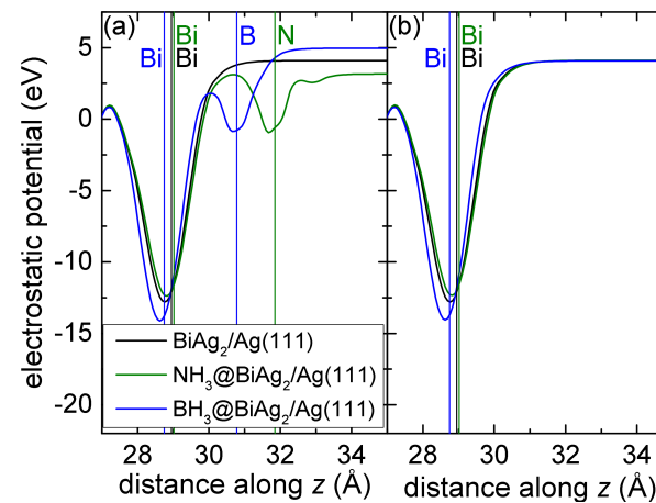
Figure 9.11.: Electrostatic potentials of the hybrid molecule-surface systems (a) and the molecular-induced geometries (b) for NH 3 and BH 3 on the BiAg 2 /Ag(111) surface alloy. The vertical lines in the figures indicate the positions of the respective first layer Bi, B and N centers along z . As a reference in (a) and (b) also the electrostatic potential of the clean BiAg 2 /Ag(111) surface alloy is included. Note that in each case the asymptotic value of the potential for large z -distances represents the calculated work function. For clarity in both diagrams the positions of the first layer Ag atoms are not indicated.
