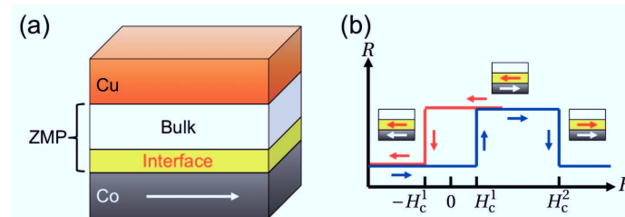
Figure 4.8.: Schematic representation of the device showing IMR [51] (a) made up of a bottom Co electrode, an interface region at the Co-ZMP boundary, the bulk part of the ZMP layer and a Cu top contact. Working principle of the IMR device (b): For large negative magnetic fields the bulk Co and the interface magnetization are aligned parallel leading to a low resistance state of the device. When the field is increased, the bulk Co layer switches at its coercive field H_c^1 giving rise to antiparallel alignment with higher resistance. At much larger fields also the hard interface magnetic layer reverses its magnetization at H_c^2 switching back to the low resistance state. Based on a figure in Ref. [51].
