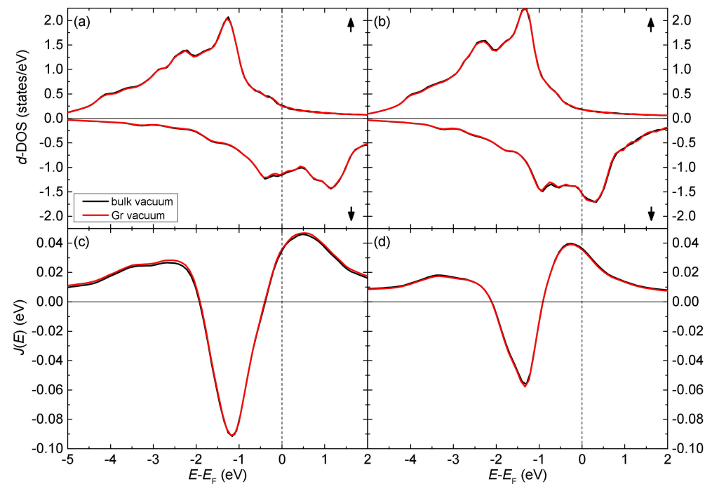
Figure C.2.: d -SP-DOS (a, b) and energy-dependent exchange coupling constants (c, d) for the first layer magnetic atoms of the clean 1 ML Fe, Co on Cu(111) surfaces, respectively. In all cases the results obtained from (i) structuring the vacuum region above and below the slab as continued bulk layers and (ii) by applying the Gr structure of the cells in the vacuum but leaving these cells empty, are included.
