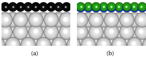
Figure 7.4.: Side view of the relaxed top-hcp geometry for Gr (a) and hBN (b) adsorbed on the Co(111) surface.
