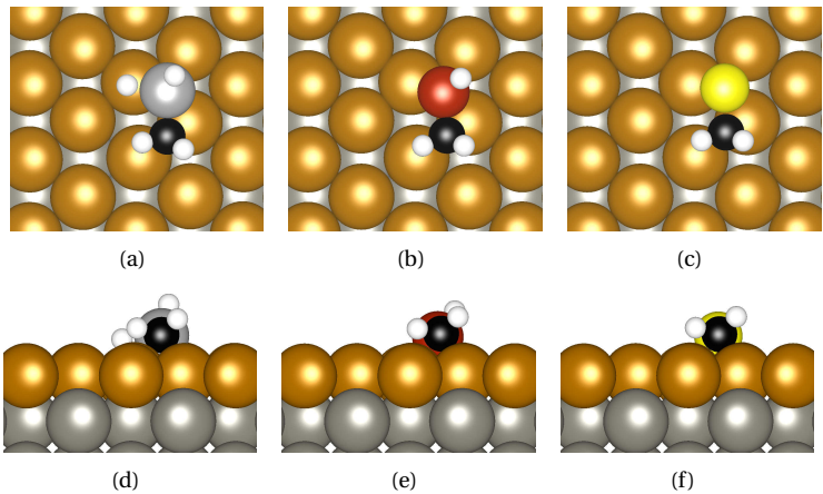
Figure A.5.: Optimized metastable structures for methylidenesilane (CH 4 Si) ((a), (d)), phosphethene (CH 3 P) ((b), (e)) and thioformaldehyde (CH 2 S) ((c), (f)) on 1 ML Fe/W(110) in top view and side view, respectively.
