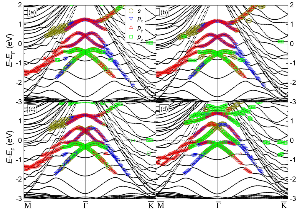
Figure 9.5.: Comparison of the band structures calculated for the clean BiAg 2 /Ag(111) surface alloy using different functionals: (a) band structure calculated with PBE including SOC for a geometry optimized with PBE without SOC, (b) band structure calculated with PBE including SOC for a geometry optimized with rev-vdW-DF2 without SOC, (c) band structure calculated with PBE including SOC for a geometry optimized with PBE with SOC and (d) band structure calculated with PBE including SOC for a geometry optimized with rev-vdW-DF2 with SOC. In each case the s -, p_x -, p_y - and p_z -orbital contributions (of at least 0.08 e in the PAW spheres) of states mainly located at the surface are plotted on top of the band structure.
