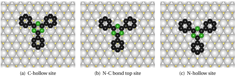
Figure B.1.: Investigated adsorption sites for TPT on 2 ML Co/Cu(111). Color code for molecular atoms same as in Fig. 5.2. Color code of the surface atoms: light gray for Co and orange for Cu.
