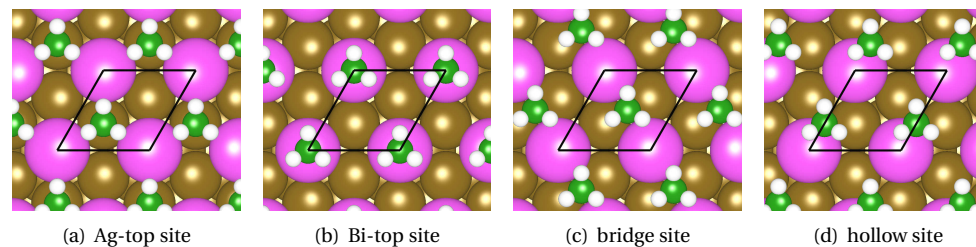
Figure 9.7.: Investigated adsorption sites for \text{NH}_3 and \text{BH}_3 on the \text{BiAg}_2/\text{Ag}(111) surface alloy for the exemplary case of \text{NH}_3 . The unit cell of each structure is marked by the black parallelogram.
