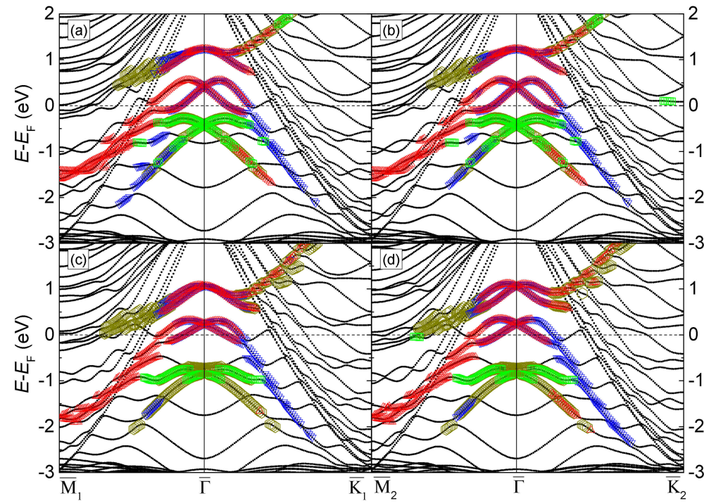
Figure 9.14.: Band structures calculated for the molecular-induced surface geometries: (a) band structure for the \text{NH}_3 -induced geometry along the \overline{\Gamma\text{M}_1} and \overline{\Gamma\text{K}_1} directions, (b) band structure for the \text{NH}_3 -induced geometry along the \overline{\Gamma\text{M}_2} and \overline{\Gamma\text{K}_2} directions, (c) band structure for the \text{BH}_3 -induced geometry along the \overline{\Gamma\text{M}_1} and \overline{\Gamma\text{K}_1} directions and (d) band structure for the \text{BH}_3 -induced geometry along the \overline{\Gamma\text{M}_2} and \overline{\Gamma\text{K}_2} directions. In each case the s -, p_x -, p_y - and p_z -orbital contributions (of at least 0.08\ e in the PAW spheres) of states mainly located at the surface are plotted on top of the band structure.
