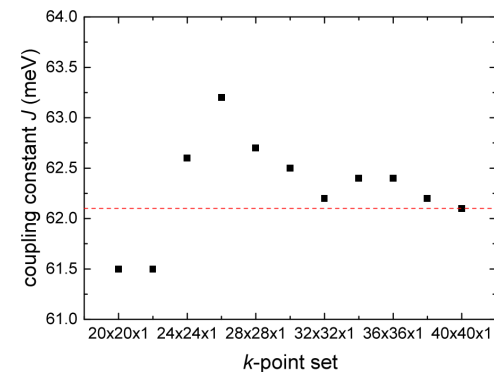
Figure A.9.: Convergence investigation of the clean surface inter-layer exchange coupling constant of the Co(111) surface with respect to the k -point set. The red dashed line corresponds to the value calculated with the largest number of k -points.
