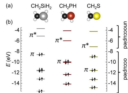
Figure A.4.: Atomic structure of methylidenesilane (CH 4 Si), phosphethene (CH 3 P) and thioformaldehyde (CH 2 S) (from left to right) (a). Calculated energy levels of the isolated molecules (b). Note that the HOMO of each system was aligned at the calculated IP of 8.61 eV, 9.98 eV and 9.02 eV for CH 4 Si, CH 3 P and CH 2 S, respectively. The bonding and antibonding \pi -states have been labeled \pi and \pi^* , respectively. The occupation of each state is indicated by arrows. Color code: white for H, black for C, gray for Si, dark red for P and yellow for S.
