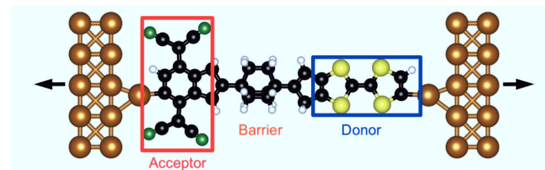
Figure 4.1.: A schematic representation of the rectifier molecule suggested by Aviram and Ratner [180] attached to two contacts. Due to the high electron affinity of the acceptor unit and the low ionization potential of the donor unit an electronic asymmetry is induced so that current is supposed to flow preferably from the left to the right side and not in the opposite direction. Both units of the molecule are isolated by a barrier between them to prevent interaction.
