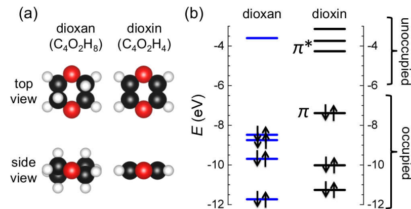
Figure 6.1.: Atomic structure of isolated dioxan and dioxin in top and side view (a) and calculated energy level diagram for both systems (b). In case of dioxin the bonding and antibonding \pi -states have been labeled \pi and \pi^* , respectively. The HOMO of each system was aligned at the calculated IP of 8.48 eV and 7.39 eV for dioxan and dioxin, respectively and the occupations of the levels are marked by arrows. Color code for atoms same as in Fig. 5.2.
