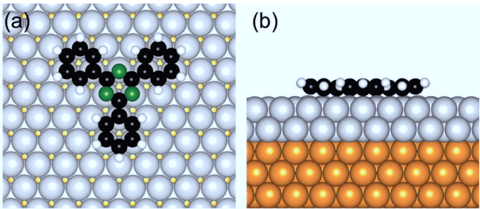
Figure B.2.: Optimized stable structure for TPT on 2 ML Co/Cu(111) in top view (a) and side view (b), respectively.
