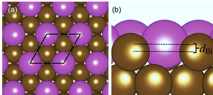
Figure 9.4.: Top (a) and side (b) view of the clean \text{BiAg}_2/\text{Ag}(111) surface alloy. The in-plane (\sqrt{3} \times \sqrt{3})R30^\circ surface unit cell is marked by the black parallelogram in (a). In (b) the outward buckling of the Bi out of the surface is labeled by d_{\text{Bi}} . Color code of the surface atoms: magenta for Bi and brown for Ag.
