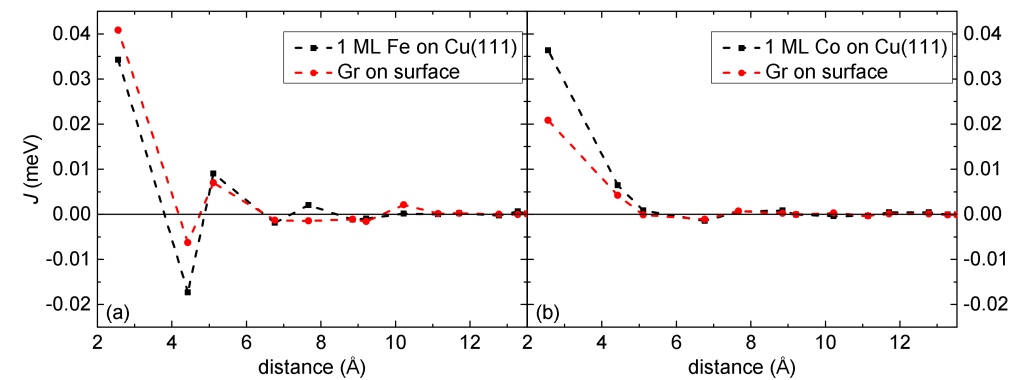
Figure C.4.: Distance dependence of the coupling constants for Gr on 1 ML Fe (a) and 1 ML Co (b) on the Cu(111) substrate. In addition also the respective clean surface data are included.
