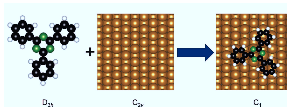
Figure 8.4.: Symmetry analysis for the TPT adsorption on 2 ML Fe/W(110). The isolated TPT molecule has D_{3h} symmetry, the clean surface has C_{2v} symmetry and the resulting adsorption geometry belongs to the C_1 point group, i. e. it lacks of any symmetry except of identity.
