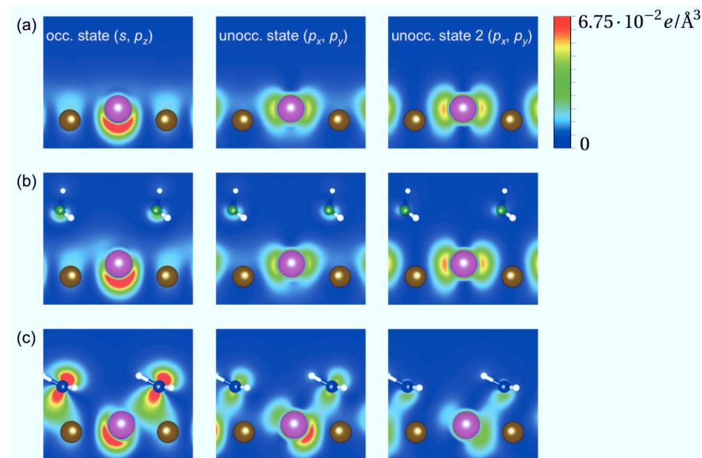
Figure 9.15.: Visualization of the charge density of the surface states at \bar{\Gamma} for the clean \text{BiAg}_2/\text{Ag}(111) surface alloy (a) and for \text{NH}_3 (b) as well as \text{BH}_3 (c) on the (110) and (100) planes marked as dashed lines in Fig. 9.8, respectively.
