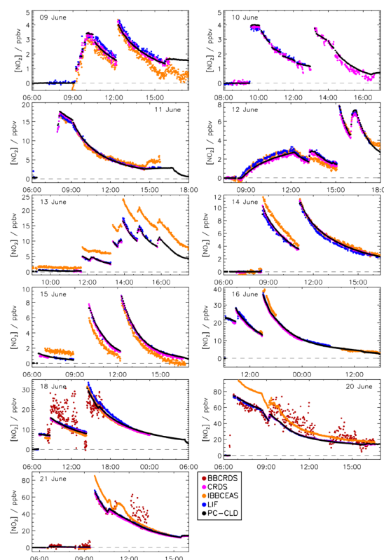
Fig. 4. Time series of NO 2 mixing ratios from all instruments. Data were averaged to a 1 min time resolution, if the original data set provided a higher temporal resolution. Only data which are used for the analysis are shown, e.g. data during the addition of trace gases were rejected in the analysis because of potential inhomogeneities of the trace gas in the chamber.
