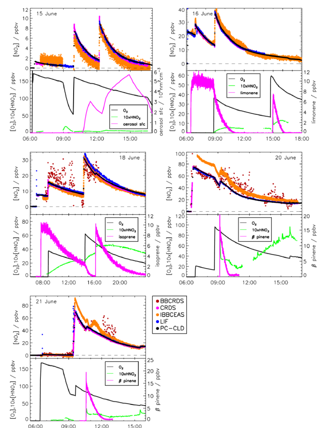
Fig. 3. Same as Fig. 2. In addition aerosol surface area measured by SMPS and mixing ratios and limonene, isoprene and β-pinene measured by PTRMS is shown.
