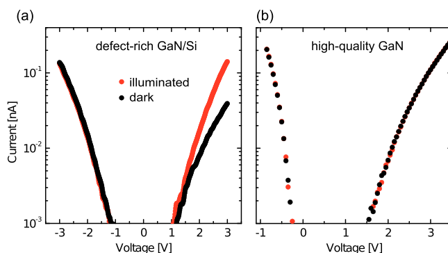
FIG. 4. Tunneling spectra acquired in the dark (black symbols) and under laser illumination (red symbols) (a) 30 nm away from the GaN/Si interface on the defect-rich GaN layer and (b) on the high quality GaN layers. (a) and (b) were acquired using mechanical and electronic optical choppers, respectively. The irradiances of the 405 nm laser were (a) \sim 2.5 \times 10^5 \text{ W m}^{-2} and (b) \sim 1.5 \times 10^5 \text{ W m}^{-2} . The tip-sample separations were defined by a voltage and current of (a) -3 \text{ V} and 150 \text{ pA} and (b) +3 \text{ V} and 100 \text{ pA} , respectively. The tip-sample separation is identical for the spectra in the dark and under illumination. Only for the defect rich GaN layer, sub-bandgap laser illumination increases the tunnel current, due to excitation of electrons from defect states.
