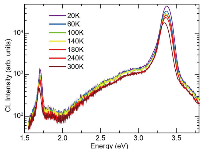
FIG. 2. Top-view cathodoluminescence spectra measured on the growth plane of the defect-rich GaN/Si sample at different temperatures.
