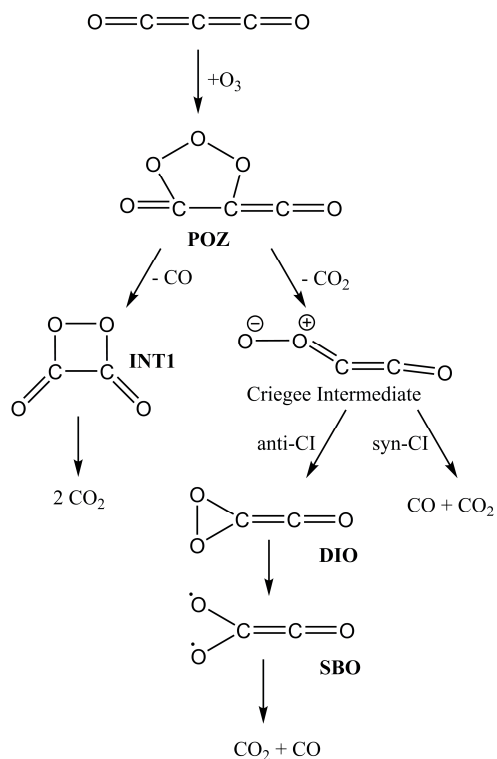
Figure 11: Simplified mechanism for the reaction of carbon suboxide with O 3 . Additional calculations are available in the supporting information.
