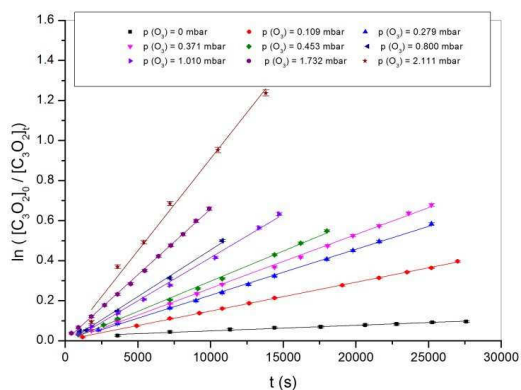
Figure 9: Relative concentration change of C 3 O 2 at various reaction times in the presence of 9 different O 3 concentrations. All experiments were performed at room temperature (~ 295 K) and at a pressure close to 1 bar.
