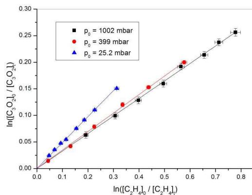
Figure 6: Depletion factors for C_3O_2 versus C_2H_4 during reaction of both trace gases with OH at three different pressures. Error bars are 2\sigma as returned by the least-squares fitting routine. The slope at each pressure yields the relative rate constant ratio k_4/k_5 .
