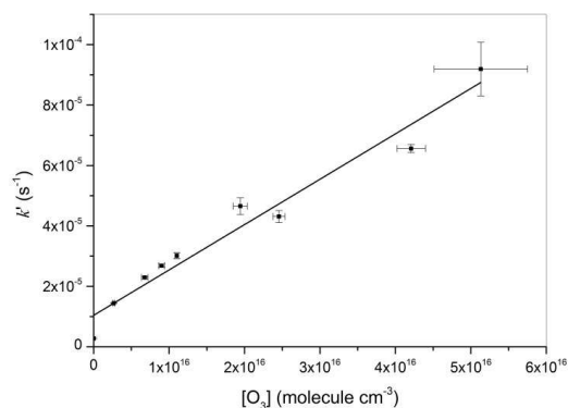
Figure 10: Pseudo-first-order decay constant of \text{C}_3\text{O}_2 plotted against the \text{O}_3 concentration. The slope is the bimolecular rate constant k_6 . The horizontal errors bars represent uncertainty in the \text{O}_3 concentration based on analysis of three different spectral regions (see text). The vertical error bars are 2\sigma from the fits to data as shown in Figure 9.
