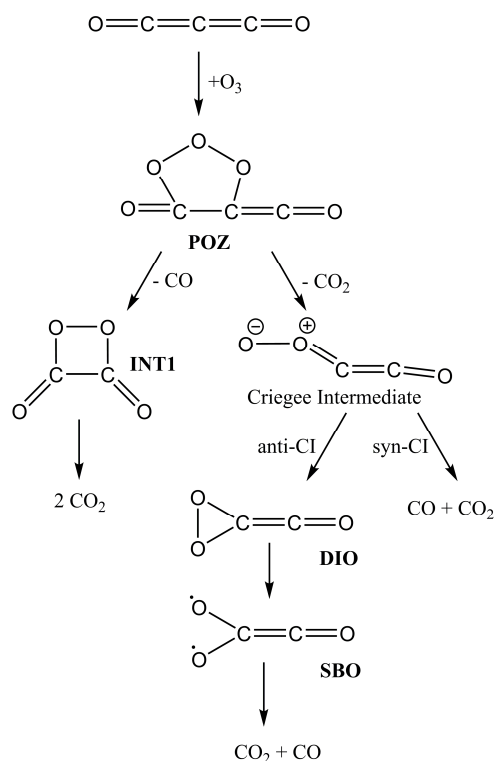
Figure 11: Simplified mechanism for the reaction of carbon suboxide with O 3 . Additional calculations are available in the supporting information.
