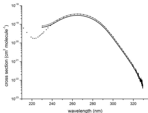
Figure 3: UV spectrum of C_3O_2 in the spectral range 210 to 330 nm. The dots are the spectrum reprinted with permission from Bayes (1961). (Copyright 1961 American Chemical Society). The thick black line is our spectrum; the thin black line was obtained by scaling our spectrum by a factor 1.17 (see text).
