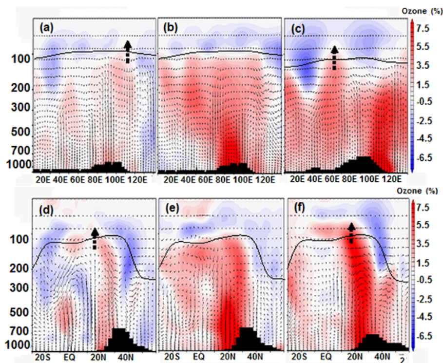
Figure 4. Longitude–pressure cross section of percentage ozone anomalies averaged for the monsoon season (June–September) obtained from (a) Ind38 (averaged over 8–35° N), (b) Ind73 (averaged over 8–35° N), and (c) Chin73 (averaged over 20–45° N) simulations. Latitude–pressure cross section of percentage ozone anomalies averaged for the monsoon season (June–September) obtained from (d) Ind38 (averaged over 70–90° E), (e) Ind73 (averaged over 70–90° E), and (f) Chin73 (averaged over 85–120° E) simulations. Black arrows indicate wind vectors. The vertical velocity field has been scaled by 300. The black line represents the tropopause, and the black dashed arrows indicate the cross-tropopause transport.
