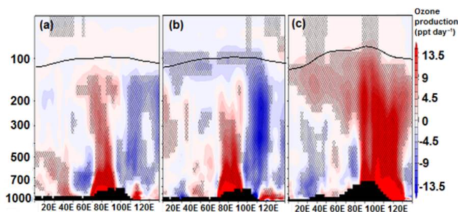
Figure 3. Longitude–pressure cross section of changes in net ozone production ( \text{ppt day}^{-1} ) due to enhanced \text{NO}_x with respect to the CTRL simulation, averaged for the monsoon season (June–September) obtained from (a) Ind38 (averaged over 8\text{--}35^\circ\text{N} ), (b) Ind73 (averaged over 8\text{--}35^\circ\text{N} ), and (c) Chin73 (over 20\text{--}45^\circ\text{N} ) simulations. The black line shows the tropopause while black hatched lines indicate 95 % confidence level.
