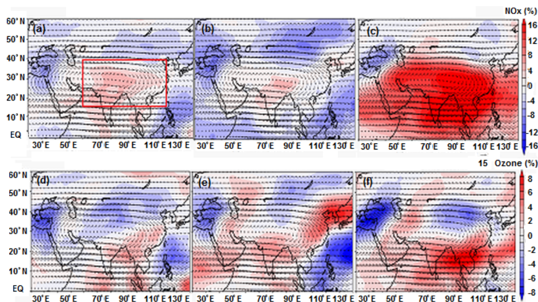
Figure 5. Latitude–longitude cross section of percentage \text{NO}_x anomalies averaged for the monsoon season (June–September) at 110 hPa obtained from (a) Ind38, (b) Ind73, and (c) Chin73 simulations. (d–f) show the same but for percentage ozone anomalies at 110 hPa for the (d) Ind38, (e) Ind73, and (f) Chin73 simulations. Black arrows indicate horizontal winds at 110 hPa. The red box in (a) indicates the ASM anticyclone region used to compute the associated radiative forcing regional average.
