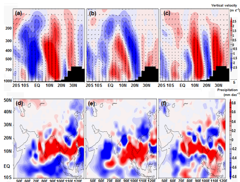
Figure 9. Difference in the meridional circulation due to enhanced \text{NO}_x emissions averaged for the monsoon season (June–September) and over 70\text{--}100^\circ\text{E} for (a) Ind38-CTRL, (b) Ind73-CTRL, and (c) Chin73-CTRL simulations. Shaded contours indicate the anomalies in vertical velocity ( \text{m s}^{-1} ). The vertical velocity field has been scaled by 300. Precipitation anomalies ( \text{mm day}^{-1} ) averaged for the monsoon season (June–September) obtained from (d) India38-CTRL, (e) Ind73-CTRL, and (f) Chin73-CTRL simulations.
