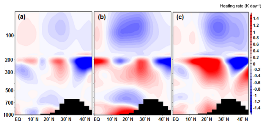
Figure 7. Latitude–pressure distribution of ozone heating rate changes (in K day −1 ) for the (a) Ind38 (averaged over 70–100° E), (b) Ind73 (averaged 70–100° E), and (c) Chin73 (averaged over 70–100° E) perturbed simulations, compared to the CTRL simulation.
