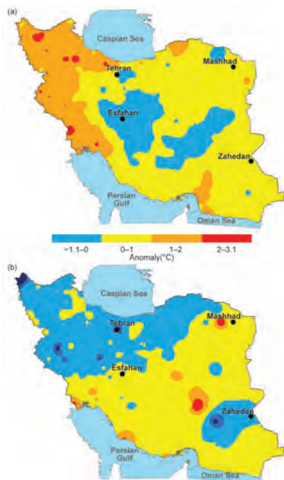
FIG. 7.49. Seasonal mean surface temperature anomalies ( ^{\circ}\text{C} ) in (a) summer (Jun–Aug) and (b) autumn (Sep–Nov). (Source: I.R. of Iran Meteorological Organization & National Center for Drought and Disaster Risk Management.)
