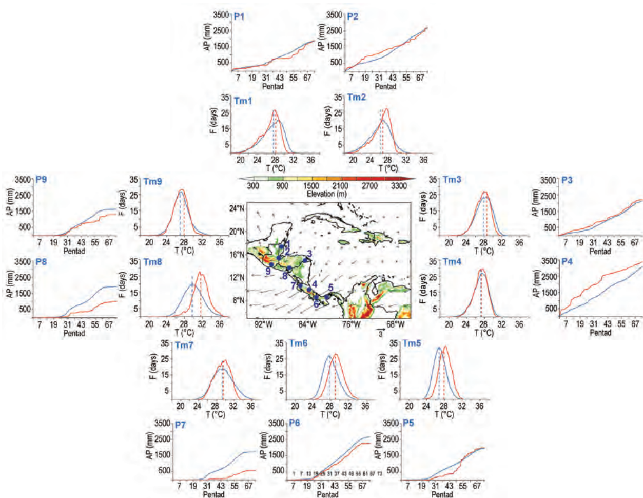
FIG. 7.8. Mean surface temperature (Tm) frequency (F; days) and accumulated pentad precipitation (P; mm) time series are shown for nine stations (blue dots) in Central America: (1) Philip Goldson International Airport, Belize; (2) Puerto Barrios, Guatemala; (3) Puerto Lempira, Honduras; (4) Puerto Limón, Costa Rica; (5) Tocumen International Airport, Panamá; (6) David, Panamá; (7) Liberia, Costa Rica; (8) Choluteca, Honduras; and (9) Puerto San José, Guatemala. The blue solid line represents the 1981–2010 average values and the red solid line shows 2015 values. Vertical dashed lines depict the mean temperature for 2015 (red) and the 1981–2010 period (blue). Vectors indicate July wind anomalies at 925 hPa (1981–2010 base period). Shading depicts regional elevation (m). (Source: NOAA/NCEI and Central American NWS.)
