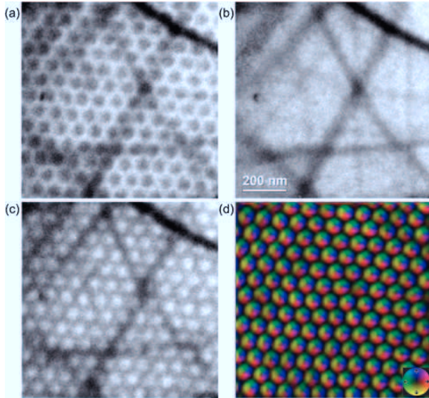
Fig. 2. Transport of intensity equation analysis of a magnetic skyrmion lattice in FeGe recorded at 220 K in the presence of 100 mT magnetic field. (a–c) Fresnel defocus images recorded at defocus values of -200 , 0 , and +200 \mu\text{m} , respectively. (d) Magnetic induction map generated from the gradients of the phase distribution recovered from images (a–c) using the transport of intensity equation
