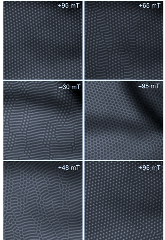
Fig. 3. Overfocus Fresnel images (defocus \sim 1 mm) recorded at specimen temperature of 240 K, demonstrating in situ switching of skyrmion polarity by applying the indicated magnetic fields to the sample using the objective lens of the TEM
