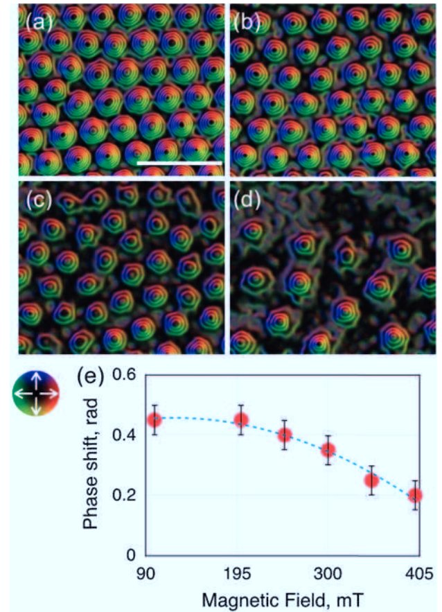
Fig. 6. Magnetic induction maps recorded using off-axis electron holography showing the magnetic field dependence of a skyrmion lattice at 200 K, shown for applied magnetic fields of (a) 200, (b) 300, (c) 350, and (d) 400 mT. The magnetic phase contour spacing is 2\pi/64 = 0.098 radians. The scale bar is 200 nm. (e) Magnetic phase shift of individual skyrmions measured at different magnetic fields
