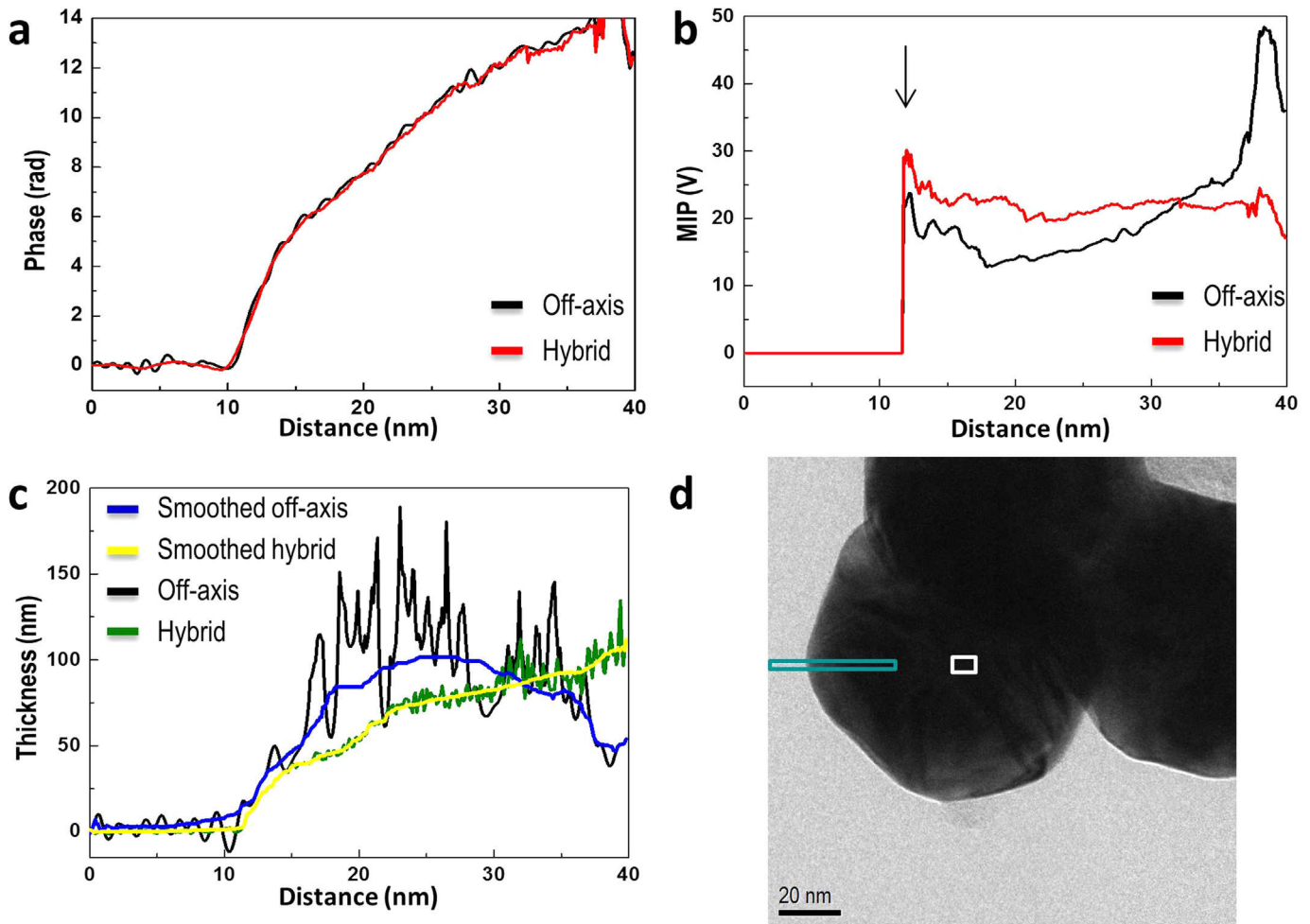
Fig. 2. (a) Phase and (b) MIP profiles obtained using off-axis and hybrid electron holography, respectively, from the region shown in (d) the black arrow in (b) indicates the edge of the specimen. (To the left of the arrow there is vacuum). (c) Specimen thickness profiles determined using the different techniques from the measured amplitude profiles. (d) Bright-field image showing the areas from which the profiles were extracted.
