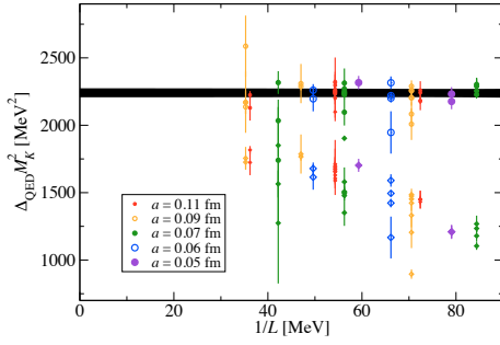
Figure 1: The Kaon splitting with and without the subtraction of the universal part of the finite volume corrections. The faded points are uncorrected and the solid points are corrected. The black line is a fit to the remaining finite volume dependence with a L^{-3} ansatz. The gray band is the statistical error. All points have been projected to the physical point in all but one finite volume direction by the fit function.
