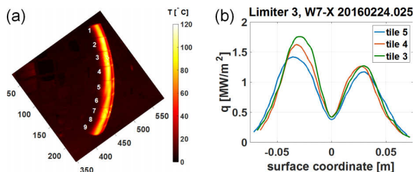
FIG. 6. (a) Infrared image of limiter in module 5 shows heterogeneous temperature distribution due to 3D structure of the scrape-off layer; (b) heat flux density profiles calculated at three tiles of limiter in module 3.
