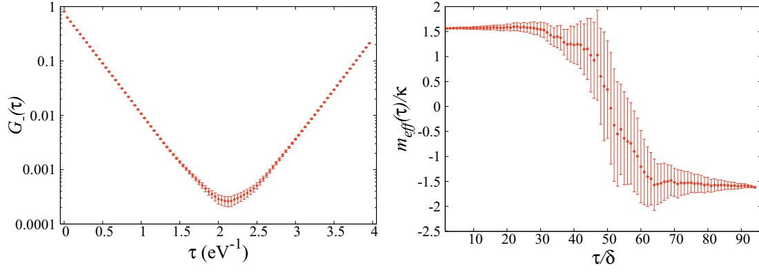
FIG. 5. Example of G_-(\tau) correlator (left panel) with momentum |\vec{T}|(|k_\parallel|, |k_{\perp,i}|) = (\frac{2\pi}{3}, \frac{4\pi}{3\sqrt{3}}) . The corresponding effective mass plot (in units of hopping parameter \kappa ) is given underneath with \Delta = 2 (right panel). Calculations were performed with N_L = 9 and N_t = 96 .
