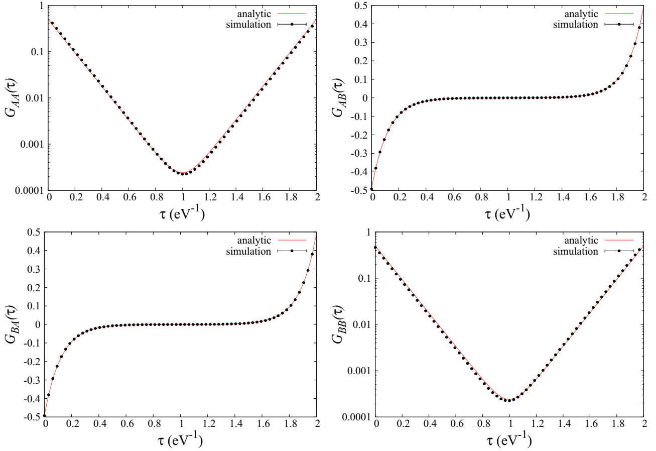
FIG. 12. The matrix of correlators G_{ij}(\tau) for the two-site Hubbard model with \beta = 2 \text{ eV}^{-1} and \kappa = 2.7 \text{ eV} , and U/\kappa = 2 . The solid lines are the analytical results. The points are from a full lattice calculation with N_t = 64 time steps. Error bars, obtained via bootstrap, are too small to be visible.
