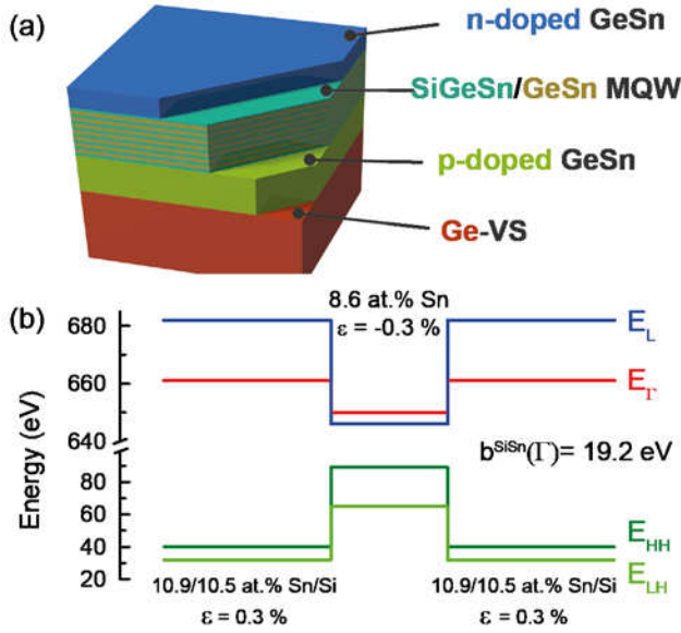
Figure 6. (a): Schematic overview on the grown MQW heterostructure. (b): Bandstructure calculations show the carrier confinement of both electrons and holes in the active well region.
