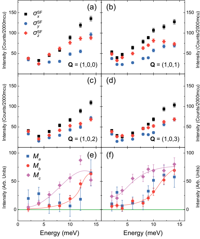
FIG. 2. Constant- Q scans of \sigma_x^{\text{SF}} , \sigma_y^{\text{SF}} , and \sigma_z^{\text{SF}} at Q = (1, 0, L) for (a) L = 0 , (b) L = 1 , (c) L = 2 , and (d) L = 3 measured at 2 K. By using the measured cross sections in panels (a)–(d), M_a , M_b , and M_c are obtained for (e) even and (f) odd L . The solid lines are to guide the eye.
