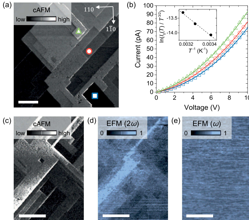
FIG. 1. Transport properties of strained \text{SrMnO}_3 probed by scanning probe microscopy. (a) cAFM scan obtained with a sample bias of 0.2 V, revealing nanodomains of varying conductance. Scale bar, 2 \mu\text{m} . (b) Local I(V) curves recorded at the spots marked in (a). Solid lines represent fits to the I(V) curves according to Eq. (2). The inset shows an Arrhenius plot of the temperature-dependent fit constant I_0(T) of Eq. (2) from measurements on a single domain. (c) cAFM image recorded at a different sample position. Scale bar, 5 \mu\text{m} . (d) Normalized EFM( 2\omega ) image obtained at the same sample position shown in (c). The EFM scan reveals the spatial distribution of mobile charge carriers, imaged in the non-contact mode. Scale bar, 5 \mu\text{m} . (e) Corresponding EFM( \omega ) image recorded at the same position as the scans in (c) and (d) reflecting a homogeneous electrostatic surface potential with no indication of domain-related stationary charges. Scale bar, 5 \mu\text{m} .
