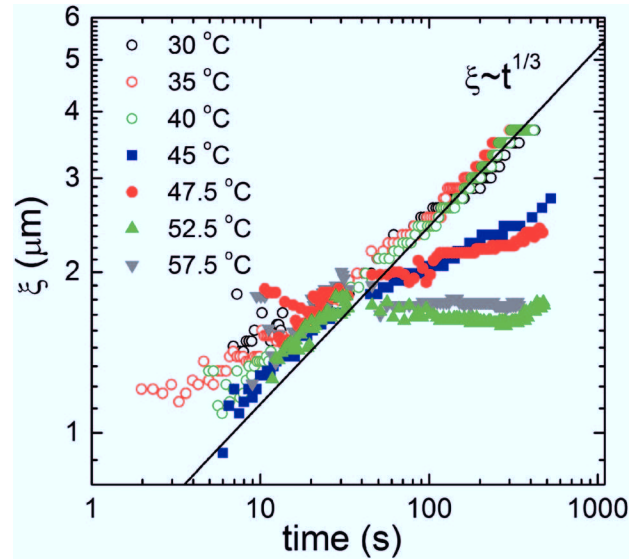
Fig. 7 Plots of the characteristic length as a function of time for a dense liquid phase prepared from a 175\text{ mg mL}^{-1} BSA with 44\text{ mM YCl}_3 parent solution at room temperature. The values of T_{\text{jump}} are shown in the figure. Above 40^\circ\text{C} a significant slowdown of the kinetics is observed and an arrested state is reached.
