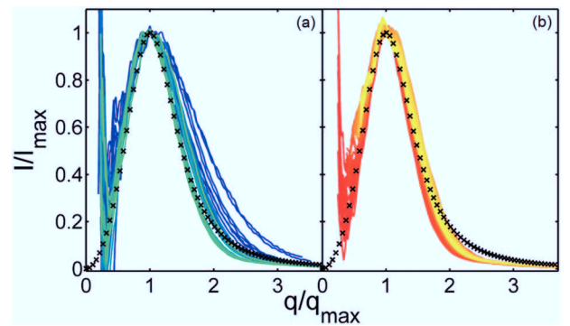
Fig. 3 Dynamic similarity scaling of USAXS data by I_{max} and q_{max} , for the same sample and temperature jump as in Fig. 2. (a) Data from 2.3 to 10.2 s after the temperature jump. (b) Data from 10.6 to 385.5 s after the temperature jump. In both figures lighter colors refer to later times, the function depicted by black crosses is the off-critical Furukawa scaling function (eqn (1)). In agreement with theory, the scaling function describes the data reasonably well for later times.
