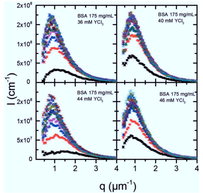
Fig. 5 VSANS profiles of the late stage (10 min to 120 min) coarsening process of dense liquid phases after a temperature jump to T_{\text{jump}} = 35^\circ\text{C} . The caption in each picture specifies the composition of the parent solution from which the dense phases were obtained. The VSANS profiles were collected every 10 min.
