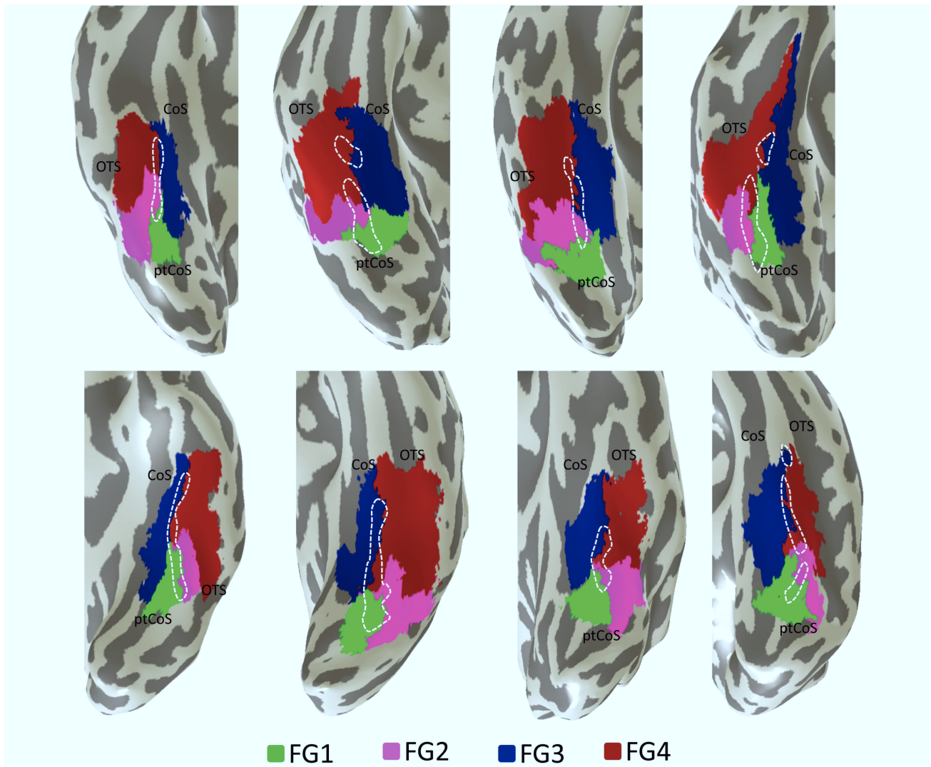
Figure 9. The cytoarchitectonic transition between FG3 and FG4 occurs within the MFS. Cytoarchitectonic regions FG1 (green), FG2 (magenta), FG3 (blue), and FG4 (red) projected to the inflated cortical surface of individual right (top) and left (bottom) hemispheres. The border between FG3 and FG4 occurs within the anterior MFS (dotted line), whereas the border between FG1 and FG2 occurs within the posterior MFS. CoS: collateral sulcus; OTS: occipitotemporal sulcus; ptCoS: posterior transverse CoS. The brains included in this image are from left to right: top: pm 10, pm 9, pm 8, and pm 7; bottom: pm 10, pm 4, pm 3, and pm 1 (cf. Table 1).
