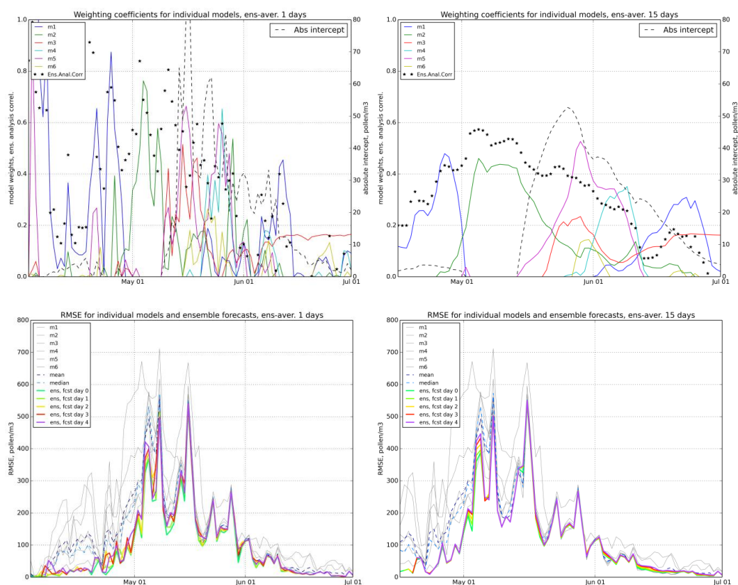
Figure 11. Sensitivity of optimized ensemble to the length of assimilation window. Upper row: optimal weights of the individual models and ensemble score over the 1- (left) and 15- (right) days-long assimilation windows; lower row: RMSE of the of individual models and the optimal ensemble forecasts against those of individual models. Obs. earlier first available date for 1-day-analysis window.
