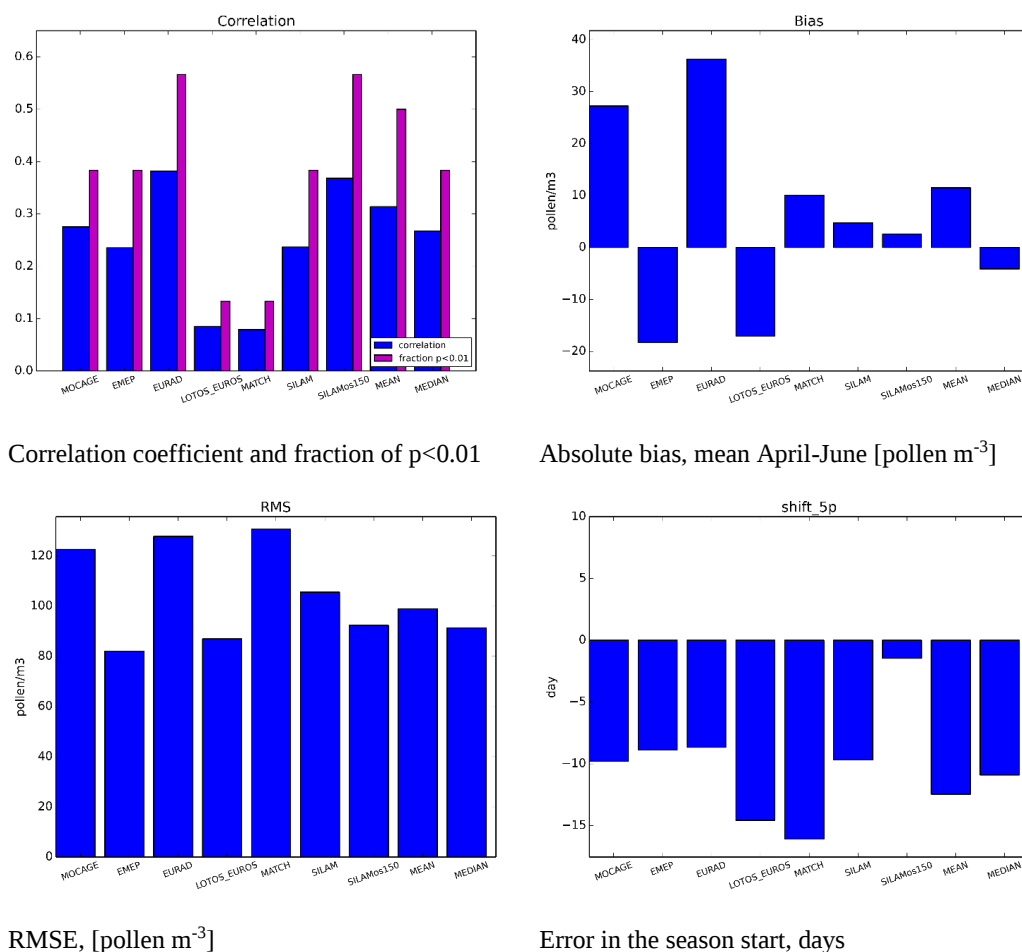
Figure 7. Scores of the individual models, mean over all stations. The same parameters as in Figure 6 . The sensitivity run SILAMos150 is explained in the discussion section
