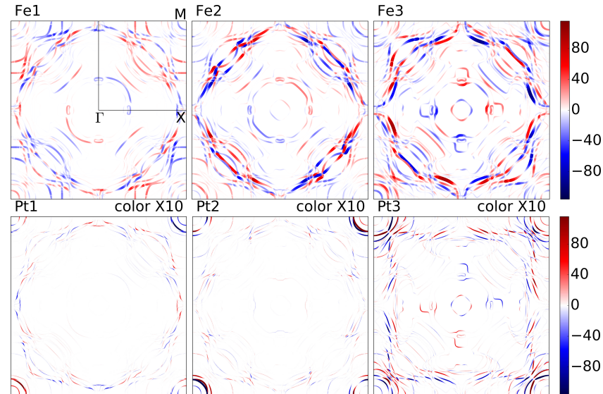
Figure 5.8.: Expectation values \langle \mathcal{T}_{x\mu} \rangle in meV (color code) for \mu = \{\text{Fe1, Pt1, Fe2, Pt2, Fe3, Pt3}\} for the states at the Fermi surface of the FePt/Pt film. Values are multiplied by a factor of ten for Pt atoms to help visualization.
