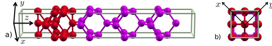
Figure 5.29.: (a) Side and (b) top view of 5 layers of Fe deposited on a Ge(001) film of 12 layers. We show the Fe and Ge atoms in red and violet respectively.
