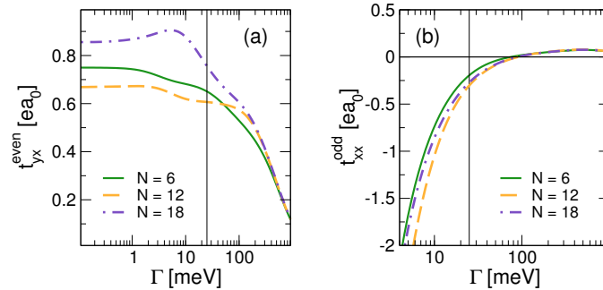
Figure 5.2.: a) Even torkance t_{yx}^{\text{even}} and b) odd torkance t_{xx}^{\text{odd}} in L1_0\text{-FePt}^2/\text{Pt}^N for N = 6 (green solid), 12 (orange dashed) and 18 (blue dot-dashed). Solid vertical lines correspond to the value of disorder strength \Gamma = 25 meV.
