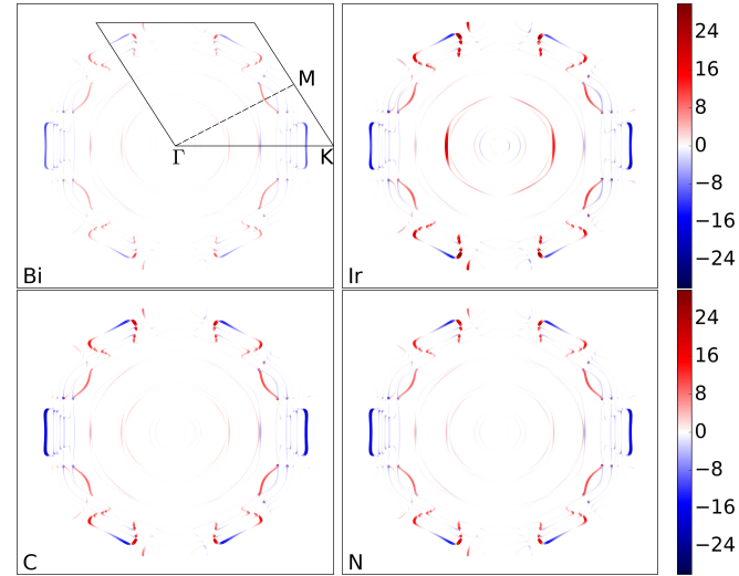
Figure 5.17.: Distribution of \langle -\sigma_{y,Co} \rangle_{\mathbf{k}} \lambda_x(\mathbf{k}) / |\mathbf{v}(\mathbf{k})| in the Brillouin zone, in units of \hbar/R_y , for a Co/Cu film with a concentration of Bi, Ir, C or N impurities per unit cell of \bar{c}_{imp} = 0.1 .
