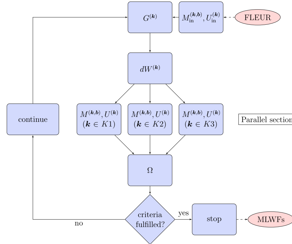
Figure 3.1.: Flowchart of the WANNIER90 program [36] parallelized as part of this thesis. The parallel section includes the calculation of the U^{(k)} and M^{(k,b)} matrices, where the total set of k -vectors is split between n independent sets K_n distributed over n nodes ( n = 3 is shown as an example). Once the parallel section ends, all U^{(k)} and M^{(k,b)} matrices are communicated to each node in order to compute the spread \Omega .
