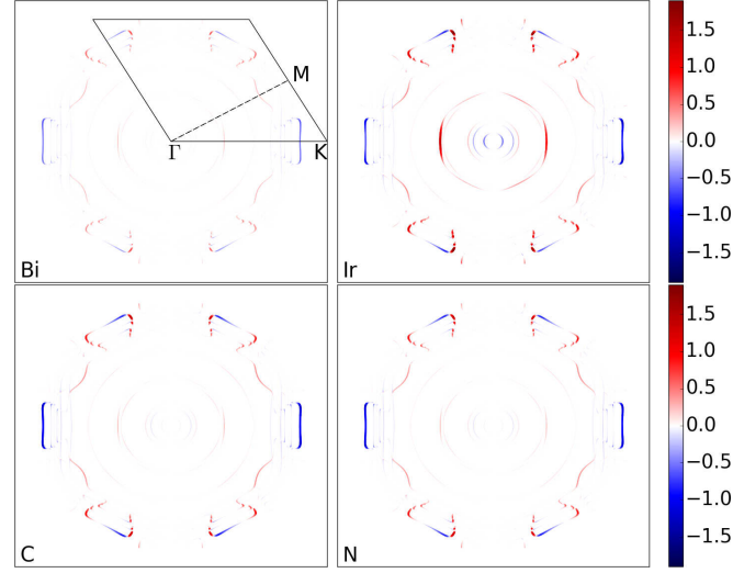
Figure 5.16.: The total torkance in terms of the Fermi surface distribution of \langle \mathcal{T}_x \rangle_{\mathbf{k}} \lambda_x(\mathbf{k}) / |\mathbf{v}(\mathbf{k})| [see Eq. (4.128)], in units of \hbar , for a Co/Cu film with a concentration of Bi, Ir, C or N impurities per unit cell of \bar{c}_{imp} = 0.1 . The irreducible Brillouin zone is shown by solid lines and the dashed line is a guide to the eyes.
