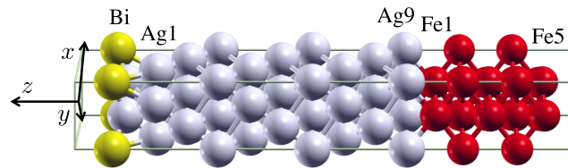
Figure 5.20.: Illustration of the unit cell of a \text{Ag}_2\text{Bi} -terminated \text{Ag}(111) film grown on ferromagnetic \text{Fe}(110) . Bi, Ag and Fe atoms are shown in yellow, gray and red respectively. Atomic coordinates are given in Table 5.5.
