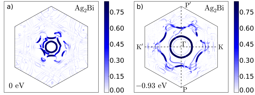
Figure 5.22.: (a) States at the Fermi energy and (b) 930 meV below the Fermi energy marked by the portion of their wave functions located on the Ag 2 Bi layer.
