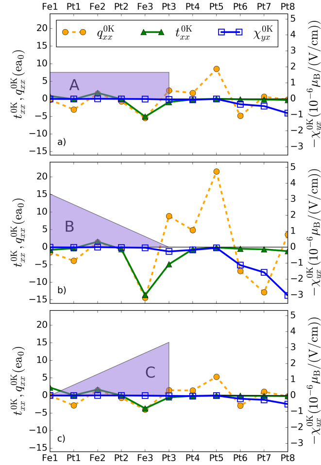
Figure 5.6.: Blue shaded areas give the average number of impurities per unit cell and per atomic layer for distributions A, B and C. The average total number of defects per unit cell is equal to \bar{c}_{imp} = 0.1 for all three distributions. The scale for zero-temperature torques (triangles) and spin-flux response coefficients (circles) is shown on the left. The scale for spin-accumulation response coefficients (squares) is given on the right.
