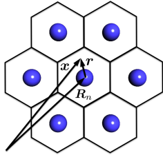
Figure 4.1.: Illustration of the atomic cells (black lines) found by the Voronoi construction and system of coordinates used in the KKR formalism. The vector \mathbf{x} is a globally defined real space vector while the vector \mathbf{r} is defined relatively to the position \mathbf{R}_n of cell n . The atoms of the crystal are shown in blue.
