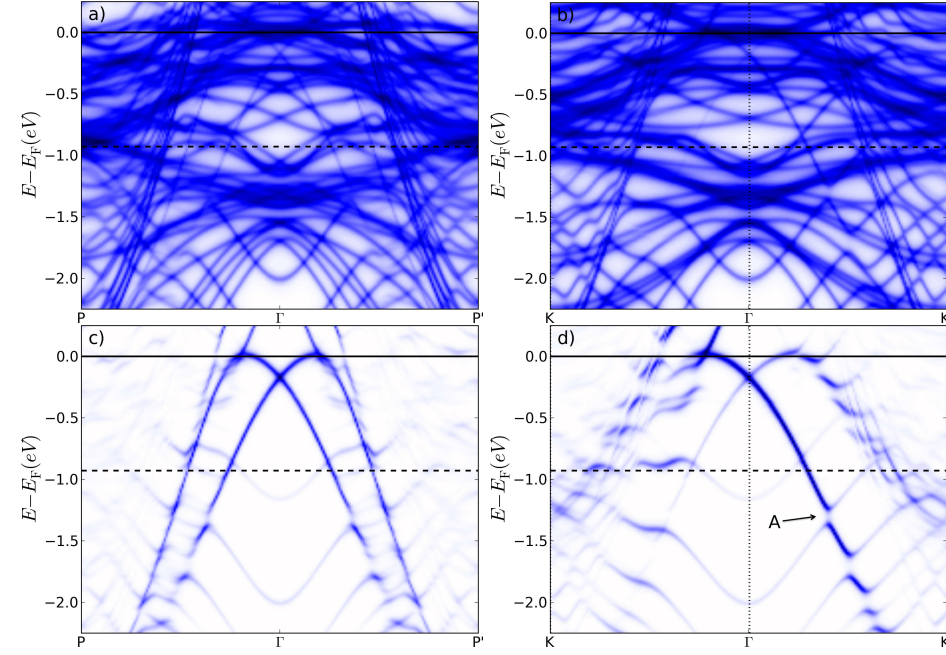
Figure 5.21.: (a,b) Spectral density of states for a Ag 2 Bi-terminated Ag film grown on ferromagnetic Fe(110) along the two different k -paths shown in Fig. 5.22. (c,d) Corresponding local density of states on the Ag 2 Bi layer. An example of asymmetric band-gap opening is marked by the letter A.
