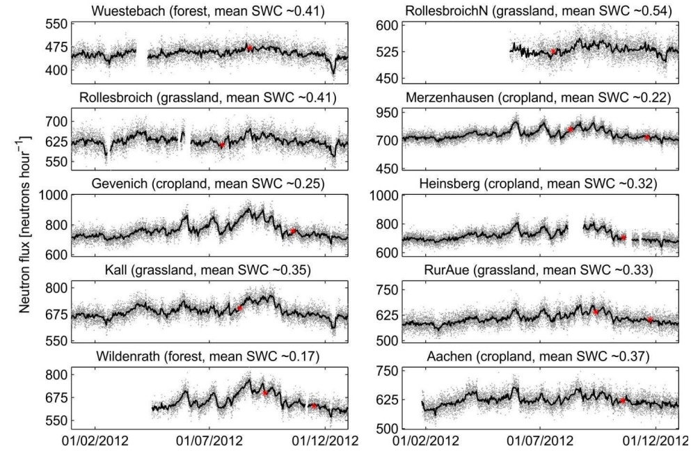
Figure 5: Hourly measured and corrected neutron flux (grey dots), daily average measured corrected neutron flux (black line) and calibration points (red dots) for the ten CRPs installed in the area. Main land use and average soil water content derived with the COSMIC operator during the measurement period in 2012 at the ten locations are also indicated.
