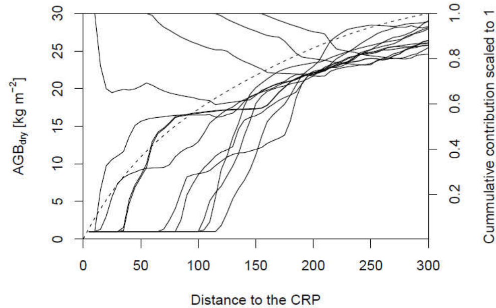
Figure 15: Aboveground biomass estimates for radial segments of the temporary CRPs at Wuestebach using the horizontal weighting scheme of Bogaen et al. (2013) with 5 meter steps. The dashed line shows the cumulative contribution of the segments to a total of 1.
