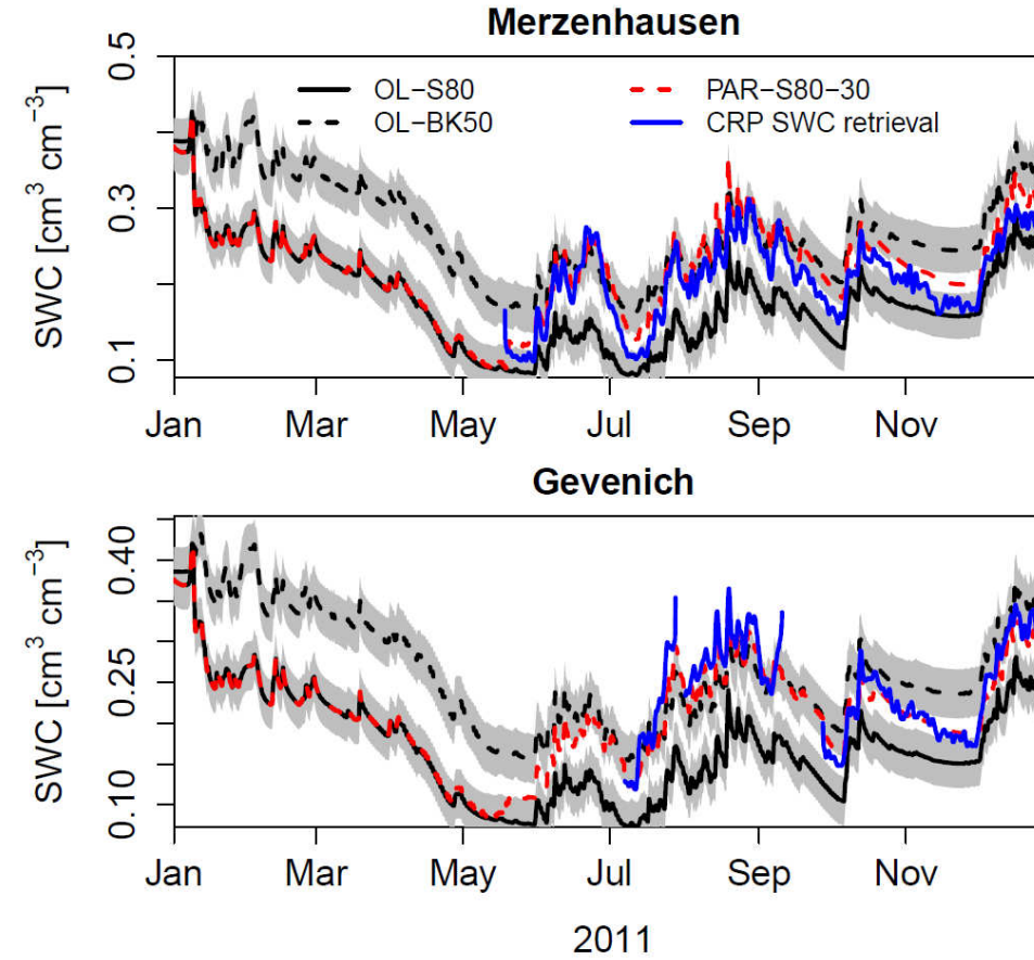
Figure 22: Temporal evolution of simulated SWC, calculated with open loop (OL-*) simulations and data assimilation including parameter updating (PAR-S80-30), together with the CRP soil water content retrieval (SWC) during the first year of simulation at the sites Merzenhausen and Gevenich. Simulated SWC was vertically weighted using the COSMIC operator to obtain the appropriate SWC corresponding to the CRP SWC retrieval.
