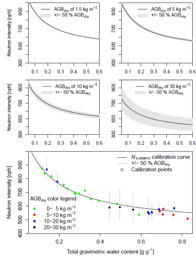
Figure 21: Uncertainty in neutron flux assuming an uncertainty of \pm 50\% AGB_{dry} and N_{0,AGB=0} = 1210 cph. The upper two panels, show resulting measured fast neutron flux N_{epih} for different biomass values, the lower panel shows the uncertainty of vegetation corrected neutron flux at the times of calibration based on biomass uncertainty.
