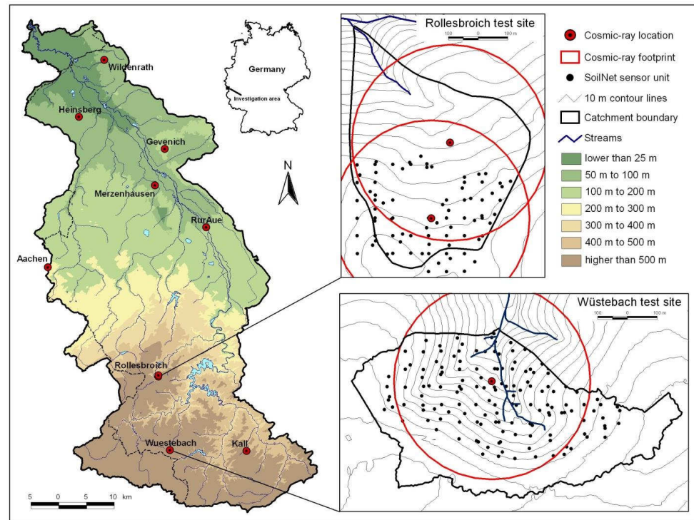
Figure 3: Locations of the ten CRPs installed in the Rur catchment (left), setup of the Rollesbroich test site (upper right) and the Wuestebach test site (lower right panel) with the SoilNet sensor units.
