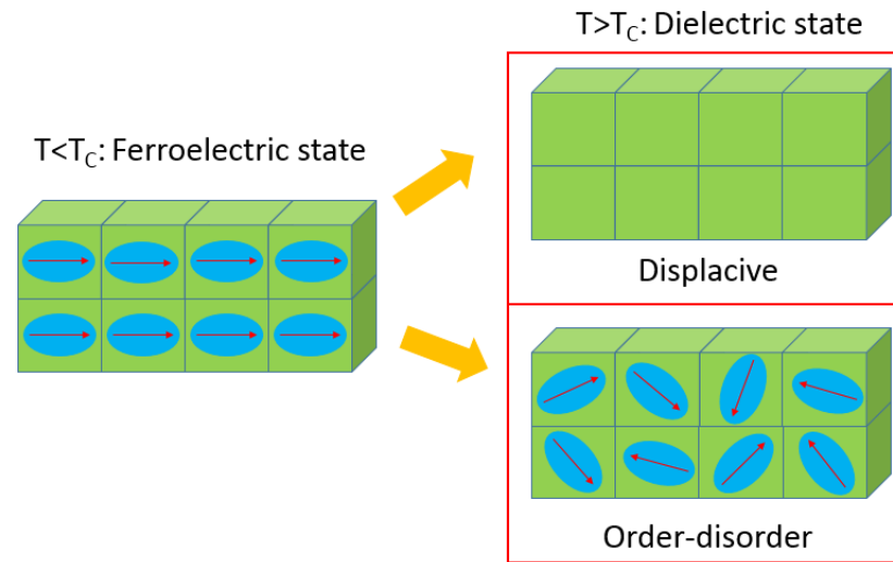
Fig. 2.9: Schematic illustrations of displacive and order-disorder ferroelectric phase transitions.
