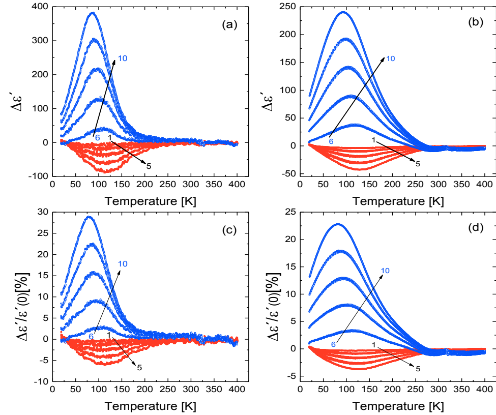
Fig. 5.4: Temperature dependence of the electric field induced modification of the permittivity with respect to the data shown in Fig. 4.3 and resulting tunability for the 27 nm (a, c) and 63 nm (b, d) thick NaNbO 3 films, where \Delta\varepsilon' is defined as \Delta\varepsilon' = \varepsilon'(E_{ac}, E_{dc}) - \varepsilon'(0) and \varepsilon'(0) = \varepsilon'(E_{ac} = 0.048\text{V}/\mu\text{m}, E_{dc} = 0) and tunability is defined as \Delta\varepsilon'/\varepsilon'(0) . For curves 1 – 5 (red solid symbols) the dc-bias is varied from E_{dc} = 0.2\text{ V}/\mu\text{m} to 1\text{ V}/\mu\text{m} in steps of 0.2\text{ V}/\mu\text{m} , the ac-field is kept at the minimum value of E_{ac} = 0.048\text{ V}/\mu\text{m} , while for curves 6 – 10 (blue open symbols) the ac-field amplitude is increased in steps of 0.2\text{ V}/\mu\text{m} from E_{ac} = 0.2\text{ V}/\mu\text{m} to 1\text{ V}/\mu\text{m} with E_{dc} = 0 . The frequency is 1 MHz for all measurements, the arrows indicate the direction of increasing electric field.
