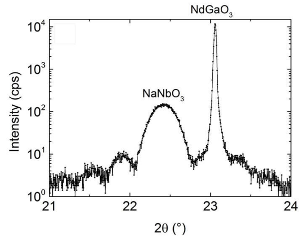
Fig. 6.3: Magnified HRXRD scans around the (110)_o reflection peaks of the \text{NdGaO}_3 substrate for the nominal \text{Na}_{1.17}\text{NbO}_{3.6} film. Contribution of the \text{NaNbO}_3 is clearly visible as well as the substrate \text{NdGaO}_3 .
