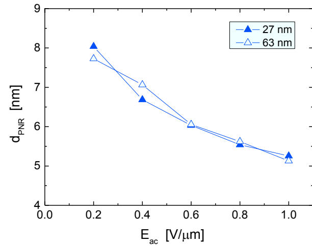
Fig. 5.8: Diameter of PNRs that are mobile (i.e. attributing to the permittivity) at the freezing temperature as function of applied ac electric field for 27 nm (solid) and 63 nm (open) thick \text{NaNbO}_3 films, respectively. The diameter of PNRs are calculated by assuming an idealized spherical shape for the PNRs.
