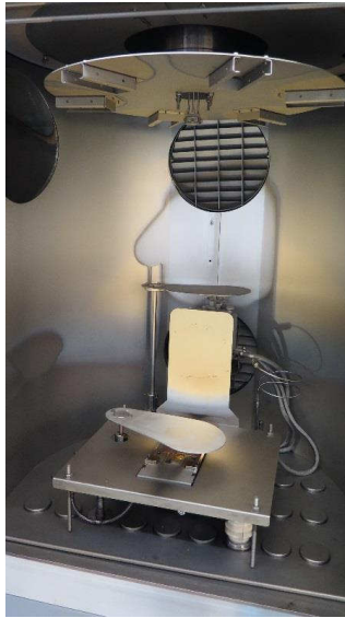
Fig. 3.3: Picture of the evaporation setup of the Helmholtz Nanoelectronic Facility (HNF) of Jülich Research Center.
