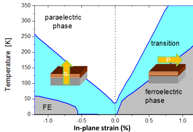
Fig. 2.19: Prediction of the shift of T_C in SrTiO 3 as function of the in-plane strain based on Pertsev et al.. The cyan region represents the range (error bar) of the phase transition. The arrows indicate the direction of enhanced polarization. Adapted from [18]
