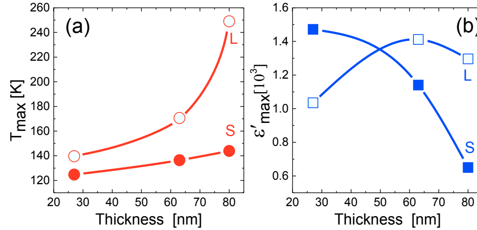
Fig. 4.7 (a) T_{\text{max}} (red circles) and (b) corresponding maximum dielectric constant \epsilon'_{\text{max}} (blue squares) of \text{NaNbO}_3 thin films for E oriented along the small (S, solid symbols) and large (L, open symbols) axis directions as function of film thickness.
