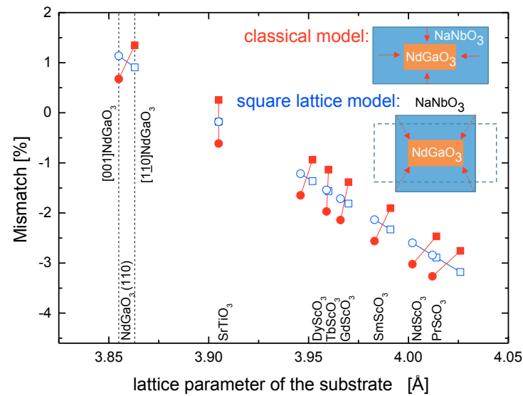
Fig. 4.8: Mismatches between the \text{NaNbO}_3 film and various substrates based on the classical approach (solid symbols) and “square lattice” model (open symbol) for the large direction (square) and small direction (circle). Sketches of the two models are given as insets.
