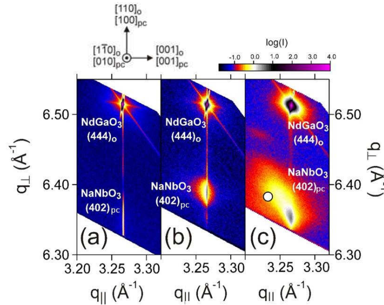
Fig. 3.6: High resolution x-ray diffraction RSM in the vicinity of the (444)_o Bragg reflection of the \text{NdGaO}_3 substrate for a 11 nm (a), 80 nm (b) and 140 nm (c) thick sample. The circle in (c) marks the position of the corresponding (402)_{pc} reflex of unstrained \text{NaNbO}_3 . The sketch shows the resulting structural correlation of film and substrate according to the “classical model” which will be discussed in detail in Chapter 4.3.
