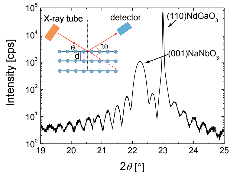
Fig. 3.4: HRXRD \theta/2\theta scan (Bragg-Brentano scan) of a \text{NaNbO}_3 on a (110)\text{NdGaO}_3 substrate. The major two peaks are explicitly analyzed and ascribed to (001)\text{NaNbO}_3 and (110)\text{NdGaO}_3 , respectively. The rest of the peaks with less intensity are thickness fringes which help to estimate the thickness of the film. The inset shows the sketch of the Bragg-Brentano geometry. Adapted from [100].
