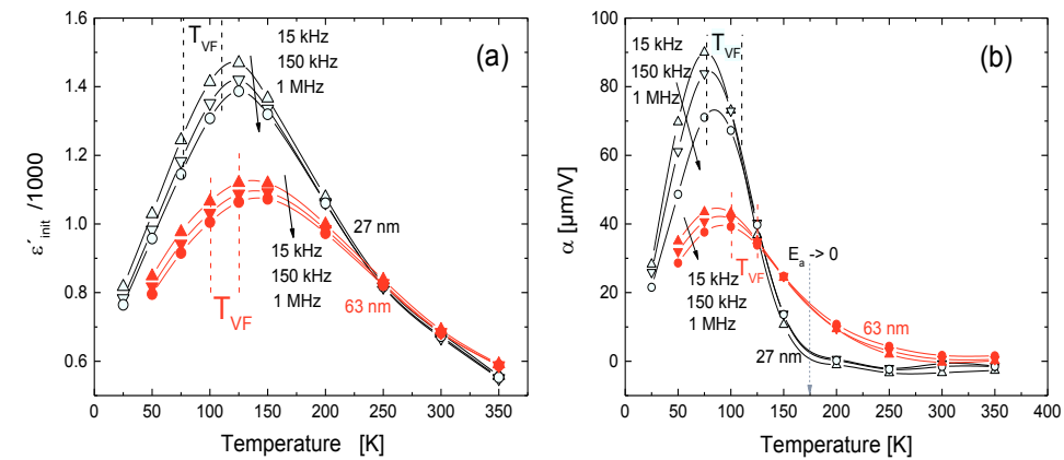
Fig. 5.10: Initial permittivity (a) and Rayleigh parameter (b) as function of temperature for the NaNbO 3 thin films with different thickness, 27 nm (open symbols) and 63 nm (solid symbols), measured at frequencies 15 kHz (triangle), 150 kHz (inverted triangle), and 1 MHz (circle). The dashed lines mark the regime of freezing temperature for E_{\text{ac}} = 1 \text{ V}/\mu\text{m} (lower temperature) and E_{\text{ac}} = 0.048 \text{ V}/\mu\text{m} (higher temperature). The solid arrows indicate the direction of increasing frequency, the dashed arrow in (b) marks the temperature at which the activation energy extrapolates to zero (see Fig. 5.6(b)).
