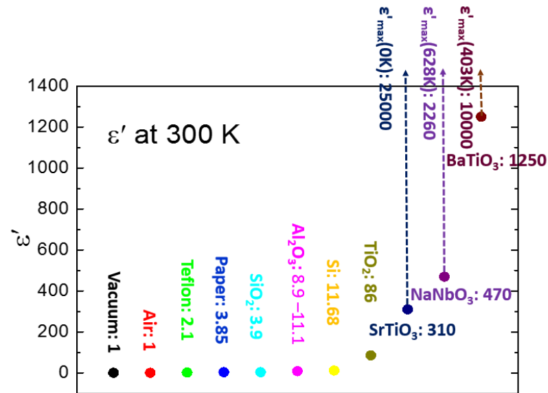
Fig. 1.2: Permittivity of various materials at room temperature, however the maximum permittivity for a number of ferroelectric oxides, e.g. \text{SrTiO}_3 , \text{NaNbO}_3 and \text{BaTiO}_3 , is obtained at temperatures close to the phase transitions far from room temperature.
