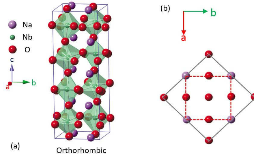
Fig. 2.5 Sketches of (a) the orthorhombic structure of bulk \text{NaNbO}_3 at room temperature (Adapted from [44]), and (b) a comparison of the orthorhombic (solid line) and pseudocubic unit cell (dash line) for the a-b plane of \text{NaNbO}_3 .
