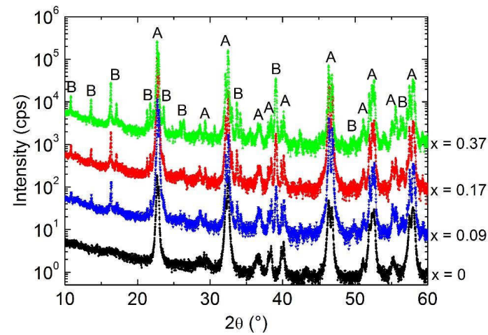
Fig. 6.1: Powder XRD measurements of \text{Na}_{1+x}\text{NbO}_{3+\delta} targets prepared with Na excess compared to the stoichiometric \text{NaNbO}_3 ( x = 0 ) composition. For better visibility the signals are shifted by a factor of 10 for each successive composition, the compositions x are given in the figure. Reflection peaks indicated by “A” and “B” are attributed to the \text{NaNbO}_3 perovskite and \text{Na}_3\text{NbO}_4 as the secondary phase, respectively. Adapted from [100].
