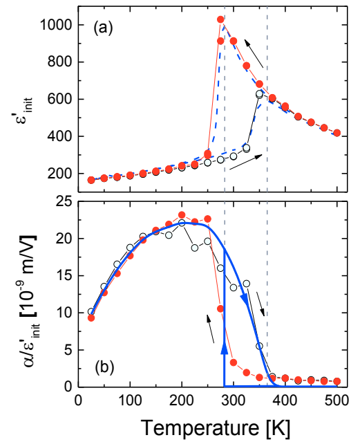
Fig. 6.8: Temperature dependence of the initial permittivity \epsilon'_{\text{init}} (a) and the normalized Rayleigh parameters \alpha/\epsilon'_{\text{init}} (b) for cooling (solid symbols) and heating (open symbols) for the (\text{NaNbO}_3)_{0.915}(\text{Na}_3\text{NbO}_4)_{0.085} film. For comparison, the permittivity measured at E_{\text{ac}} = 0.2 \text{ V}/\mu\text{m} is added by the blue dashed line in (a). The blue solid line in (b) serves as a guide for the eye for the idealized hysteretic temperature dependence. The two vertical lines mark the position of the transition from dielectric to ferroelectric behavior for cooling and heating, respectively.
