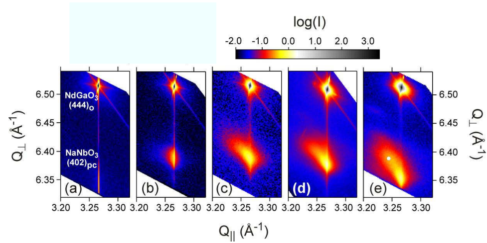
Fig. 4.1: High resolution x-ray diffraction RSM in the vicinity of the (444)_{\text{o}} Bragg reflection of the NdGaO 3 substrate for a 11 nm (a), 27 nm (b), 63 nm (c), 80 nm (d), and 140 nm (e) thick sample. The circle in (e) marks the position of the corresponding (402)_{\text{pc}} reflection of unstrained NaNbO 3 .
