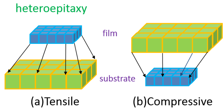
Fig. 2.18: Schematic sketch of heteroepitaxy leading to tensile (a) and compressive (b) in-plane strain, which is partially compensated by an out-of-plane strain of opposite sign.
