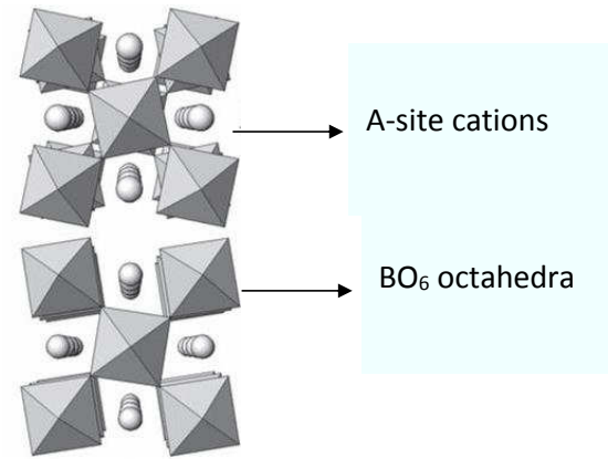
Fig. 2.17: Schematic illustration of the rotation of \text{BO}_6 octahedra, the balls represent A-site cations. The B-site cations are placed at the center of the octahedral. Adapted from [93].
