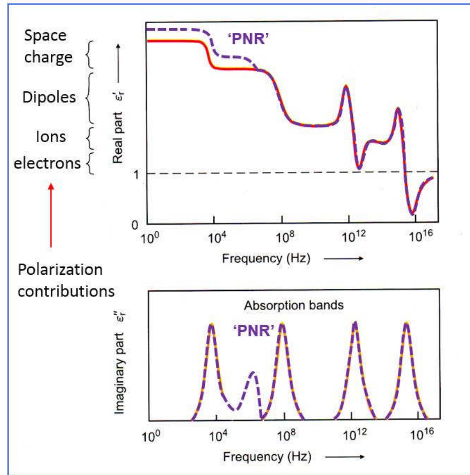
Fig. 2.2: Frequency dependence of the real part \epsilon' , and imaginary part \epsilon'' , of the dielectric constant for different polarization mechanisms without (solid) and with (dash) the contribution from polar nano-regions (PNRs). Adapted from [18].
