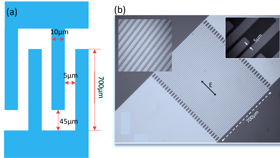
Fig. 3.10: Schematic illustration (a) of the IDEs with dimensions used in this thesis and scanning electron microscopy pictures (b) of the IDEs. The inset shows part of the IDE with larger amplification.
