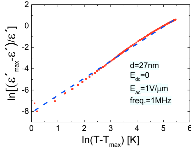
Fig. 5.3: Double logarithmic plot of the reduced and normalized permittivity versus reduced temperature at the phase transition ( T > T_{\max} ) measured at 1 MHz, E_{\text{dc}} = 0 , E_{\text{ac}} = 1 \text{ V}/\mu\text{m} for the \text{NaNbO}_3 film with a thickness of 27 nm (red). The blue dash line represents the theoretic Lorentz fit based on Eq. (5.4).
