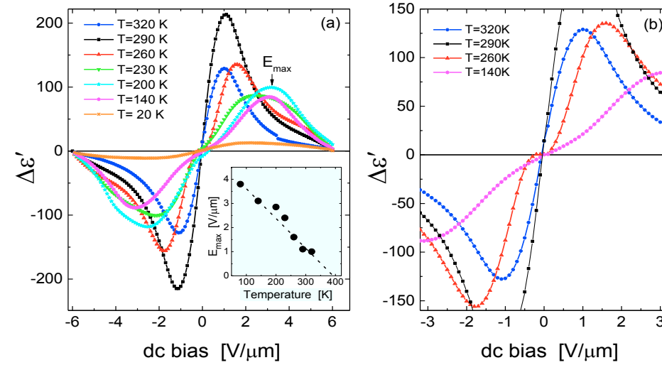
Fig. 4.10: Hysteretic behavior of the permittivity \Delta\epsilon' = \epsilon' (increasing bias) - \epsilon' (decreasing bias) of the 80 nm thick \text{NaNbO}_3 film on (110) \text{NdGaO}_3 (long axis) measured at 1 MHz for different temperatures. The inset in (a) represents the temperature dependence of the position of the maxima E_{\max} as indicated by an arrow for one temperature, (b) represents an enlarged plot of the bias dependence of \Delta\epsilon' around zero bias for selected temperatures.
