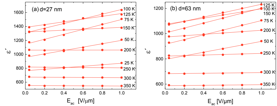
Fig. 5.9: Permittivity as function of the ac electric field measured at 1 MHz and different temperatures for E oriented along the short axis for the 27 nm (a) and 63 nm (b) thick NaNbO 3 films, respectively. The lines represent linear fits of the data according to Eq. (5.6).
