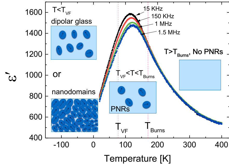
Fig. 2.16: Schematic illustrations of the evolution of PNRs in a strained \text{NaNbO}_3 film on (110)\text{NdGaO}_3 correlated to dipolar glass and random field models.
