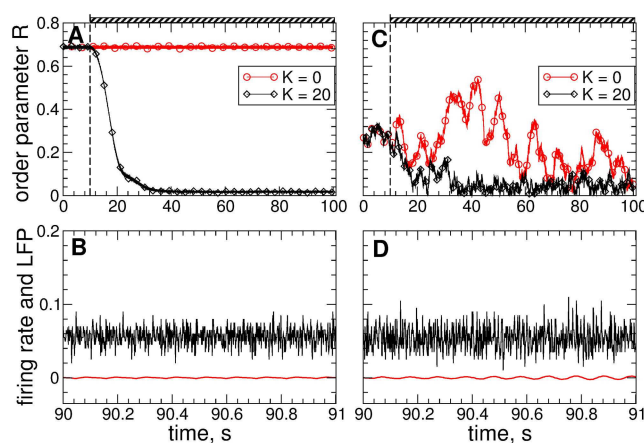
Fig 3. Suppression of synchronization in the neuronal ensemble Eqs (1)–(3) by the LDF stimulation Eq (6). Time courses of the order parameter R of STN neurons for the stimulation intensity K = 0 (stimulation-free case) and K = 20 are shown in plots (A) and (C) for strongly coupled ( g_{G-S} = 1.7 \text{ nS}/\mu\text{m}^2 ) and weakly coupled ( g_{G-S} = 1.28 \text{ nS}/\mu\text{m}^2 ) regimes, respectively. The stimulation epochs are indicated by hatched bars on the top of the plots. In plots (B) and (D) the corresponding firing rates (black curves) and filtered LFPs (red curves) of the stimulated STN neurons are depicted for the strongly and weakly coupled cases, respectively. Parameter \tau = 95 ms.
