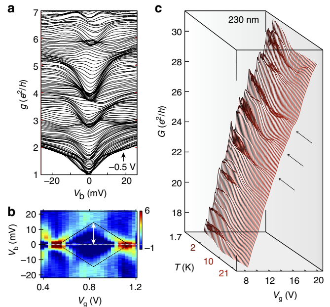
Figure 4 | Finite bias and temperature dependence of the quantized conductance. (a) Zero B-field differential conductance g as a function of bias voltage V_b , measured at T = 6 K, taken at fixed values of back-gate voltage V_g from -0.5 to 3.0 V in steps of 30 mV (see lower right label). The dense regions correspond to plateaus in conductance. (b) Transconductance \partial g / \partial V_g in units of e^2/hV (see colour scale) as a function of bias and back-gate voltage for a different cool-down of the same device (Supplementary Note 6). At V_b = 0 , the transitions between conductance plateaus appear as red spots, which provides an energy scale for the sub-band energy spacing \Delta E \approx 13.5 \pm 2 meV (see dashed black lines and white arrow), which is also in good agreement with the energy scale observed in (a) (Supplementary Note 6). (c) Conductance traces as a function of temperature and back-gate voltage. We observe features with different temperature dependencies. Above around 10 K only kinks related to quantized conductance survive (see arrows).
