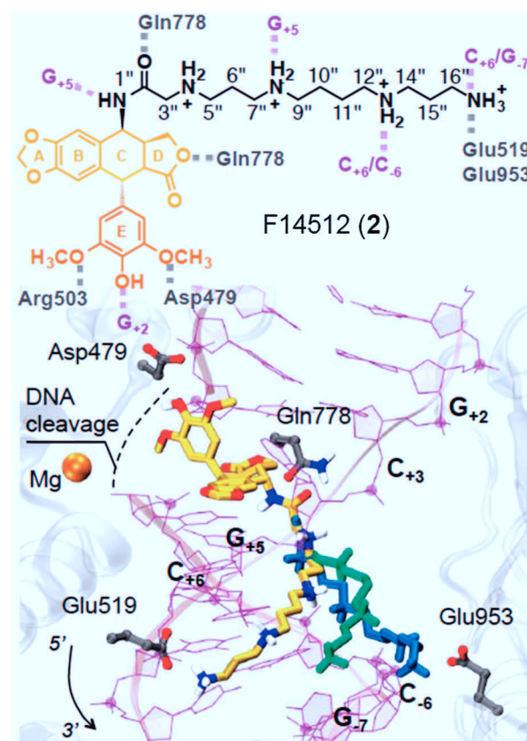
Fig. 3 Key interactions between F14512 and the topoll/DNA cleavage complex shown schematically (top). The statistical distribution over the production runs of the H-bond interactions is reported in Fig. S3 (ESI†). Three representative binding modes of F14512 from MD simulations are shown with different colours of the spermine moiety (bottom).
