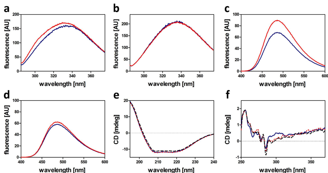
Figure 3. Fluorescence of aromatic amino acids of CitAP-BsLA (a) and wild-type BsLA (b). Protein samples, diluted to 3 \mu M in 10 mM glycine buffer pH 10 supplemented with 10 mM NaCl, were excited at 278 nm. (c) Fluorescence emission spectra of 4,4'-dianilino-1,1'-binaphthyl-5,5'-disulfonic acid (bis-ANS) of samples containing CitAP-BsLA or wild-type BsLA (d). 6 \mu M of bis-ANS was added to protein samples (3 \mu M) in 10 mM glycine buffer pH 10 supplemented with 10 mM NaCl. Bis-ANS was excited at 385 nm. All fluorescence emission spectra were recorded in the presence (red line) and absence (blue line) of 1 mM sodium citrate. Far-UV (e) and near-UV (f) circular dichroism (CD) spectra of CitAP-BsLA in 10 mM glycine buffer pH 10 supplemented with 10 mM NaCl (blue solid line), after addition of 1 mM sodium citrate (red dashed line) and in the presence of 1 mM sodium citrate and 50 \mu M Triton X-100 (black dashed line). All spectra were recorded at 25 ^{\circ} C.
