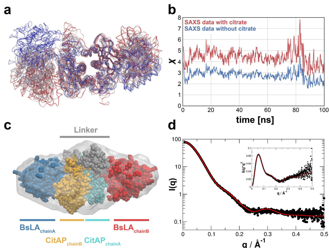
Figure 5. (a) Structural changes during the molecular dynamics (MD) simulations of the dimeric M_{low-free} CitAP-BsLA model. The proteins are shown as ribbons and the colors represent structures at different times, changing from red at t = 0 ns to blue at t = 100 ns. (b) Time evolution of \chi during the MD simulations of the M_{low-free} model. Deviation between the model and experimental data measured at 5 mg/ml (blue) and without citrate (red) are shown. (c) Final model of the CitAP-BsLA dimer complex superimposed onto the SAXS derived low-resolution envelope obtained from SAXS data at high protein concentration in the presence of citrate. (d) SAXS scattering curve recorded for CitAP-BsLA at a protein concentration of 5 mg/ml in the presence of citrate (black dots) and the CRY SOL-fitted theoretical scattering curve of the final CitAP-BsLA dimer model (red line).
