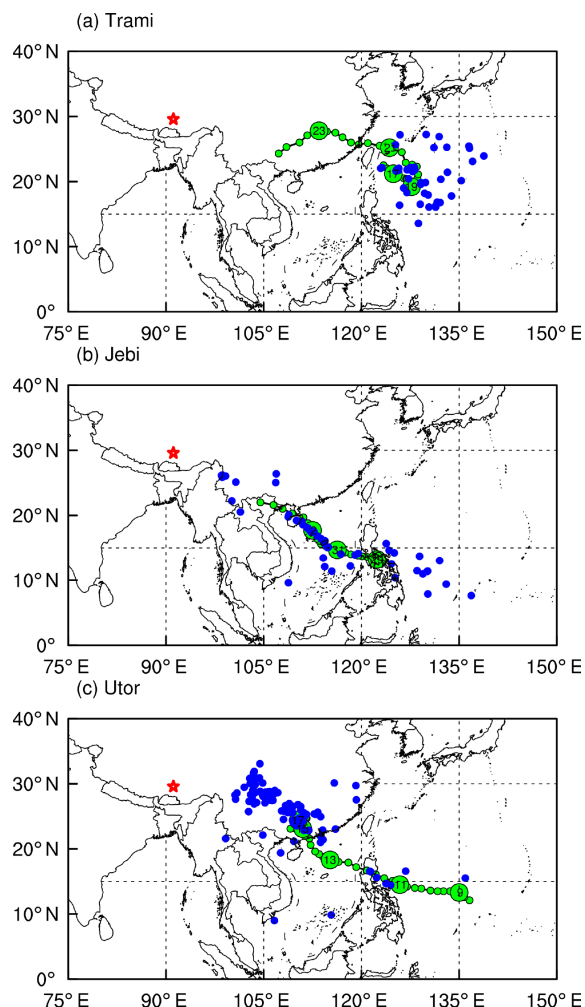
Figure 2. Pathways of tropical cyclones (a) Trami, (b) Jebi, and (c) Utor are marked as green dots for every 6 h. The number printed inside the large green dots indicates the day in August 2013, except 29 and 31 in (b), which refer to 29 and 31 July. The blue points denote the average geographical position where air parcels experienced strong uplift within tropical cyclones. The red star marks the location of Lhasa.
