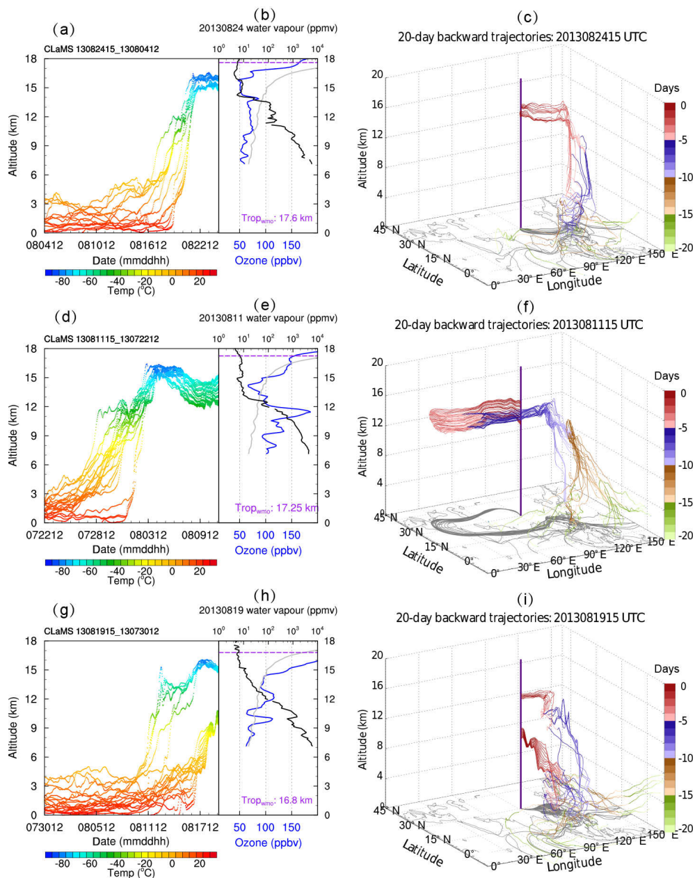
Figure 3. The 20-day backward trajectories started along measured balloon profiles of target parcels on 24 (a, c), 11 (d, f), and 19 (g, i) August 2013. Backward trajectories influenced by tropical cyclones Trami, Jebi, and Utor are shown colour-coded by temperature (left). The vertical profiles of ozone (blue line), water vapour (black line), and the mean of ozone profiles in August 2013 (grey line) are also shown (middle). The geographical position (latitude, longitude, and altitude) of the 20-day backward trajectories is given (right) colour-coded by days observed from measurement. The vertical line marks the location of the Lhasa site. The grey lines in the maps show the longitude–latitude projection of the trajectories.
