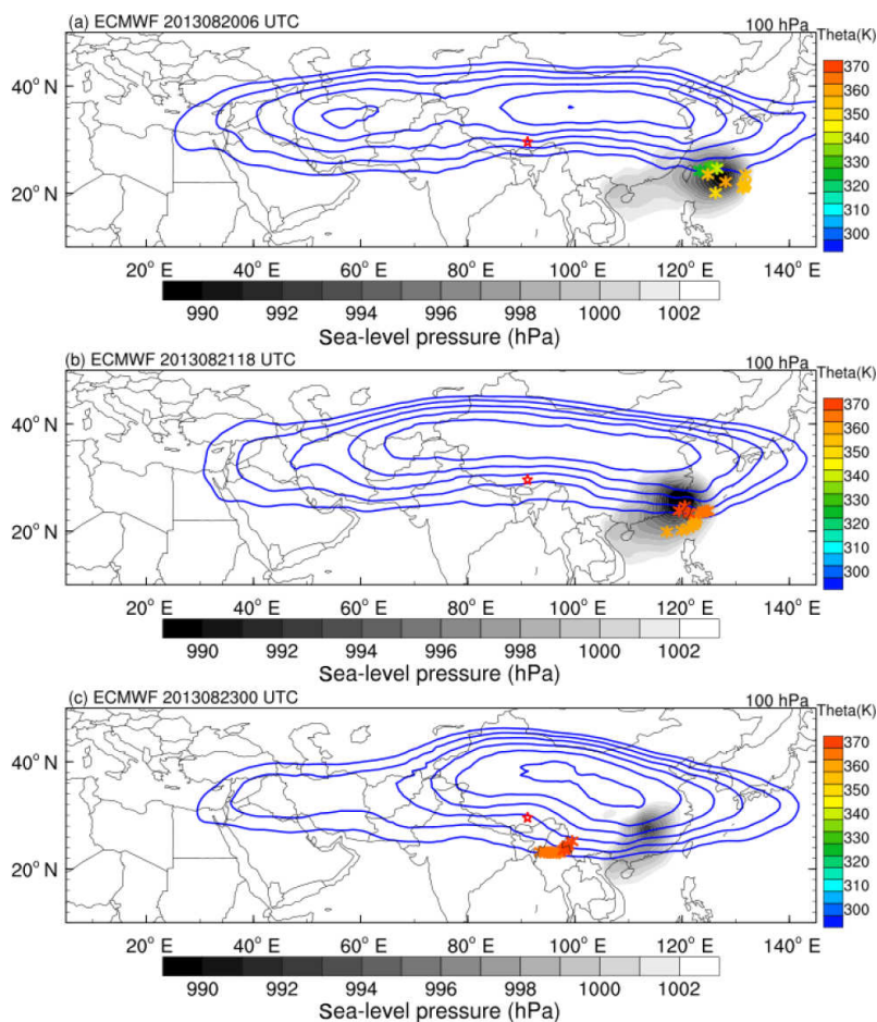
Figure 5. The geopotential height at 100 hPa pressure level (blue contour lines, > 16.72 km) and sea-level air pressure (shade, hPa) of Trami at (a) 06:00 UTC 20 August, (b) 18:00 UTC 21 August, and (c) 00:00 UTC 23 August. The asterisks, colour-coded by potential temperature, mark the geographical positions of target parcels. The red star marks the location of Lhasa.
