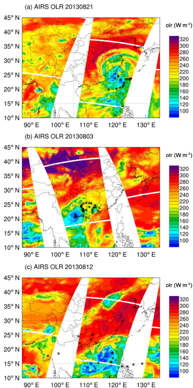
Figure 8. Outgoing long-wave radiation from AIRS satellite on 21, 3, and 12 August. The asterisks mark the locations of target air parcels at the time of the AIRS measurements.
