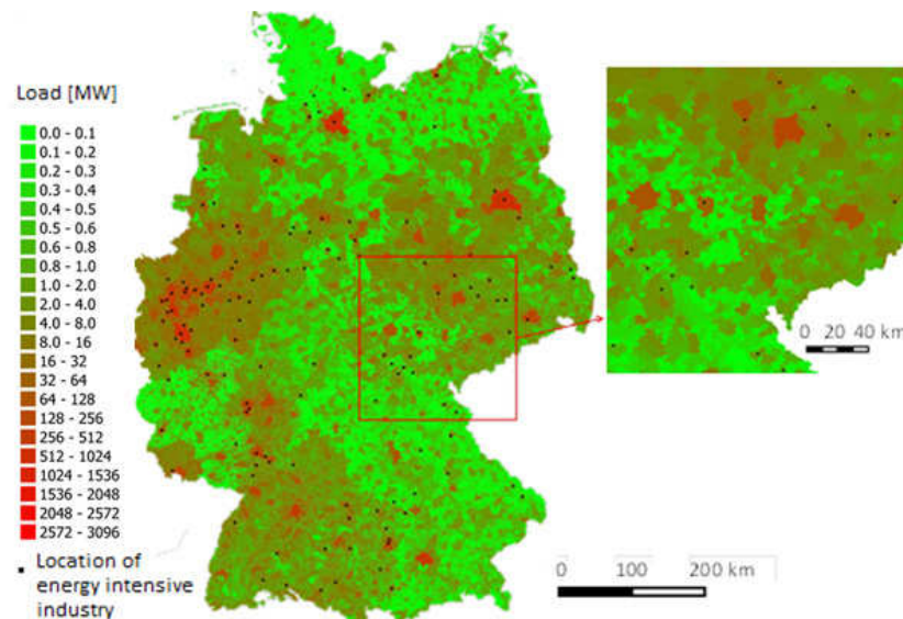
Figure 6. Electrical load on 5 December 2013 at 18:00 with adjusted load factors and displaying the location of energy-intensive industries [58].
