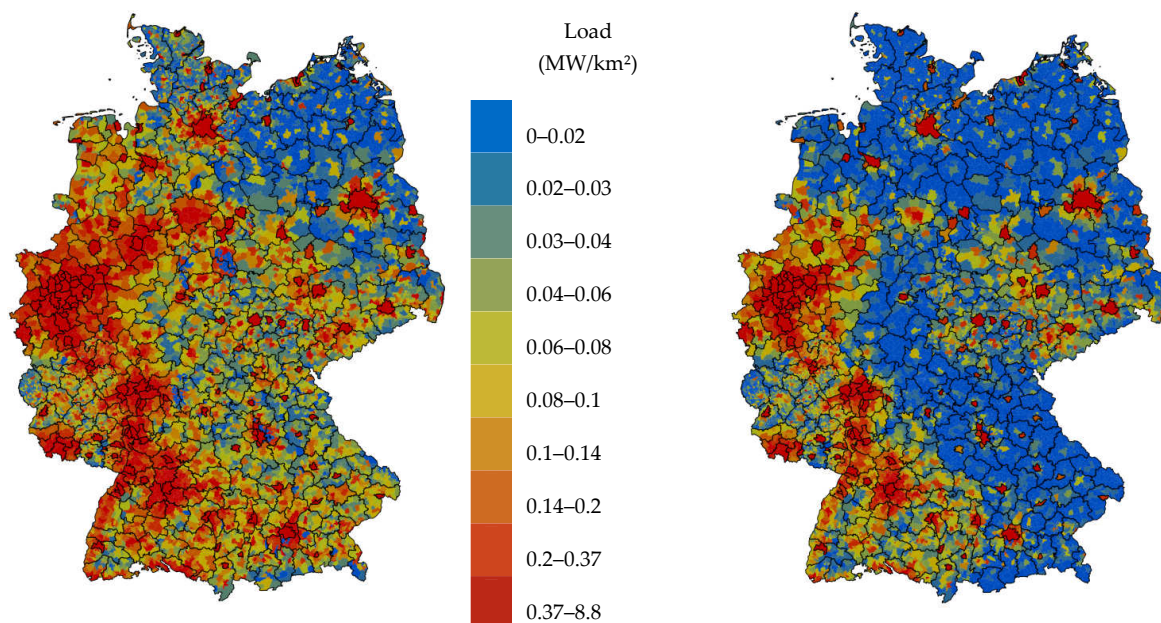
Figure 7. Electrical load with the adjusted load factors and the additional steady load; (left) highest load (5 December 2013, 18:00); (right) lowest load (2 June 2013, 07:00) [59].
