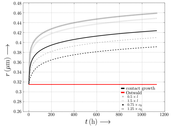
FIG. 17. Experiment performed by Faes. The black curve is calculated by taking into account only the agglomeration process developed in Sec. II. The red curve describes the agglomeration due to the Ostwald ripening. The gray dotted lines represent a variation of the free parameter l by \pm 50\% , whereas the black dotted lines are calculated with a relative change of the free parameter c_0 by 25%.
