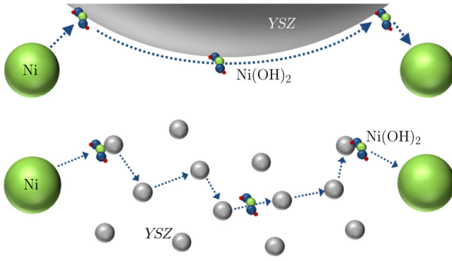
FIG. 8. The scheme shows the influence of the YSZ particle size on the agglomeration mechanism by the Ostwald ripening. The \text{Ni(OH)}_2 molecules can move more freely on the surface; thus, they can cover larger distances if the YSZ particles are larger. This process connects more distant particles and enables a more effective exchange between two Ni spheres.
