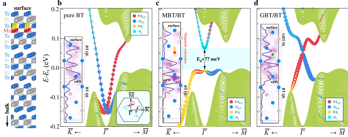
Figure 1: (a) Atomic structure of MBT/BT with gold arrows indicating the Mn 3d moments, pointing out of the surface plane. (b,c,d) Spin-resolved surface band spectra of BT (b), MBT/BT (c) and \text{GeBi}_2\text{Te}_4/\text{BT} (GBT/BT (d)). The size of color circles reflects the value and sign of the spin vector Cartesian projections, with red/blue colors corresponding to the positive/negative in-plane components (that directed perpendicular to the \mathbf{k} vector), and gold/cyan reflecting the out-of-plane components +s_z/-s_z . Green areas correspond to the bulk band structure projected onto the surface Brillouin zone. The insets to (b), (c) and (d) show the real space distribution of the topological surface state charge density as projected onto the ac -plane (color map in the white-to-pink palette) and as integrated over the ab plane (purple line) for BT, MBT/BT and GBT/BT, respectively. In the insets, the 'vdW' stays for the van der Waals gap.
