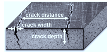
Figure 5.20: Schematic view of the crack parameters on a typical beryllium specimen.
