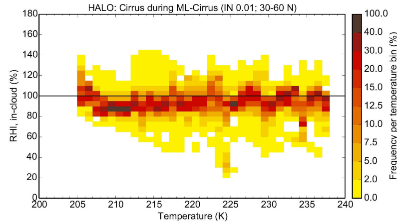
Figure 4.1: Probability of occurrence of RH measurements within clouds as a function of temperature. The expected distribution would have a peak at \text{RH} = 100\% . Graphic: courtesy of Christian Rolf.
