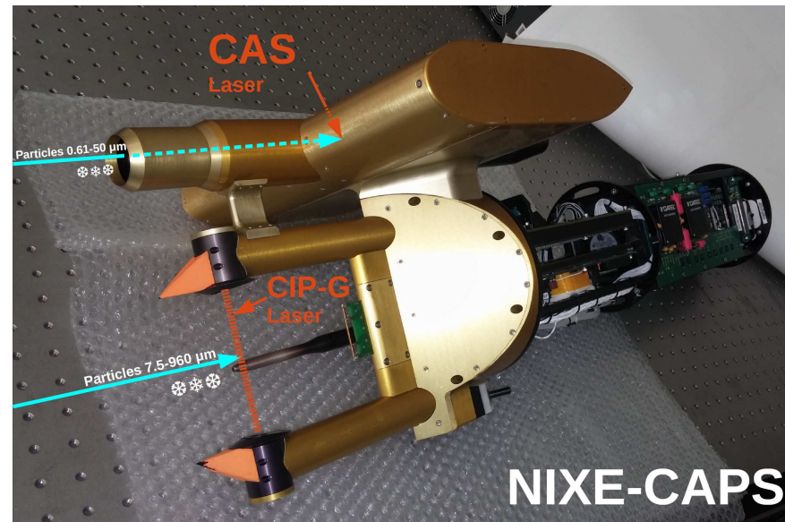
Figure 2.1: NIXE-CAPS dismounted. The upper flat box contains the CAS instrument; its laser beam is hidden in the housing. The CIP laser beam is located between the two arms capped with oranges spikes, which lead shattered particle fragments away from the measurement area. The blue arrows indicate the air flow direction in flight.
