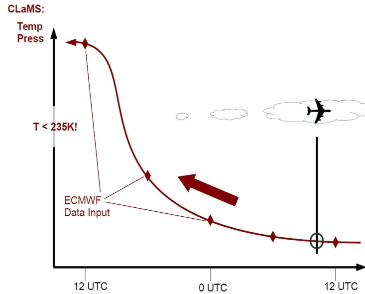
Figure 4.2: 24 backward trajectories are calculated by CLaMS that show the air parcel origin and the temperature/pressure history before the air reached the flightpath. Temperature, pressure, relative humidity and ice water content based on the ECMWF data fields are assigned to the trajectory.
