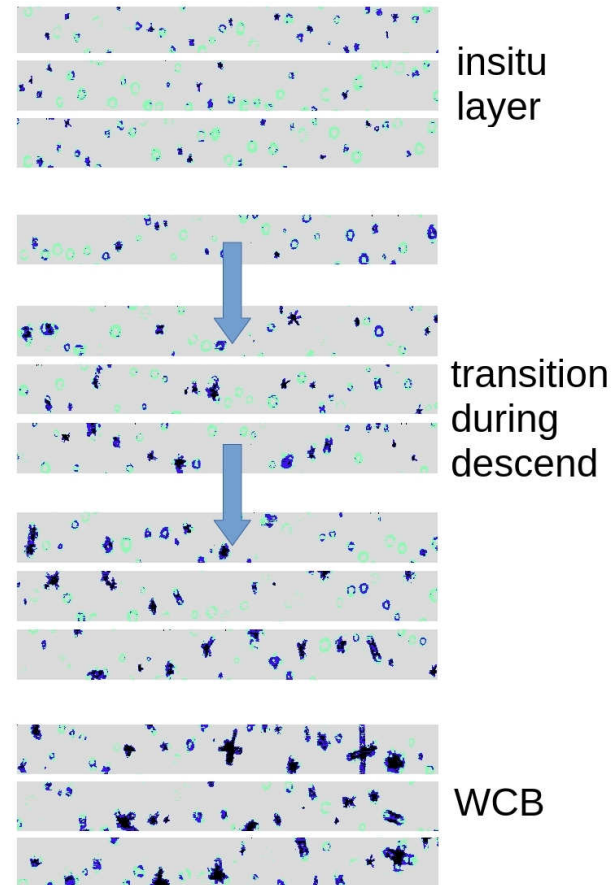
Figure 4.15: Top: CIP images recorded within the cirrus cloud layer at the higher altitude above the liquid origin clouds (compare Figure 4.17). Middle panels: As the aircraft descends into the liquid origin cloud region, a shift in the particle habits towards larger diameters and more complex shapes can be observed. Bottom: Within the liquid origin clouds, large rosettas and aggregates are recorded by the CIP.
