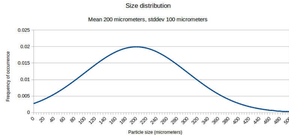
Figure A.6: Simulated size distribution for a typical cirrus cloud.
