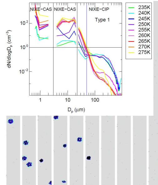
Figure 3.6: Type 1 clouds: Example of CIP images and average particle size distributions (PSDs) in 5 K intervals, all campaigns. The thin vertical line at 3\mu\text{m} marks the boundary between aerosol and cloud particles. The line at 20\mu\text{m} marks the transition from the NIXE-CAS-DPOL to the NIXE-CIPg instrument. The thick blue line divides the cloud particle population in particles smaller and larger than 50\mu\text{m} .
