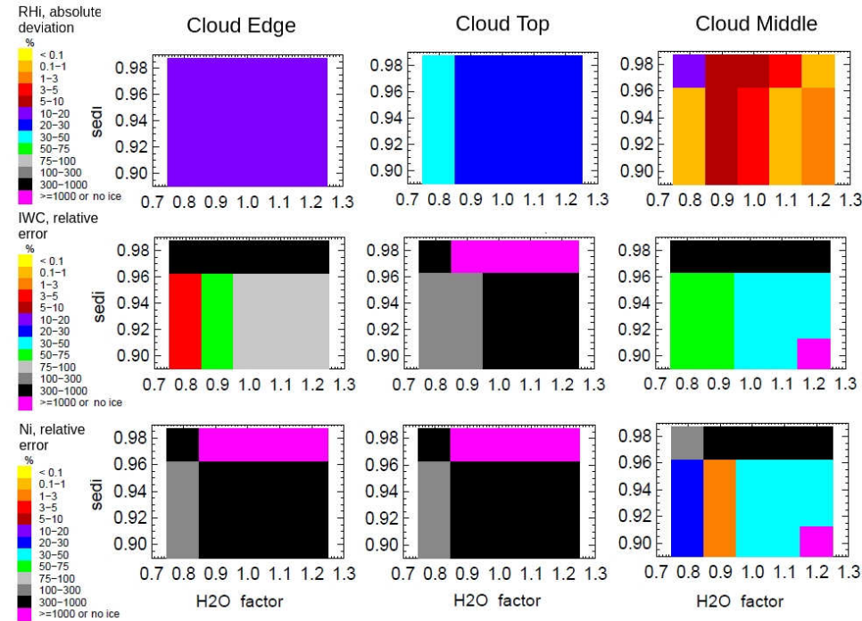
Figure 4.13: Case study II: The model input parameters that led to the best results are quite different for each respective cloud segment. The plot shows the cloud edge (left panels), top (middle panels) and cloud middle (right panels). The top row shows the results from the RH i comparison, middle row: ice water content, bottom row: cloud particle concentrations.
