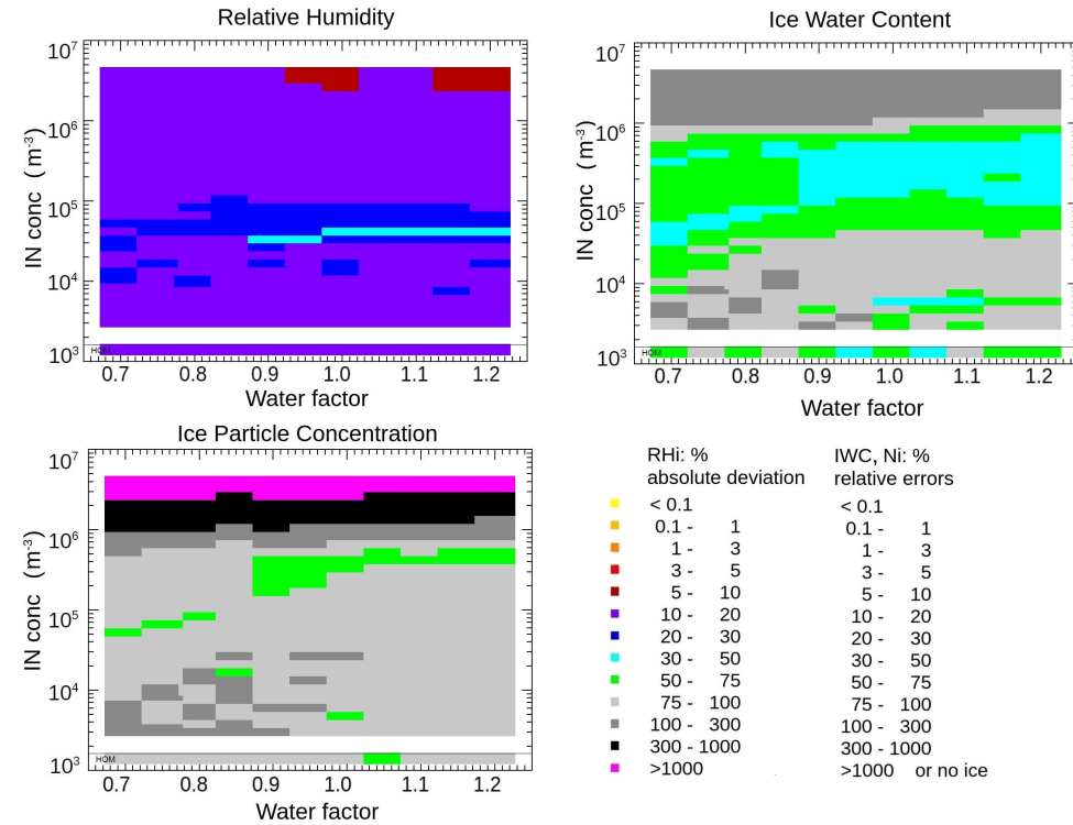
Figure 4.11: 'Continental air' trajectories. Top left: This graph shows the model's deviation from the observed values for 352 model runs with regard to the parameter RH. Each colored square depicts a model/observation comparison of 1100 data points (1 Hz observational data, 1 simulation result per minute interpolated to 1 Hz values). The deviation is given as absolute difference in the simulated and measured RH. The model runs below the horizontal line show the results for a purely homogeneous nucleation; in this case, the initial model concentration for IN is 0 cm -3 . Top right: Model deviation from the observed values for 352 model runs with regard to the parameter IWC. The deviation is given as relative error between the simulated and measured IWC. Bottom left: As top right, but for N ice .
