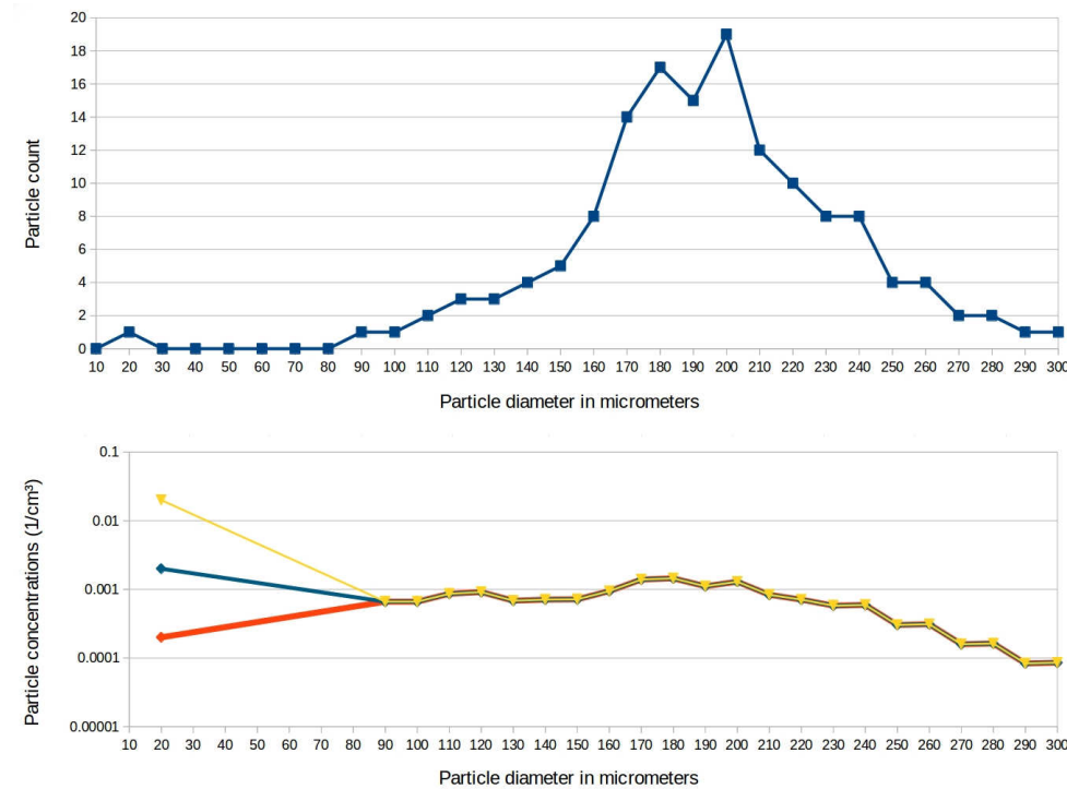
Figure A.7: Particle counts and resulting size distributions for an idealized cirrus cloud measurement. One particle at 20\text{ }\mu\text{m} is recorded. This single particle has a significant influence on the size distribution averaged for 1 second of flight (yellow). When averaging over 10 seconds (blue line), the single particle's influence on the size distribution is still comparable to the numbers obtained by the bulk of larger cloud particles. Only when averaging over 100 seconds (red line), the size distribution gives a hint that the small particle was a rare event compared to the frequent occurrence of large particles.
