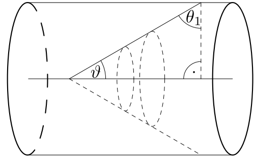
Fig. 2.4: Opening angle of the light cone, which is guided along the fiber
