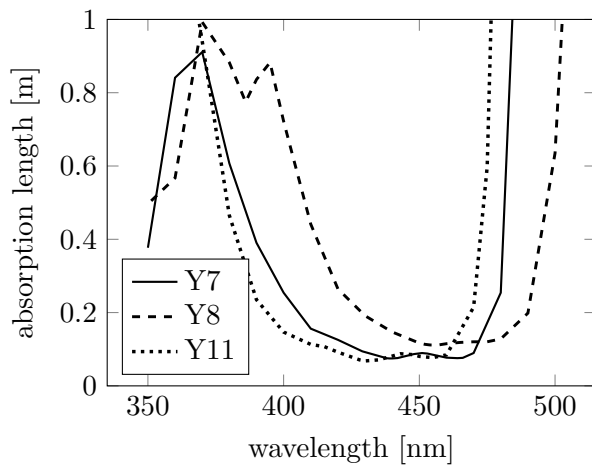
Fig. 4.15: Total optical attenuation length depending on photon wavelength for a dye concentration of 1 \text{ ppm}^{-1} .
