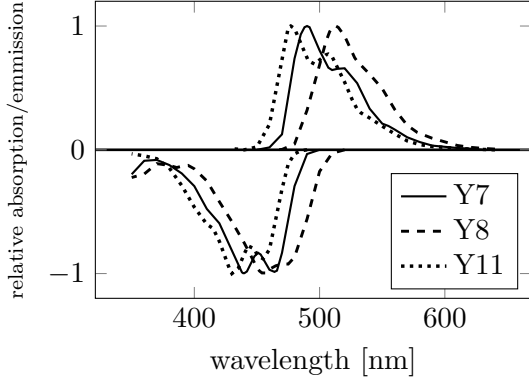
Fig. 4.14: Dye's emission (above 0) and absorption (below zero) spectra of optical light for three different dye types, provided by the manufacturer Kuraray [25].
