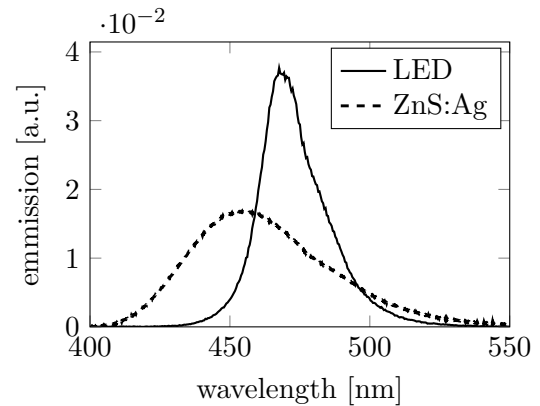
Fig. 5.5: Emmission spectra of the scintillator material and the blue LED used in the transmission measurements.
