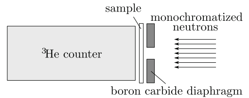
Fig. 5.1: Setup of a neutron absorption measurement.
