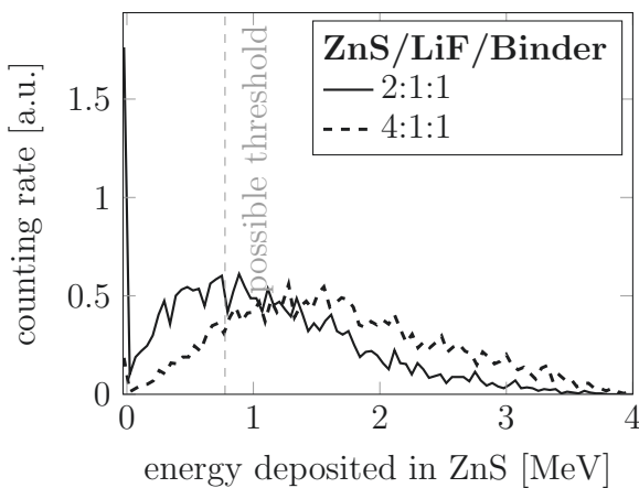
Fig. 6.3: Distribution of energy deposited in ZnS grains. If one assumes a threshold of energy needed to produce enough photons for the neutron to be detected, the efficiency is the area under the curves to the right of the threshold.
