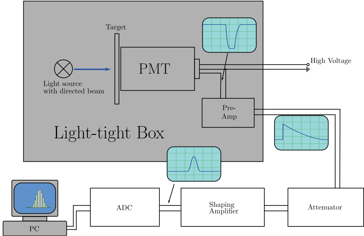
Figure 5.4: Setup for transmission measurements. The PMT signal is amplified in a pre-amplifier and then, if necessary, attenuated by some factor of 2^n . After a shaping amplifier creates pulses for the ADC to digitize, the computer records the pulse data in a histogram.
