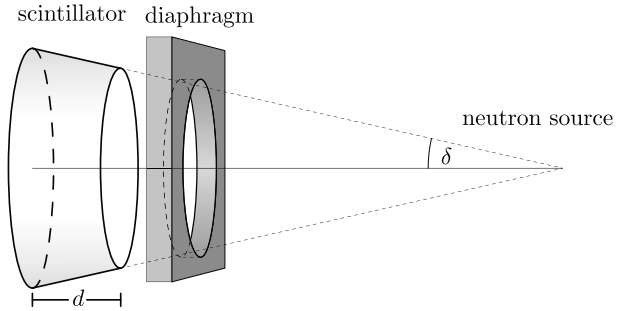
Fig. 5.2: An incoherent neutron beam passes the scintillator plate in a conic section. Almost all neutrons traverse a distance longer than d .
