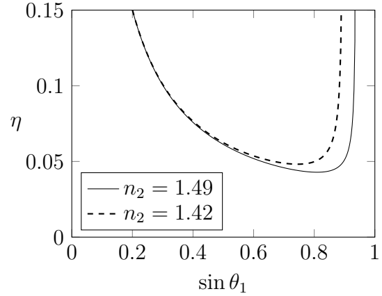
Fig. A.2: Distance travelled in outer cladding per fiber length as calculated in (A.1.2) for n_1 = 1.59 and \xi = 0.03 . For n_2 the two possible refractive indices of outer cladding, PMMA and FP have been chosen.
