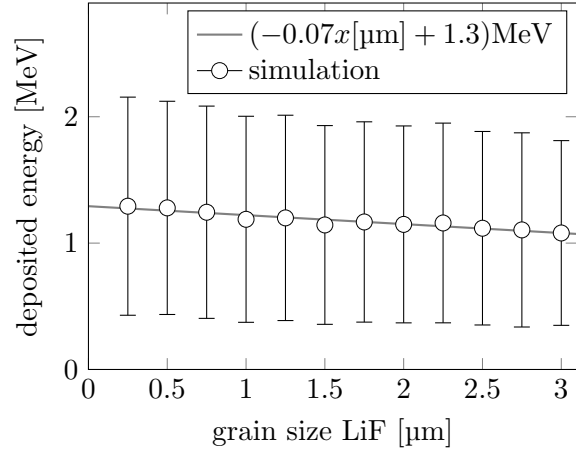
Fig. 7.3: Average amount of energy deposited in ZnS grains for LiF grain sizes smaller than 3\mu\text{m} and default ZnS grain size of 7.5\mu\text{m} . The bars indicate the root mean square deviation of the distribution, the error is a factor 45 smaller since each data point represents 2000 simulated events. The linear fit shows that the average deposited energy is decreasing for increasing LiF grain size.
