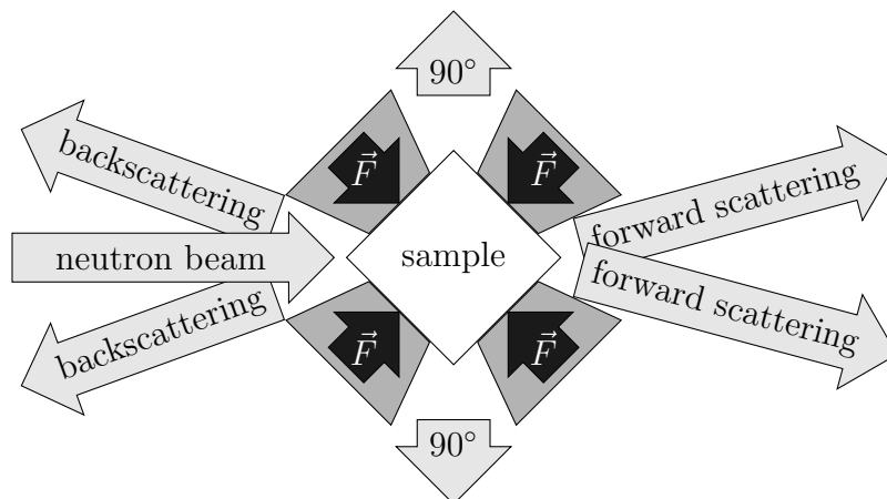
Figure 2.7: Schematic of possible detection directions at the SAPHiR instrument with the sample in the center, four anvils on each side and the neutron beam incoming from the left. The top and bottom anvils are not shown. The anvils exerting pressure on the sample cover much of the solid angle. Thus, only neutrons scattered forward, backward or perpendicular can be examined.
