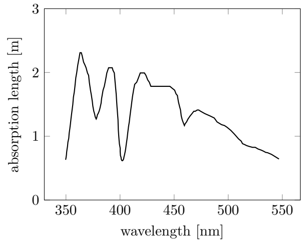
Fig. 4.16: Absorption length of a photon in a clear fiber depending on its wavelength according to [28].
