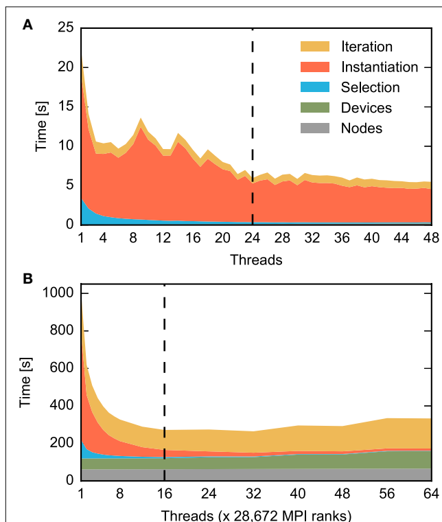
FIGURE 3 | Contributions to construction time for small and large neuronal networks for different numbers of threads. The time required for different construction steps is indicated by color and stacked: time for creation of network nodes (gray) and connecting devices to neurons (green) are shown in total, while the time for connecting neurons to each other using the fixed-indegree algorithm is further divided into the random selection of sources (blue), the instantiation of individual connections (red), and iteration over nodes (yellow). Listing 1 shows correspondingly colored code for the latter three components. A network of fixed size is distributed across increasing numbers of OpenMP threads (strong scaling). The dashed vertical line indicates the number of physical cores available on the compute node. Network construction is performed with instrumented code incurring runtime overhead compared to Figures 1, 5, 7 , see Section 2.5. (A) Construction of the small benchmark. Times required for creation of network nodes and for connections between devices and neurons are not visible. Same network model and machine as in Figure 1 . (B) Construction of a balanced random network model representing 200 million neurons and 2.25 trillion synapses (large benchmark, Table 1 , detailed model specification in Section 2.2.2) on an IBM BlueGene/Q supercomputer ( Table 1 , detailed system specification in Section 2.2.1). The benchmark emulates distributed computing on a constant number of 28,672 compute nodes coupled by MPI while the number of OpenMP threads on each node is increased using the dryrun feature of NEST (Kunkel et al., 2014).
