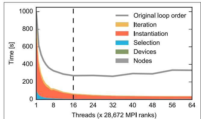
FIGURE 6 | Time required for the construction of the large neuronal network using the alternative loop order. Color code and data ranges are the same as in Figure 3B showing the construction time prior to the reorganization of loops. The times required to create the network nodes and to connect devices and neurons are too small to be visible in the present graph. Listing 3 illustrates the algorithm. The gray curve shows the total construction time from Figure 3B for comparison. The dashed vertical line indicates the number of physical cores available on a compute node. The double-logarithmic representation of the same data in Figure 7 illustrates the scaling at large numbers of threads. Network construction is performed with instrumented code incurring runtime overhead compared to Figure 7 , see Section 2.5.
