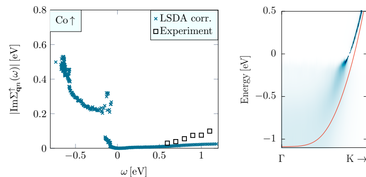
Figure 4.21: Quasiparticle lifetime broadening and dispersion anomaly caused by the electron-magnon interaction for a majority band in cobalt which crosses the Fermi level along the \Gamma to K direction. Left: imaginary part of the quasiparticle solution (blue crosses) compared to experimental data [60] (black squares). Right: single-particle band (red line) and its renormalized spectral functions shown as a blue color-coded map. The corrected LSDA Green function serves as starting point, the Fermi level is set to zero.
