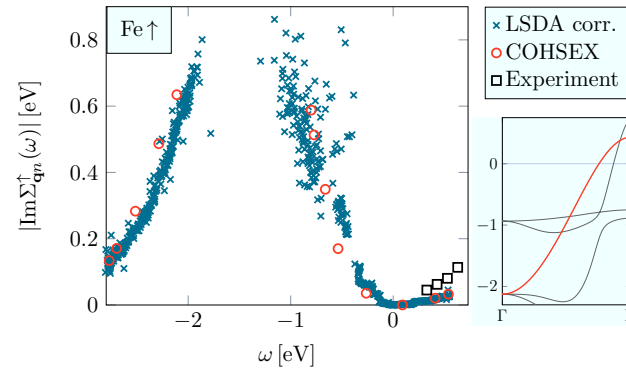
Figure 4.16: Starting-point dependence of the quasiparticle inverse lifetime employing the corrected LSDA (blue crosses) and the COHSEX Green function (red circles) compared to experimental values (black squares) taken from Knorren et al. [60]. The quasiparticle inverse lifetime is calculated for a majority band along the \Gamma to N direction shown as the red thick line in the inset.
