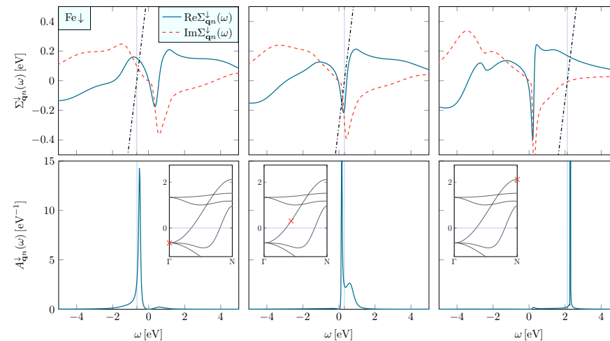
Figure 4.14: Same as Fig. 4.13 for a minority band along the \Gamma to N direction in iron. The dash-dotted line in the upper panel corresponds to \omega - \epsilon_{qn}^{\downarrow} .
