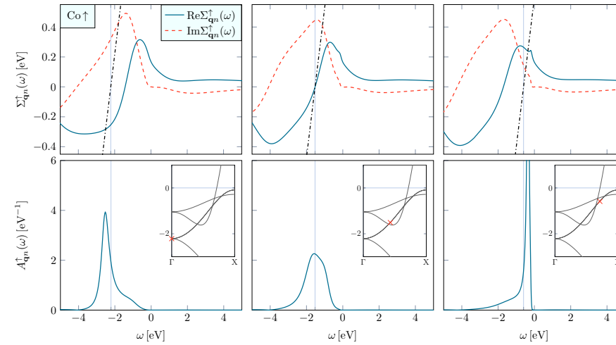
Figure 4.19: Same as Fig. 4.13 for a majority band along the \Gamma to X direction in cobalt.
