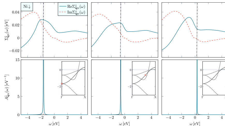
Figure 4.24: Same as Fig. 4.14 for a minority band along the \Gamma to X direction in nickel.
