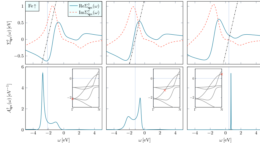
Figure 4.13: Self-energy (upper row) and the corresponding spectral function (lower row) for three majority states of a band along the \Gamma to N direction in iron. The insets of the spectral function show the band structure along that \mathbf{k} direction and the considered state is indicated as a red cross. The single-particle energy is indicated as a grey thin vertical line in the upper and lower panel. The dash-dotted line (upper panel) corresponds to \omega - \epsilon_{qn}^{\uparrow} and its intersection with the self-energy indicates a quasiparticle solution. The self-consistent COHSEX Green function serves as starting point for the GT self-energy calculation. The Fermi level is set to zero.
