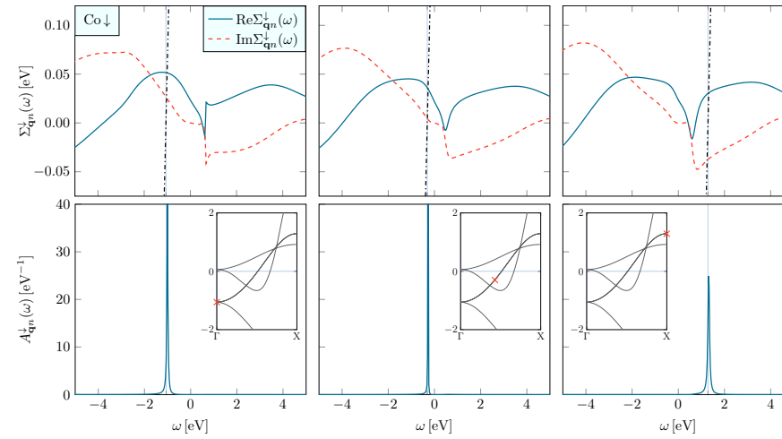
Figure 4.20: Same as Fig. 4.14 for a minority band along the \Gamma to X direction in cobalt.
