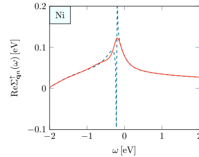
Figure 4.10: The analytic continuation of a Padé approximation can lead to spurious peaks in the result in rare cases (blue dashed line). To smoothen such numerical artifacts the result of multiple Padé approximations is averaged (red solid line).
