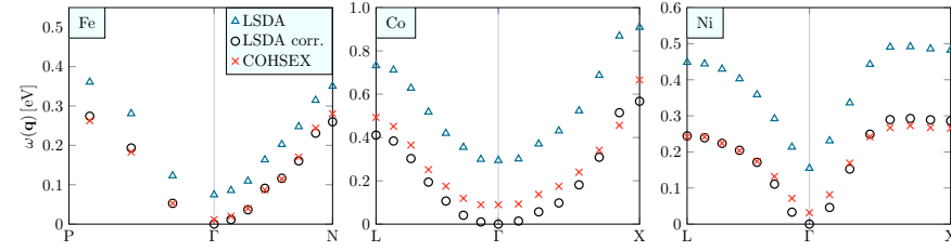
Figure 3.5: Starting-point dependence of the spin-wave spectra for Fe, Co, and Ni obtained with the LSDA (blue triangles), corrected LSDA (black circles), and COHSEX (red crosses) Green function. The spin-wave dispersion is shown along the high-symmetry line P \rightarrow \Gamma \rightarrow N and L \rightarrow \Gamma \rightarrow X for the bcc and fcc lattice structure, respectively. This figure was published recently [51], ©2016 American Physical Society.
