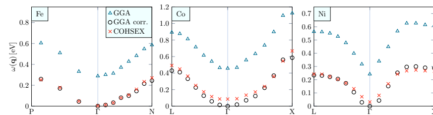
Figure 3.6: Same as Fig. 3.5 for a GGA starting point.
