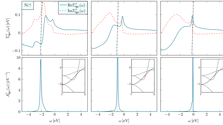
Figure 4.23: Same as Fig. 4.13 for a majority band along the \Gamma to X direction in nickel.
