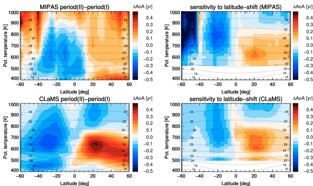
Figure 5. Top: Difference of MIPAS zonal mean age of air distributions between the periods I and II (left), compared to the effect of a shift of the zonal mean age of air distribution of period I according to the altitude dependent latitude shifts of the subtropical transport barriers as derived for MIPAS (Fig. 2, bottom right panel, blue lines) (right). Bottom: The same for CLaMS zonal mean age of air.
