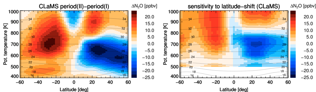
Figure 4. Difference of CLaMS zonal mean \text{N}_2\text{O} distributions between the periods I and II (left), compared to the effect of a shift of the \text{N}_2\text{O} zonal mean distribution of period I according to the altitude dependent latitude shifts of the subtropical transport barriers as derived for CLaMS (Fig. 2, bottom right panel, orange lines) (right).
