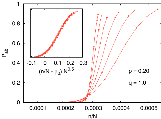
FIG. 11. Probabilities P_{ab} versus seed size n/N , for p = 0.20 and q = 1 . Each curve corresponds to one value of N , with N = 2^{20}, 2^{21}, \dots, 2^{25} (steeper curves correspond to larger N ). The inset shows a data collapse, obtained by plotting these data against [n/N - \rho_0(p, q)]N^x with \rho_0 = 0.000282 and x = 0.5 .
