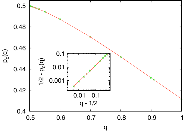
FIG. 17. Critical value of p versus q , for square lattice and algorithm with delay. The inset shows a log-log plot which suggests Eq. (11) for q \approx 1/2 .
