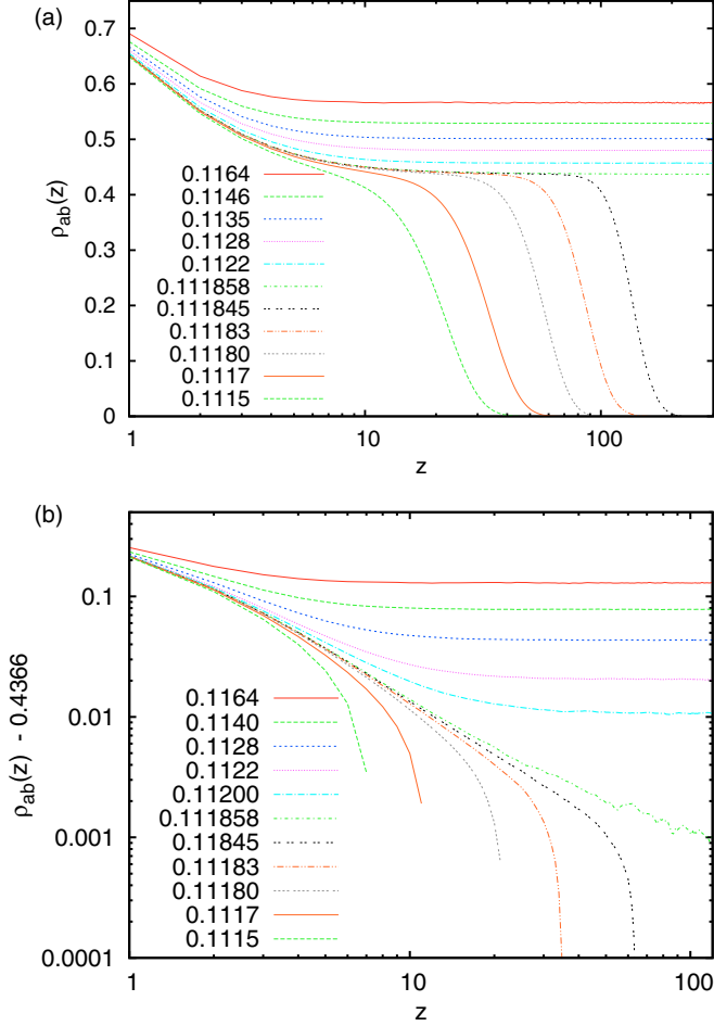
FIG. 28. (a) Densities of ab sites at given height z , after the cluster had stopped growing at this height, for q = 1 and various values of p . Panel (b) shows the same data replotted as a log-log plot of \rho_{ab}(z) - \rho_{ab,c} against \ln z .
