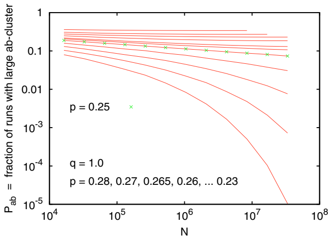
FIG. 5. Fraction of events that lead to giant ab clusters which contribute to the peaks in Fig. 3. Each curve corresponds to one value of p , while q = 1 for all curves. The curve for p = p_c is indicated by crosses.
