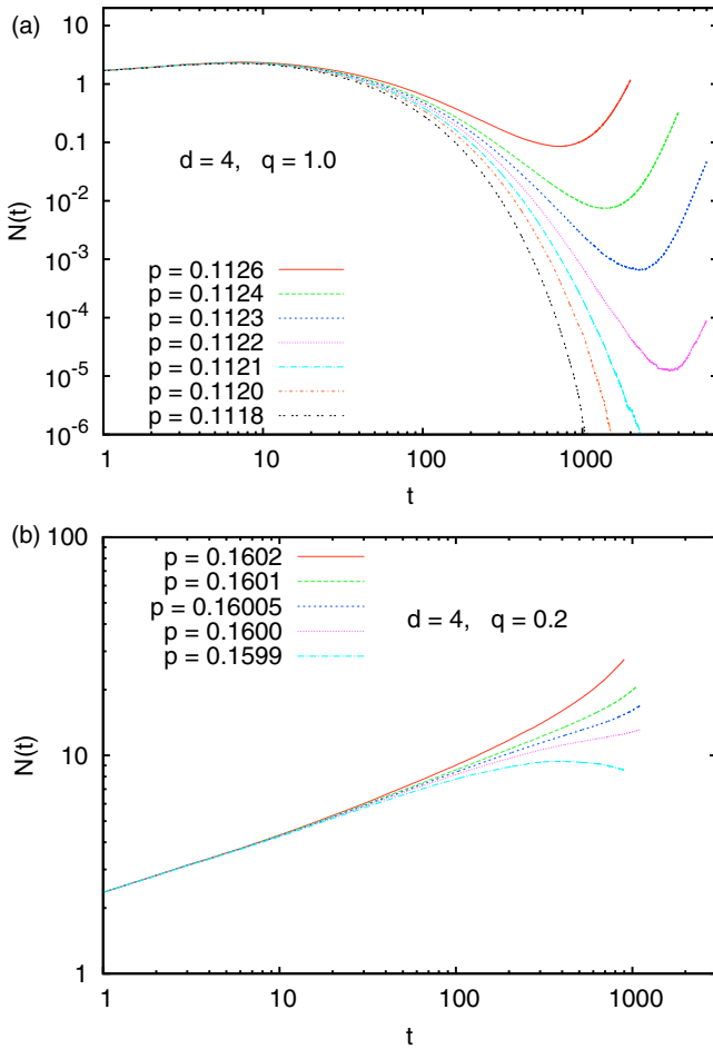
FIG. 20. Log-log plots of N(t) versus t for 4-d simple hypercubic lattices. For this lattice, ordinary bond percolation has p_c = 0.16013(1) [51]; thus all curves except the uppermost one in panel (b) correspond to p < p_c . Panel (a) shows results for q = 1.0 . The best estimate for p_c(q = 1.0) from these data is \approx 0.112 , but a more precise estimate will be given later. Panel (b) is for q = 0.2 . Here cooperativity is much weaker, and thus our estimate p_c(0.2) = 0.15997(5) is much closer to the value for OP. Superficially, this plot might suggest a power law and thus a second order transition, but all structures seen in this plot are real (statistical errors are much smaller than the line thicknesses) and suggest also a (weak) first order transition.
