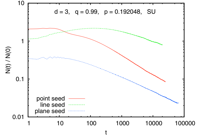
FIG. 43. Log-log plot of N(t)/N(0) against t , at p = p_c , for three types of initial conditions: Point seeds, planar seeds, and seeds consisting of every second point on a long straight line. In spite of the large corrections to scaling, the data seem compatible with a power law with common exponent -0.38(3) .
