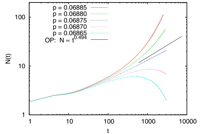
FIG. 36. Log-log plot of N(t) for the algorithm with delay, using again a single doubly infected seed site (but, for a small change, q = 1 ). But now any site could infect 14 other sites as described in the text.
