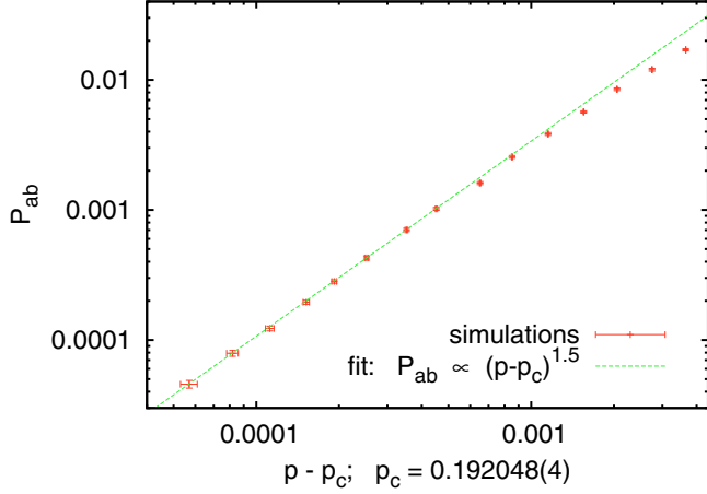
FIG. 41. Log-log plot of P_{ab} against p - p_c . In contrast to the 4-d case (Fig. 22) we now see a clear power law, with exponent compatible with 3/2 . For this and the following two figures we used q = 0.99 .
