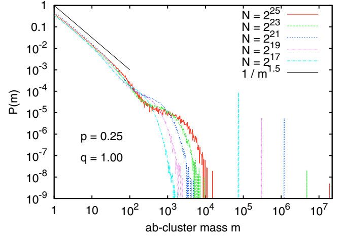
FIG. 3. Mass distribution of ER network at p = 0.25 and q = 1.0 . Each curve corresponds to a fixed network size. The vertical lines on the right hand side are very narrow peaks, whose widths are smaller than the linewidth. The straight full line indicates the power law P(m) \propto m^{-3/2} .
