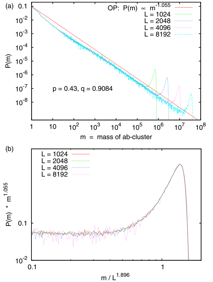
FIG. 15. Upper panel: Mass distributions of ab clusters obtained with the algorithm without delay at the critical point for q = 0.9084 . Lattice sizes are L \times L with L = 2^{10}, \dots, 2^{13} , and helical boundary conditions were used. The straight line indicates the scaling P(m) \sim m^{1-\tau} with \tau = 187/91 for ordinary percolation. Lower panel: Data collapse of the high-mass data, obtained by plotting m^{\tau-1}P(m) against m/L^{D_f} , where D_f = 91/48 is the fractal dimension of the giant cluster in OP [43].
