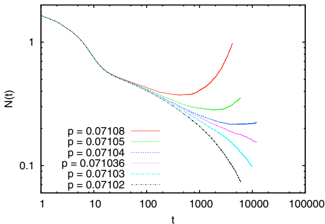
FIG. 37. Log-log plot of N(t) for the algorithm with delay, using again a single doubly infected seed site with q = 1 . But now any site can infect 12 other sites which are distances 1 and 2 away on the coordinate axes (see text).
