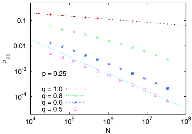
FIG. 8. Log-log plot of the probabilities P_{ab} to generate large ab clusters versus N . Each curve is for a different value of q , while p is fixed at the critical point p = 1/\langle k \rangle . The two straight lines indicate power laws N^{-0.123} (which gives a perfect fit for q = 1 ) and N^{-0.67} , which is the asymptotic value for q < 1 .
