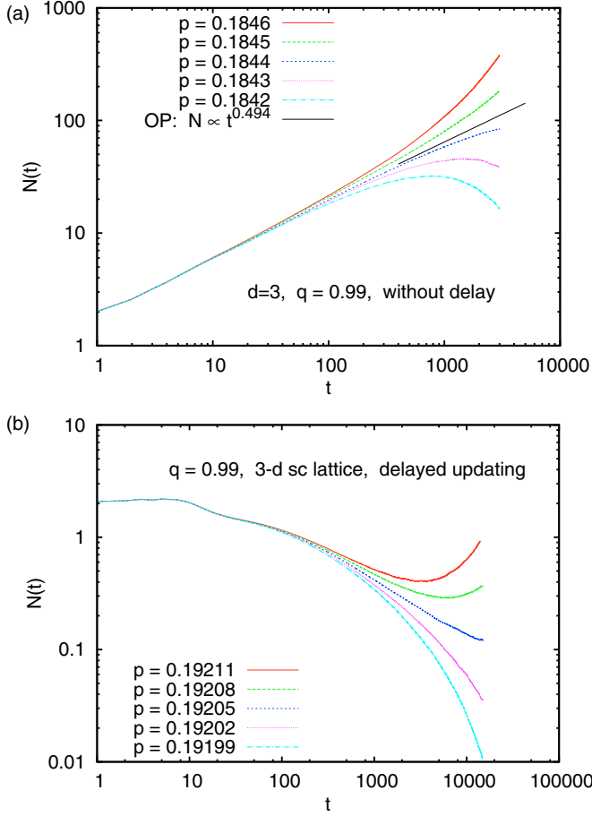
FIG. 33. Log-log plot of N(t) against t , for cooperative percolation on the simple cubic 3-d lattice with q = 0.99 . Each curve is based on many runs with doubly infected point seeds, and care was taken that the infected cluster never reached the boundary. Error bars are smaller than the line thicknesses. Panel (a): Data obtained by the algorithm without delay. The solid straight line represents the scaling for OP. Panel (b) shows data for the algorithm with delay.
