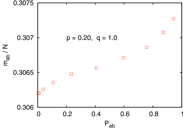
FIG. 10. Average masses of “giant” ab clusters for N = 2^{20} , p = 0.20 , and q = 1 , plotted against the probability to obtain such giant ab clusters. Each point corresponds to a different value of n , where n is the size of the “seed” (the number of initially infected nodes). The values of n are 200, 240, 280, \dots , 560, with n increasing from left to right.
