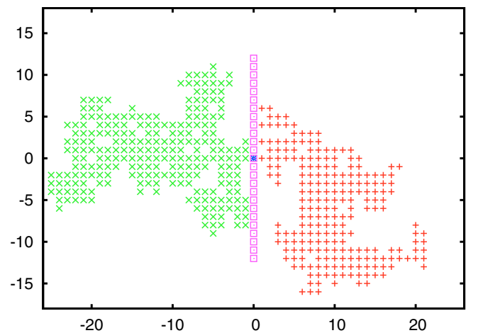
FIG. 19. Two ordinary (bond) percolation clusters, both starting at x = 0 , with a killing wall ( x = 0 ) between them. A wall is killing if any epidemic that tries to infect it is entirely deleted.
