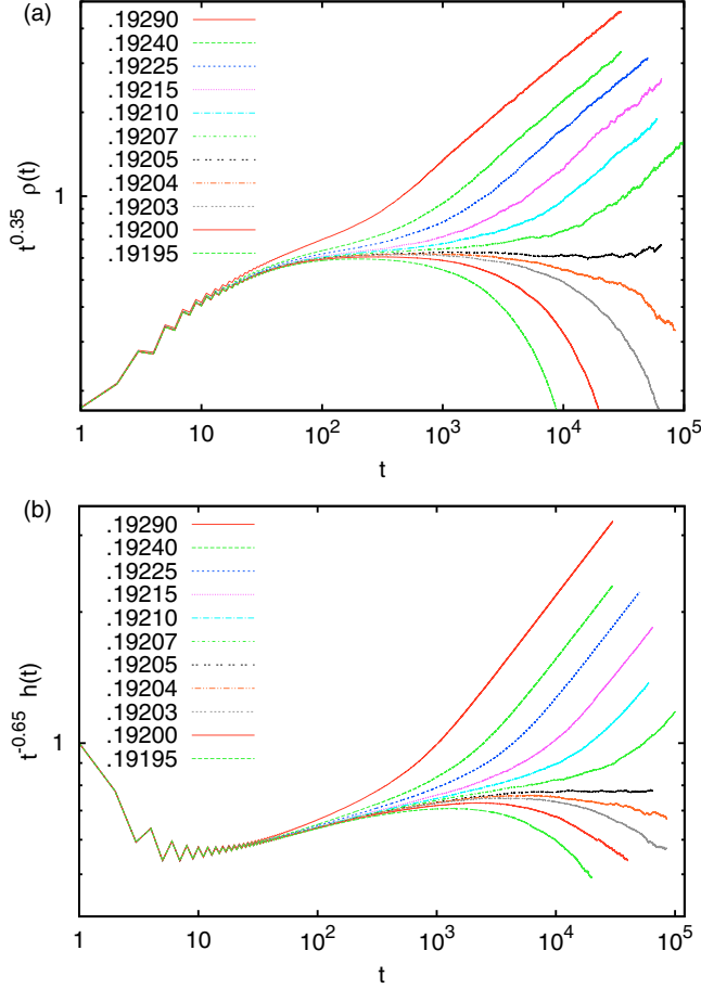
FIG. 38. Log-log plot of densities of infected sites and of their average heights versus t . We used here the algorithm with delay and with q = 0.99 . The sc lattice was used as in Figs. 33(b) and 35, but now the seed consisted of the set of all even points on an entire L \times L base surface of an L \times L \times L_z cuboid with helical lateral boundary conditions as described in the text. Sizes of the base plane ranged from 2^{20} to 2^{23} sites. As in the 4-dimensional case, we actually plotted the data multiplied by a suitable power of t which makes the critical curve roughly horizontal for large t . Panel (a) shows \rho(t) = N(t)/L^2 , while panel (b) shows \rho(t) .
