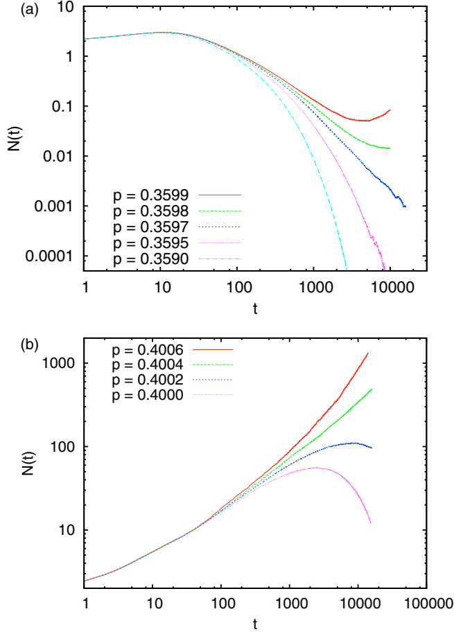
FIG. 44. Log-log plots of N(t) versus t for d = 2 , q = 1 , and several values of p close to the critical point. In each panel we used two initially infected neighbor sites, one infected by A and the other by B . In panel (a) the contacts are power law distributed with \sigma = 1.1 , while \sigma = 1.5 for panel (b).
