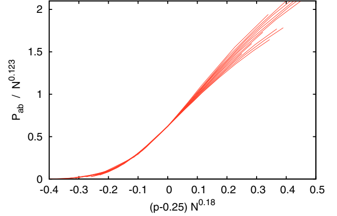
FIG. 6. Same data as in Fig. 5, but plotted in a way that suggests a data collapse according to the FSS ansatz Eq. (10).
