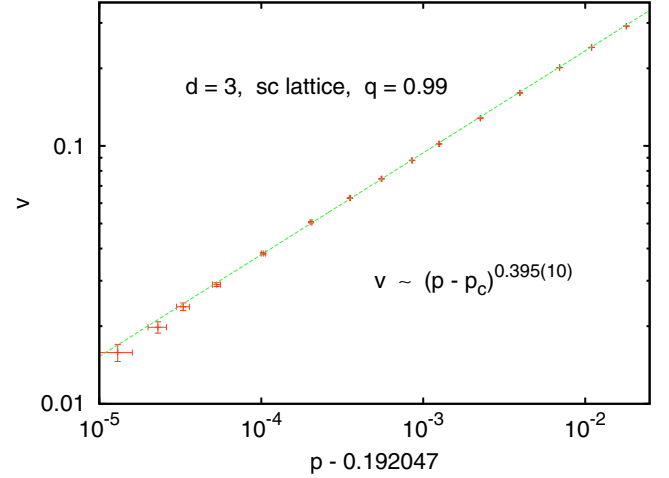
FIG. 39. Log-log plot of the speed v = \lim_{t \rightarrow \infty} h(t)/t against p - p_c . The straight line represents a power law fit for 0.19215 \leq p \leq 0.1922 . For p < 0.1921 the data are unreliable due to possible finite size and finite time corrections.
