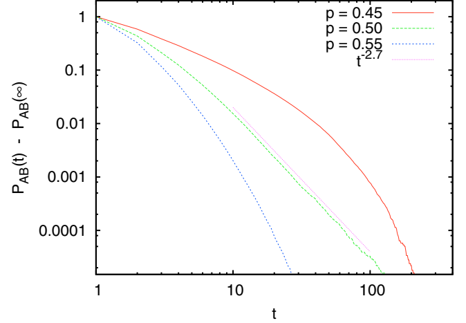
FIG. 18. Log-log plots of P_{AB}(t) - P_{AB}(\infty) versus t for 2-d lattices with q = 1 . The central curve corresponds to the critical point for single diseases. The straight line indicates its exponent for large t .
