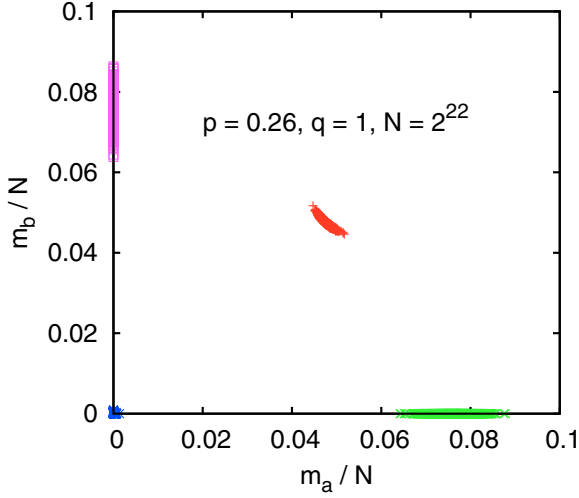
FIG. 7. Scatter plot of the joint distribution of single-disease clusters, for p = 0.26 and q = 1.0 . Each of the four clusters of points is well separated from the others, and corresponds to the cases of no giant outbreak, giant outbreaks of only one disease, and outbreaks of both diseases. In the latter case (and only then) also the cluster of nodes which have both diseases is large.
