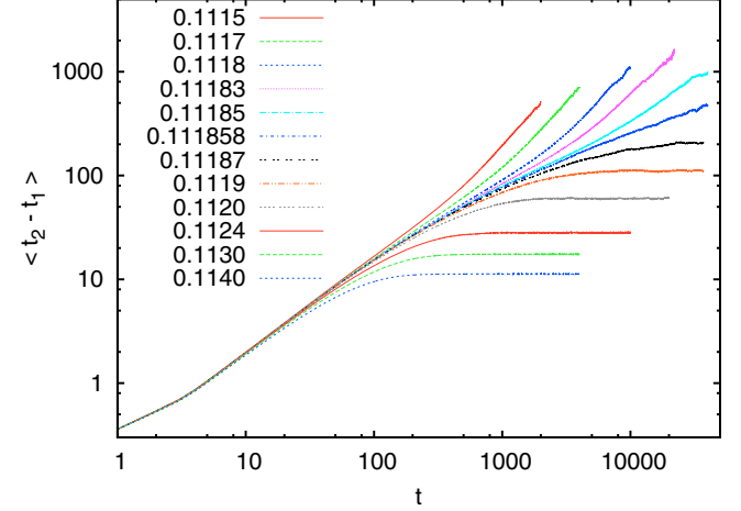
FIG. 30. Average time lags between first and second infections of sites whose second infection happened at time t , plotted against t .
