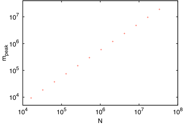
FIG. 4. Positions of the right hand peaks in Fig. 3, i.e., average masses of the “giant” ab clusters, for p = 0.25 and q = 1.0 , plotted against N . Error bars are smaller than the symbol sizes. The data are fitted perfectly by a straight line with slope 1; i.e., giant ab clusters contain a fixed fraction of the nodes.
