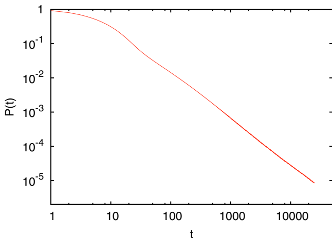
FIG. 42. Log-log plot of P(t) against t , at p = p_c . The data are compatible t^{-1.37(5)} , while the analogous plot for d = 4 would have given a faster decay, similar to the p = p_c curve in Fig. 20(a).
