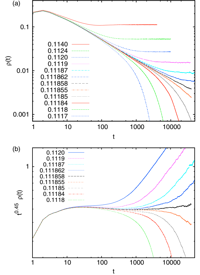
FIG. 23. (a) Log-log plots of \rho(t) = N(t)/L^3 versus t for d = 4 and q = 1.0 , when using all sites of an entire hyperplane z = 0 as seeds. Lateral boundary conditions are helical, and the diseases are allowed to spread into the positive z region only. (b) Part of the same data, but shown as t^\delta \rho(t) against t , with \delta = 0.45 . Since the data for small t have obviously large nonscaling corrections, only data for t > 10 are plotted.
