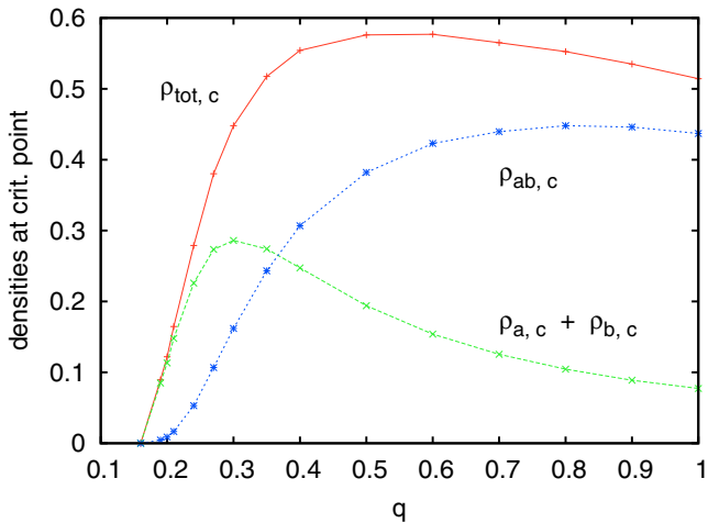
FIG. 32. Densities of singly and doubly infected sites at the critical point. They vanish only at q = 0.16013 which is the critical point for single epidemics.
