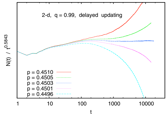
FIG. 16. Log-linear plots of t^{-0.5843}N(t) versus t for q = 0.99 and for five values of p close to the critical point. The exponential prefactor is chosen such that the curve should be asymptotically flat for p = p_c .
