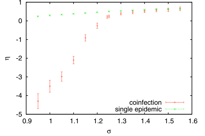
FIG. 45. Exponents \eta for the growth of the number of infected sites, plotted against the Lévy exponent \sigma controlling the decrease of the infection probability with distance. For comparison, we also show the analogous exponents for single epidemics, taken from [68]. The exponents were estimated from plots like the two previous ones, by finding for each \sigma the critical value p_c of p where the curve looks most likely to become straight for t \rightarrow \infty . The error bars reflect essentially the uncertainty in the determination of p_c .
