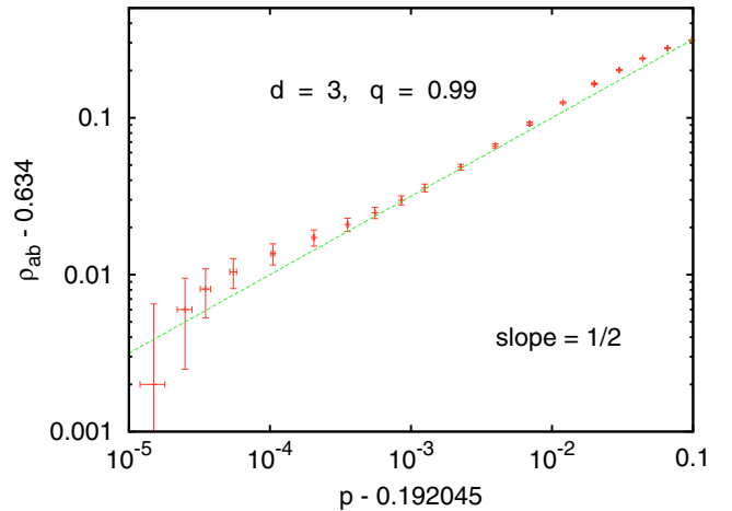
FIG. 40. Log-log plot of \rho_{ab}(\infty) - \rho_{ab,c} against p - p_c , similar to the inset of Fig. 29. The huge error bars on the points for small p are due to possible finite size and time corrections.
