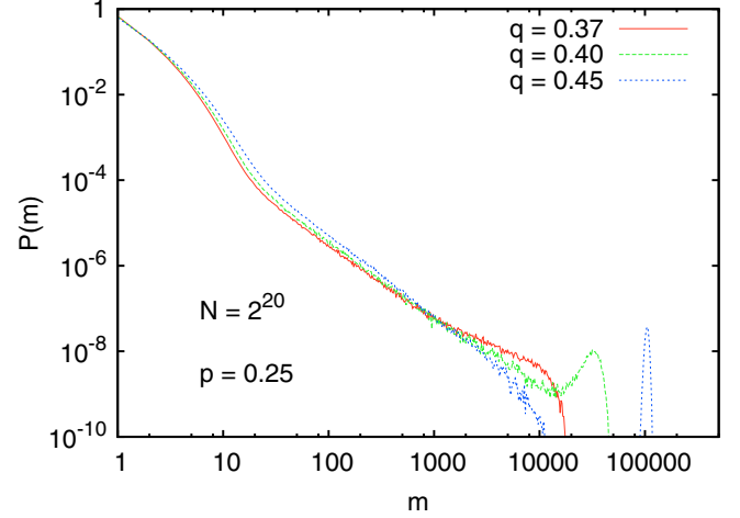
FIG. 9. Mass distributions analogous to Fig. 3, but for three values of q slightly larger than q^* . One sees clearly that the two peaks coalesce as q^* is approached. Data for q = q^* are not shown due to the much larger finite size effects which make their interpretation difficult.
