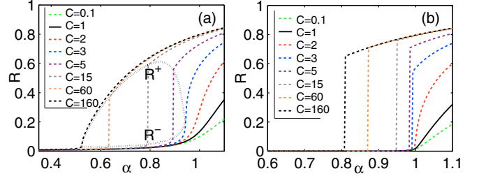
FIG. 2. Order parameter R = 1 - S_\infty plotted against \alpha for (a) \epsilon = 0.005 (where \epsilon is the initial fraction of sick agents) and (b) \epsilon = 10^{-4} . Each curve corresponds to a different level of cooperativity C . The dotted lines in panel (a) indicate the upper and lower limits R^+ and R^- of the jumps at the first order transitions.
