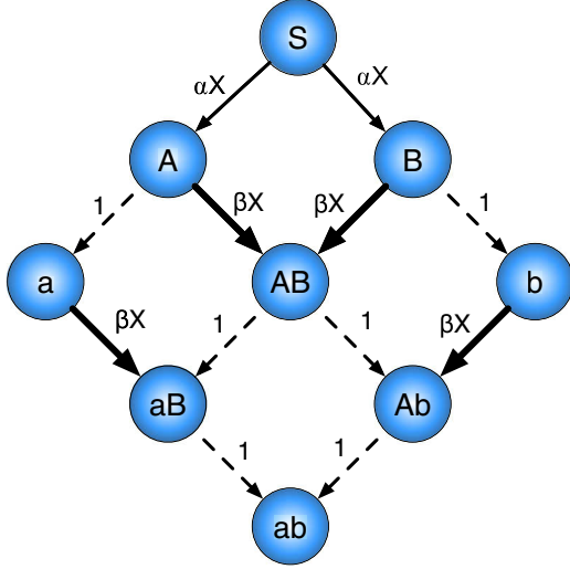
FIG. 1. Flow chart in two-disease coinfection with A, B symmetry and restrictions on the infection rates as discussed in the text. Capital letters A and B represent infective states; lowercase letters a and b stand for “recovered” ones. Infecting neighbors are not indicated explicitly, but it is assumed that all individuals infected with disease A , say, have the same chances to pass A on to another individual. Thus every infection process occurs with a rate proportional to the fraction X of the population having the corresponding disease.
