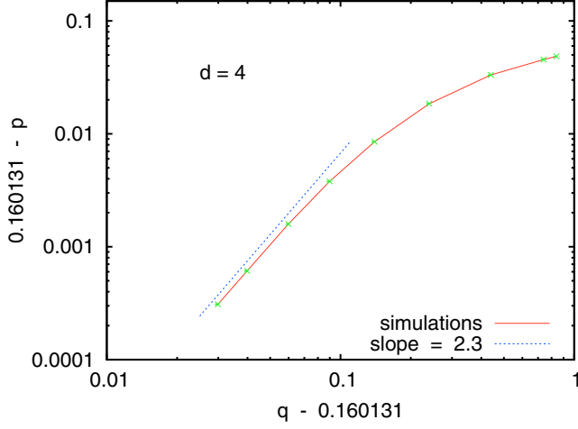
FIG. 24. Log-log plot of p_c - p_c(q) against q - p_c , where p_c = 0.160131 [60] is the (bond) percolation threshold on the simple 4-d hypercubic lattice.
