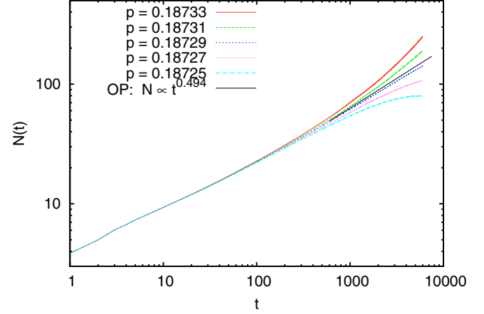
FIG. 35. Analogous to Fig. 33(b), but now the epidemics start at two neighboring sites on the simple cubic lattice. As in Fig. 33(a), the solid straight line represents the scaling for OP.
