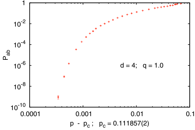
FIG. 22. Log-log plot of P_{ab} , the probability that a single doubly infected site evolves into a giant epidemic, plotted against p - p_c . As in the previous plots, AU was used with q = 1 .
