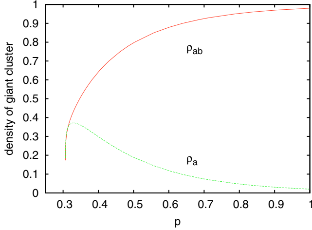
FIG. 46. Plots of the a and ab densities of giant clusters, for multiplex networks with q = 1 . Within the accuracy of the plot, identical results were obtained by direct simulations and by simulating disease A on randomly located b 's with density given by Eq. (25). System sizes were between 2^{20} and 2^{25} sites, with no visible dependence on the size.
