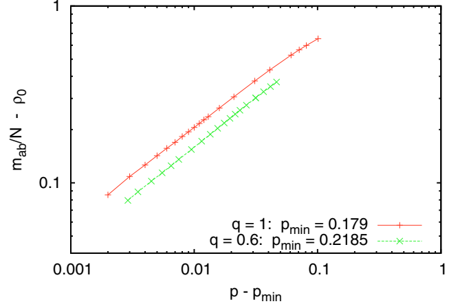
FIG. 12. Relative sizes of giant ab clusters versus p - p_{\min} for two values of q . Both curves are compatible with power laws with exponents 0.57(3), provided one subtracts the density of seed nodes.
