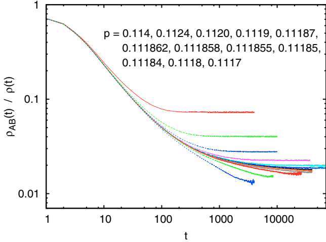
FIG. 31. Fractions of sites which get both infections, and where these infections arrive at the same time t . This is analogous to Fig. 21 where data were shown for point seeds.
