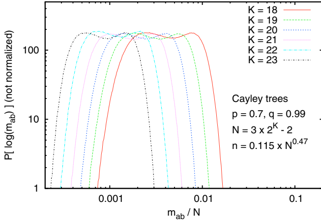
FIG. 13. Distributions of the number m_{ab} of ab nodes in the final state for Cayley trees with k = 3 . More precisely, P(\log m_{ab}) = m_{ab}P(m_{ab}) is plotted against \log[m_{ab}/N] for Cayley trees with K generations, K = 18, \dots, 23 . All curves correspond to p = 0.7 and q = 0.99 . The number n of seed nodes is chosen such that both maxima have the same height. Overall normalization is arbitrarily chosen such that also all curves have the same maximal height.
