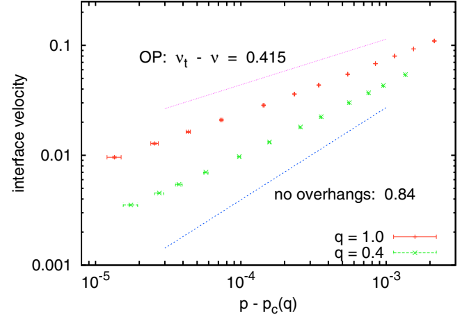
FIG. 27. Log-log plots of v(p) versus p - p_c(q) for d = 4 . The two data sets are for q = 0.4 and q = 1.0 . In this plot we used p_c(0.4) = 0.1416425(20) and p_c(1.0) = 0.1118565(15) .
