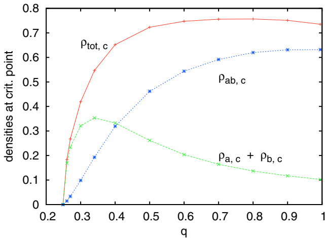
FIG. 34. Analogous to Fig. 32, but now for the sc lattice updated with algorithm SU (i.e., with delay). In contrast to Fig. 32, these data were obtained by starting from single seeds, but using the more precise critical point estimates obtained with planar seeds.
