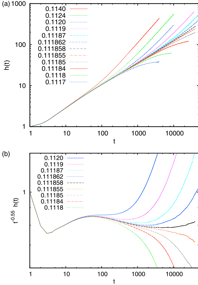
FIG. 26. (a) Log-log plots of h(t, p) versus t for d = 4 and q = 1.0 , when using all sites of an entire hyperplane z = 0 as seeds. These data are based on the same runs as those in Fig. 23. Part of these data are also shown in panel (b) as t^{-\nu_t/\nu_l} h(t, p) versus t .
