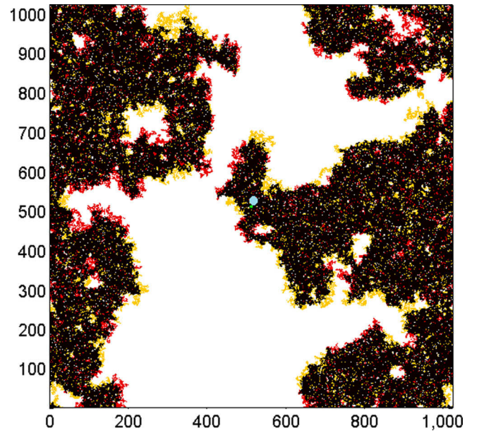
FIG. 14. Final state of a coinfection outbreak on a 2D 1024 \times 1024 lattice at q = 0.99 and p = 0.4504 \approx p_c(q) with periodic boundary conditions and using the algorithm with delay. The single seed of infection is located in the center of the lattice, as marked by the blue disk.
