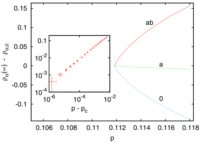
FIG. 29. Asymptotic (for z \rightarrow \infty ) densities of singly, doubly, and not at all infected sites plotted against p , for p > p_c(1.0) . To show all three curves on the same plot, we actually show \rho_\alpha(\infty) - \rho_{\alpha,c} ; i.e., we subtracted the critical densities. For the latter we used \rho_{ab,c} = 0.4366 , \rho_{a,c} = 0.03865 , and \rho_{0,c} = 0.4861 . The inset shows a log-log plot of \rho_{ab}(\infty) - \rho_{ab,c} against p - p_c .
