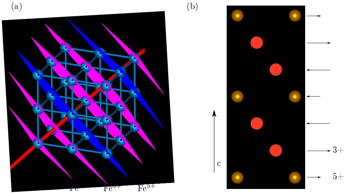
Figure 6.1: (a) Charge ordering of LSFO along the [111] -direction (red arrow) of the pseudo cubic unit cell. The ordering vector for the charge ordered phase is \vec{q}_{\text{CO}} = (1/3, 1/3, 1/3) . The colored planes perpendicular to the [111] -direction indicate the position of the \text{Fe}^{3+} and \text{Fe}^{5+} , respectively. (b) depicts the charge and magnetic ordering in space group R\bar{3}c projected onto the (010) plane. The arrows show the different spin states of \text{Fe}^{3+} and \text{Fe}^{5+} . Adapted from [94]. Sketches are generated with VESTA [14].
