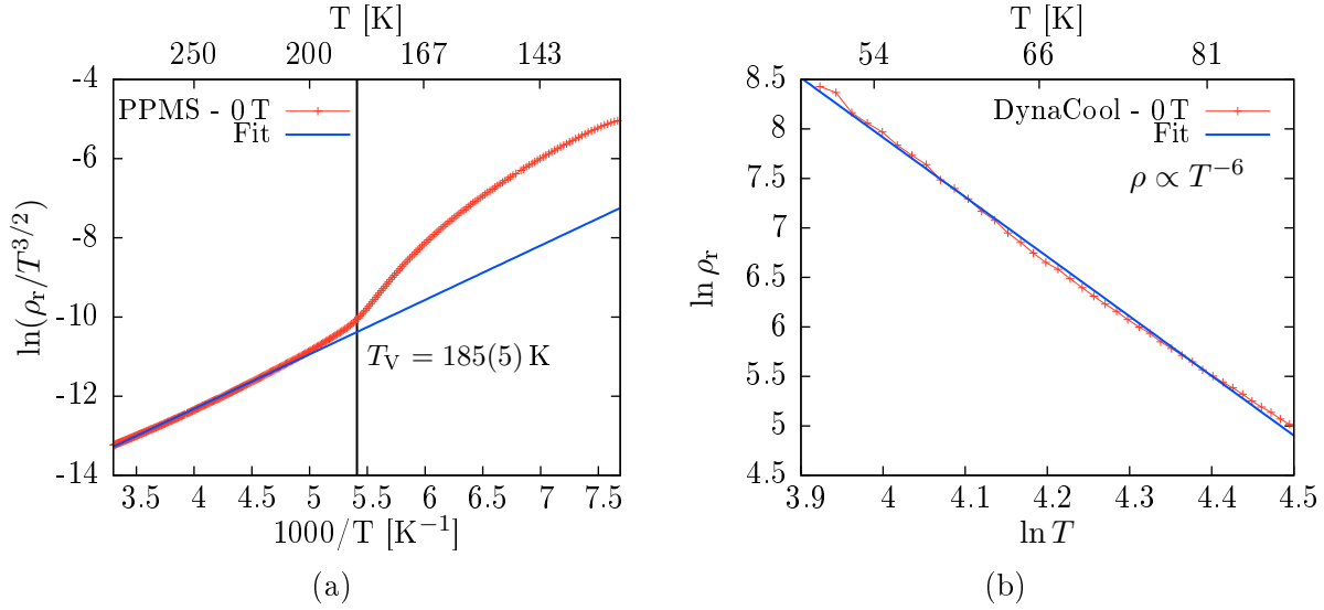
Figure 6.38: (a) Replot of the data in order to fit the non-adiabatic small polaron model. The vertical line indicates the position of the transition temperature T_V . (b) Double ln plot to determine the power law eq. 6.7 according to [40]. The used temperature range was selected to be far below the transition temperature.
