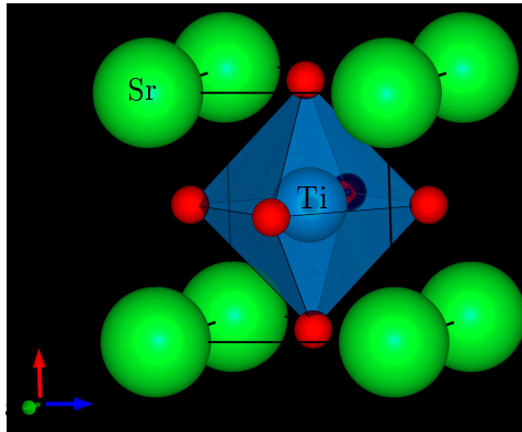
Figure 2.1: Cubic perovskite structure of STO. The A-site is occupied by Sr atoms, the B-site by Ti atoms. The blue marked octahedron specifies the oxygen environment, which is characteristic for the perovskite structure. The dedicated space group is \text{Pm}\bar{3}\text{m} . The figure was made with VESTA [14].
