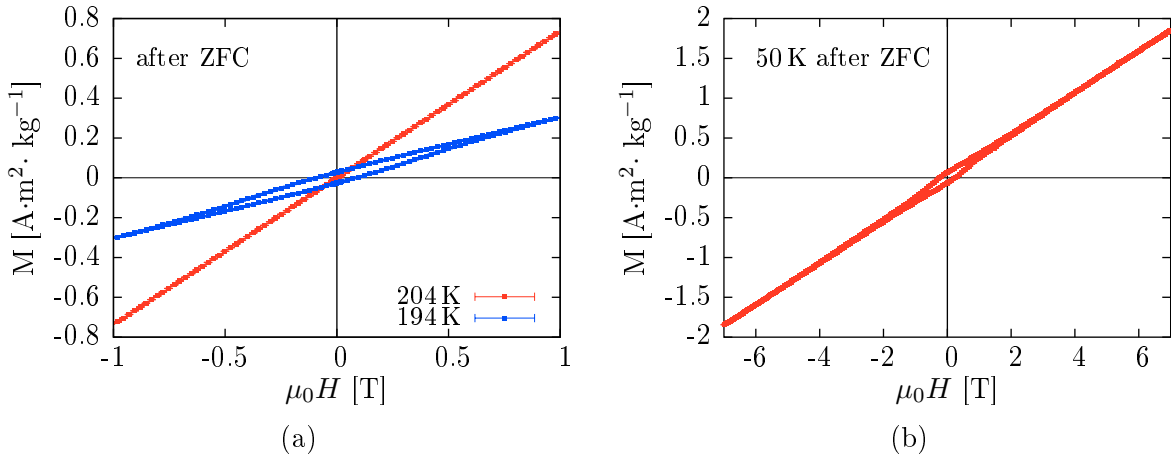
Figure 6.11: M - H -measurements at different temperatures after zero-field cooling. (a) shows a measurement right above (204K) and below (194K) the phase transition. (b) shows a measurement at 50 K for high magnetic fields, but saturation of the magnetization cannot be reached.
