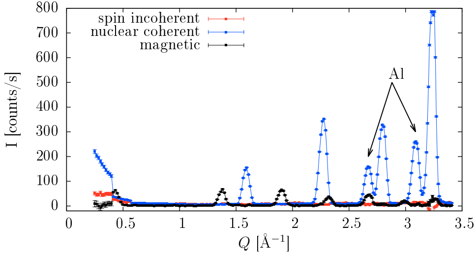
Figure 6.12: DNS measurement performed at 5 K without self-normalization. Separation of the different contributions has been done with dnsploot. Additionally, the two labeled reflections are Al (111) and (200). Aluminium has been used as sample holder and sample environment.
