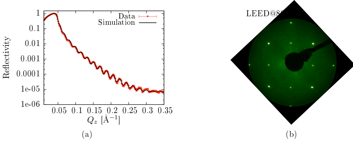
Figure 6.31: (a) XRR data and simulation. The parameters are shown in Tab. 6.7. (b) LEED image taken at 80 eV. Very sharp reflections confirm the good surface morphology of the sample.
