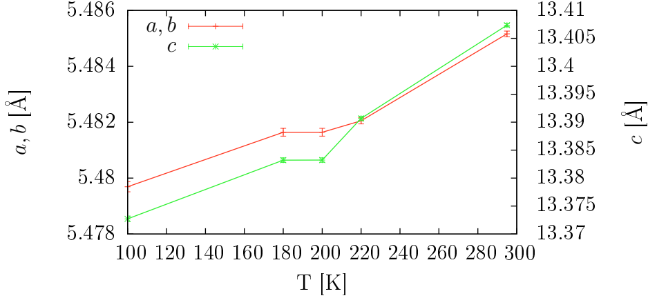
Figure 6.18: Temperature dependence of the lattice parameter measured with 11-BM.
