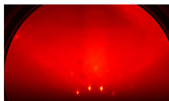
RHEED
