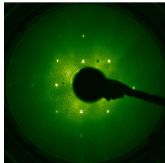
LEED @ 200 eV
