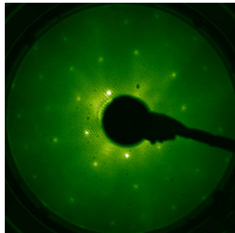
LEED @ 250 eV
