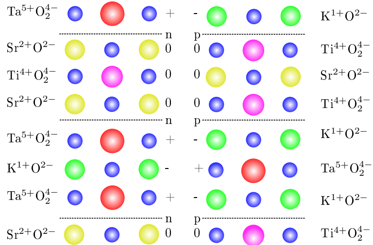
Figure 9.2: Used p- and n-type superlattices for calculation. The stacking sequence determines the charge at the interface. The charge arises from the charged \text{TaO}_2 and \text{KO} layers. The STO layers are neutral. As the whole system has to be neutral, the interface has to compensate the surplus charges by introducing electrons or holes to the interface. Adapted from [2].
