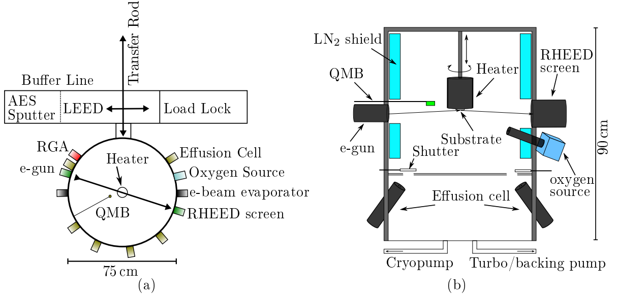
Figure 4.2: (a) Bird's eye view of the used system. The system is divided into three sections. The load lock, the buffer line, and the main chamber. A transfer system allows one to move the sample within the system. The main chamber, or growth chamber, is equipped with two electron beam evaporators and six effusion cells. In total up to eight elements can be evaporated simultaneously. (b) depicts a cross section of the main chamber to see the arrangement of the equipment that is necessary for sample growth. The substrate is mounted upside-down on a heater. The oxygen source and the evaporators can be closed with shutters. Both sketches are not true to scale. AES: Auger electron spectroscopy, QMB: quartz microbalance, LEED: low energy electron diffraction, RHEED: reflection high energy electron diffraction, RGA: residual gas analyzer.
