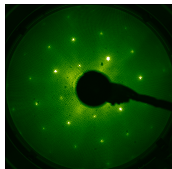
LEED @ 200 eV
