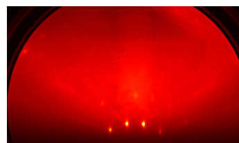
RHEED
