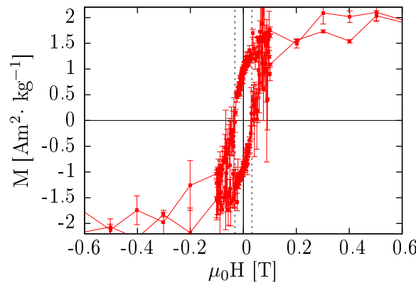
Figure 6.34: A M-H -curve measured at 110 K after field-cooling in 20 mT along [100]. The dotted lines are describing the coercive field H_{\text{C}} . The opening of the hysteresis hints a ferromagnetic component.
