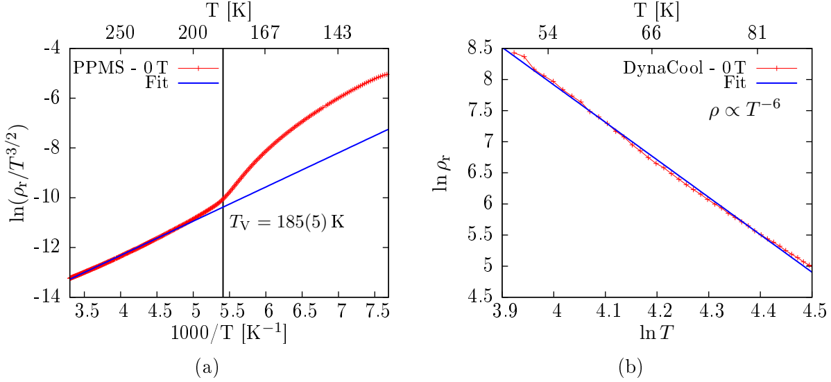
Figure 6.38: (a) Replot of the data in order to fit the non-adiabatic small polaron model. The vertical line indicates the position of the transition temperature T_V . (b) Double ln plot to determine the power law eq. 6.7 according to [40]. The used temperature range was selected to be far below the transition temperature.
