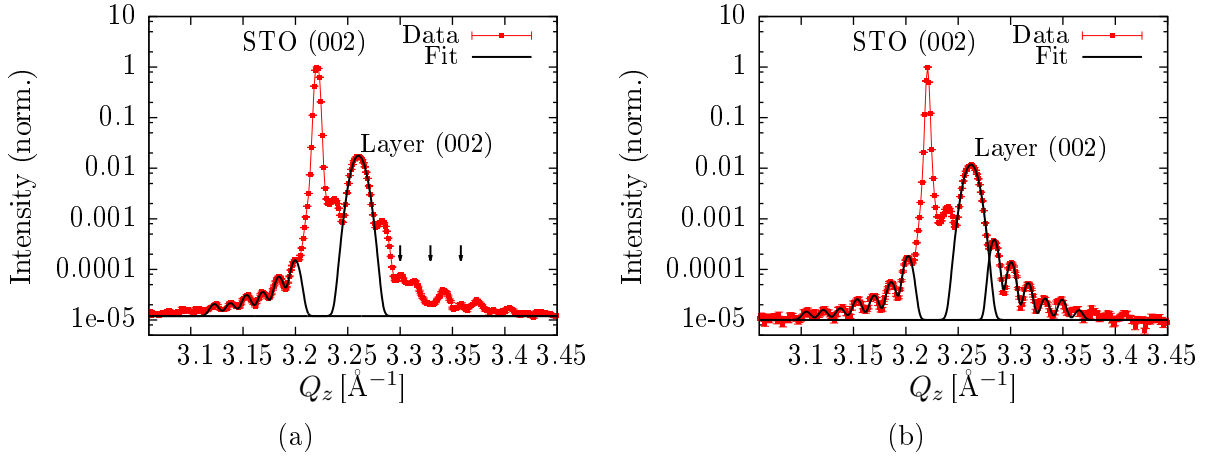
Figure 8.4: (002) - measurement of sample LSMOfinal (a) and LSFOfinal (b). A \theta_0 correction was applied. The thickness oscillations were analyzed by applying a sum of Gaussians, which consider the distance between oscillations as a parameter. The thickness oscillations are attributed to the total thickness. However, in (a) a second period was found (see arrows), which is identified as oscillations caused by the single layers. The arrows point to the minima of the second oscillations indicating a destructive interference which extinct the bilayer oscillation significantly.
