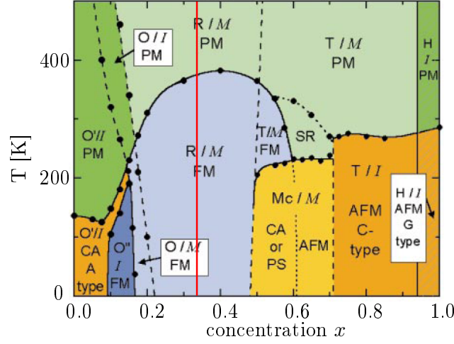
Figure 7.1: Structural, magnetic, and electronic phase diagram of \text{La}_{1-x}\text{Sr}_x\text{MnO}_3 from Hemberger et al.. The concentration used here is x = \frac{1}{3} , which exhibit a rhombohedral crystal structure, and is a metallic-like ferromagnetic material with a bulk T_c of 370 K. The symbols in the diagram are orthorhombic O, rhombohedral R, tetragonal T, monoclinic Mc, hexagonal H; insulating I, metallic M; ferromagnetic FM, antiferromagnetic AFM, paramagnetic PM. Reprinted from [13], with the permission of AIP publishing.
