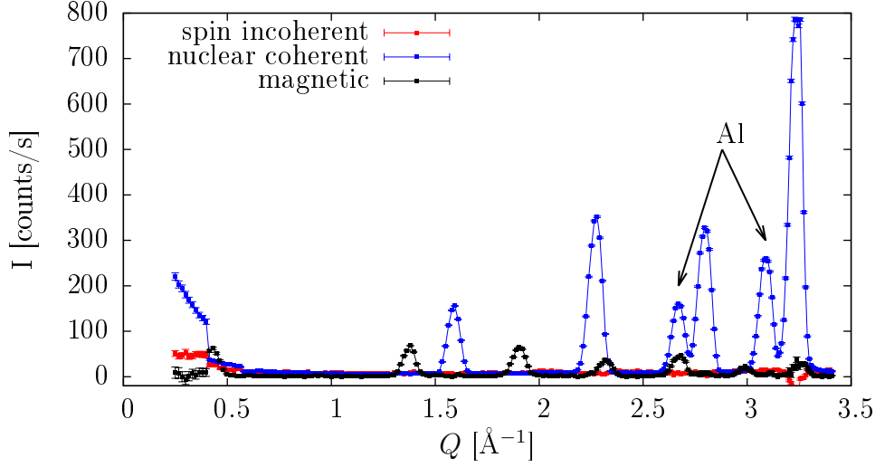
Figure 6.12: DNS measurement performed at 5 K without self-normalization. Separation of the different contributions has been done with dnsploot. Additionally, the two labeled reflections are Al (111) and (200). Aluminium has been used as sample holder and sample environment.
