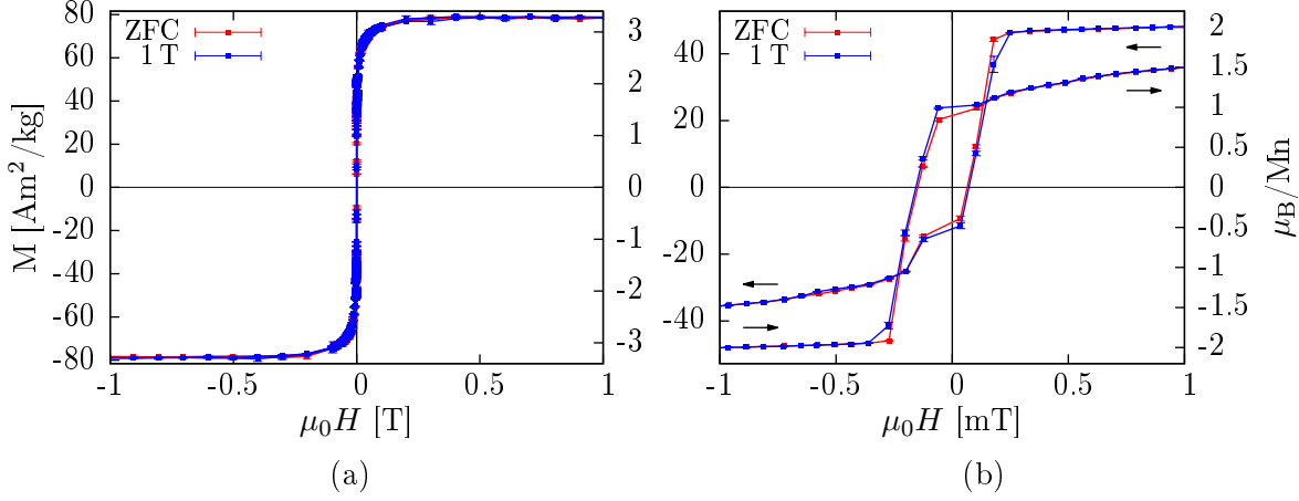
Figure 8.11: M - H - measurements of LSFO final after zero-field-cooling and field-cooling in 1 T applied along [001] at 110 K. The measurement was done between \pm 1 T as shown in (a). The closer look depicted in (b) revealed an unusual behavior, known as inversed magnetic hysteresis.
