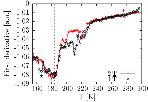
Figure 6.37: First derivative of measurement shown in Fig. 6.36b. The minimum of the derivative corresponds to the Verwey transition temperature. The less significant minima are measurement artifacts. A moving window derivative has been used.
