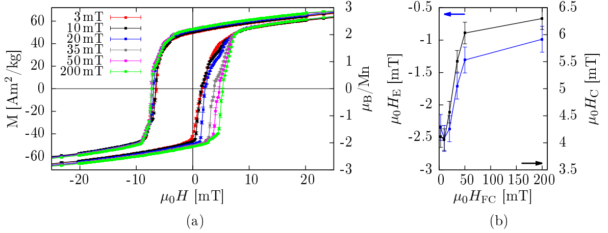
Figure 8.12: M - H - measurements at 10 K of LSFOfinal after field-cooling. The measurement was done from \pm 1 T starting from positive field. A zoom on an interesting region is given in (a). (b) shows field-cooling field dependence in the exchange bias field and coercive field, respectively. The coercive field is defined as H_C = (H_{C2} - H_{C1})/2 and is used to compare the different measurements.
