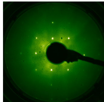
LEED @ 200 eV
