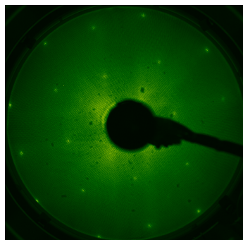
LEED @ 100 eV
