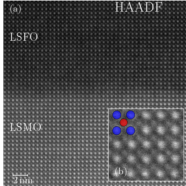
Figure 8.5: HAADF-STEM image of the well-ordered interface region of sample LSFOfinal in (a). The interface is not sharp, but is slightly wavy and buckled. The inset (b) is a magnification to identify the perovskite structure with its A- and B-sites as indicated by colored spheres.
