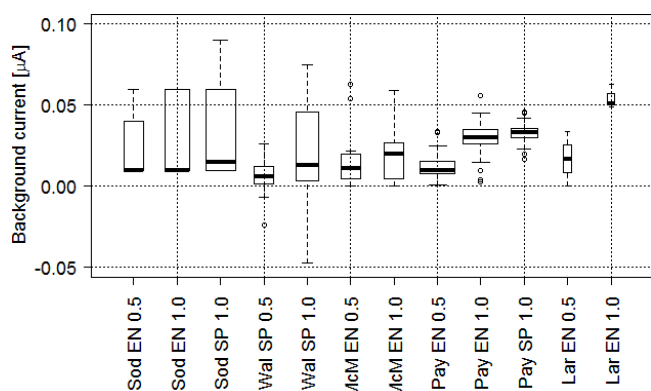
Figure 1. Boxplot of the background current ( \mu\text{A} ) measured at the five stations which flew a number of dual- or multi-ozonesonde gondolas: Sodankylä (Sod), Wallops Island (Wal), McMurdo Station (McM), Payerne (Pay), and Laramie (Lar). Following the station location, the ozonesonde manufacturer (EN or SP) and then the KI solution concentration (0.5 or 1.0 %) are identified. Medians are the thick black segments, the interquartile range is the box height, 1.5 times the interquartile range are the whiskers, outliers are denoted as circles, and the square root of the number of measurements is reflected in the box width. A value of 0.03 \mu\text{A} corresponds to 0.1 \text{ mPa} of ozone.
