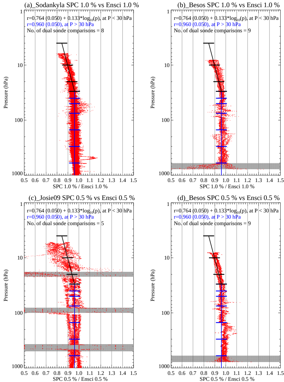
Figure 7. Vertical profiles of ratios of ozone partial pressure using ozonesondes of different manufacturer (SP, EN) with the same KI concentrations in both ozonesondes, either 1.0 % (a, b) or 0.5 % (c, d). (a) Sodankylä – 1.0 %; (b) BESOS – 1.0 %; (c) JOSIE09 – 0.5 %; (d) BESOS – 0.5 %. The hashed areas denote regions of low ozone concentration in tests in the laboratory during JOSIE09, or during initial problems with the BESOS data system. Fits to the data using the transfer functions from Eq. (6), and included at the top of each panel, are shown in blue and black. The numbers in parentheses behind each slope are the uncertainties of the fit.
