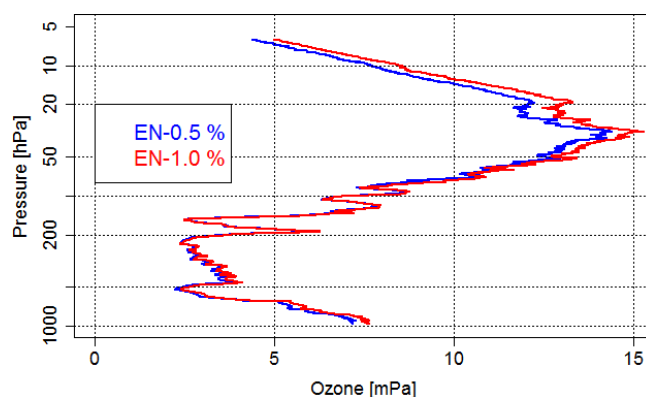
Figure 4. Example of the results of a dual-ozonesonde flight profile from Payerne. The only difference between the ozonesondes is the KI solution concentration.
