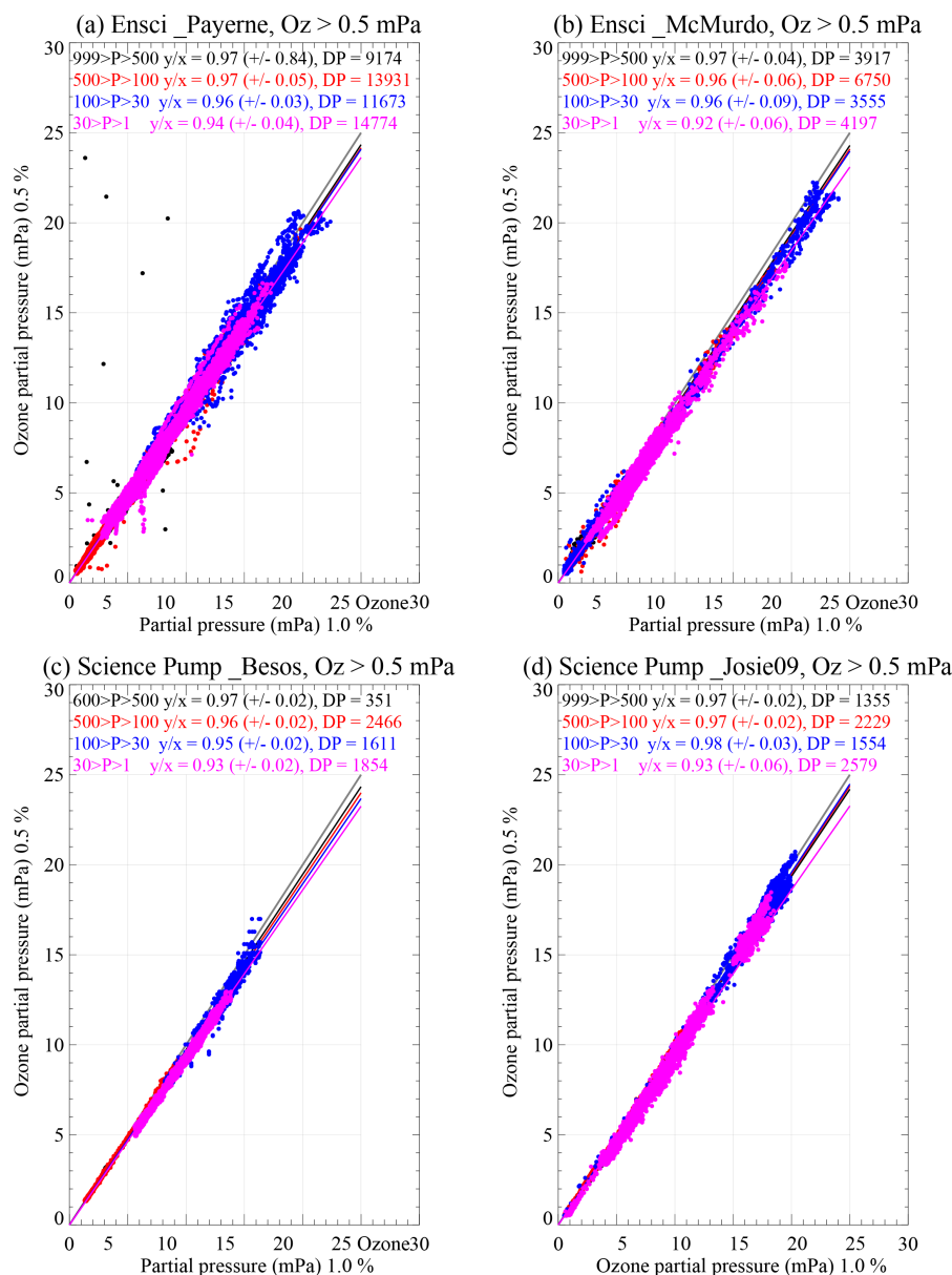
Figure 5. Scatterplots of ozone partial pressures measured with KI concentrations of 1.0 % ( x axis) and 0.5 % ( y axis) using EN ozonesondes flown from (a) Payerne and (b) McMurdo Station, and with SP ozonesondes from (c) BESOS and (d) JOSIE09. The data are subdivided into four pressure intervals, and averages and standard deviations of the ratios of y : x are listed on the panels along with the number of measurements (noted as DP for data points). Only ozone measurements above 0.5 mPa are included. At p \geq 30 hPa there is little variation in the ratios by pressure interval, location, or ozonesonde type. At p < 30 hPa ratios are decreasing. The 1 : 1 line is shown in gray.
