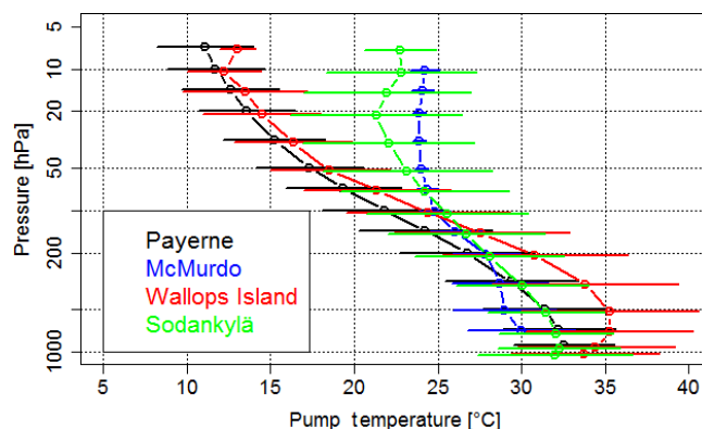
Figure 3. Mean profile of the measured pump temperature for the different dual-ozonesonde flight data sets. The higher pump temperature at the upper part of the profiles for the McMurdo and Sodankylä stations is due to a heat source to avoid freezing of the solution. Error bars are 1 standard deviation of the measurements.
