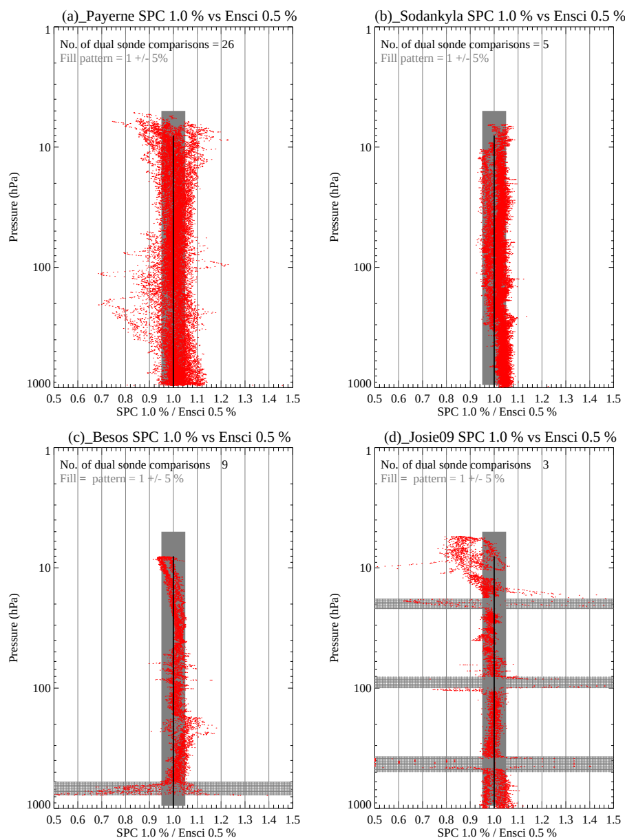
Figure 8. Ratios of SP-1.0 % to EN-0.5 % ozonesondes. The measurements are from (a) Payerne, (b) Sodankylä, (c) BESOS, and (d) JOSIE 2009. The filled regions represent 5 % around 1.0. The hashed areas are as before to indicate regions of low ozone concentration during tests in JOSIE 2009 or difficulty with the data system in BESOS.
