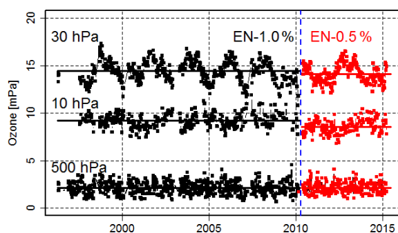
Figure 9. Ozone time series from the Nairobi station at three pressure levels: 500, 30, and 10 hPa. The black symbols correspond to the data from 1996 to 2010 (EN-1.0 % solution), and the red symbols from 2010 onwards (EN-0.5 %). The horizontal segments are the mean values over the two periods. No corrections to the EN-1.0 % data have been made for this figure.
