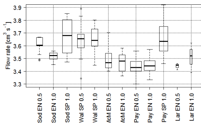
Figure 2. Ozonesonde pump flow rates ( \text{cm}^3 \text{s}^{-1} ) measured at the different stations, following the nomenclature of Fig. 1 for the station and ozonesonde.
