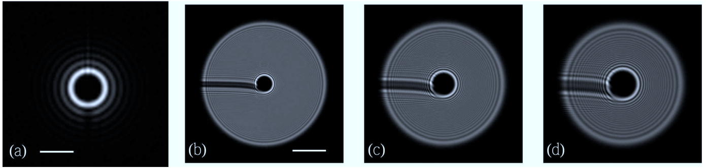
Fig. 5. Simulated images generated for line charges of length 100 \mu\text{m} and a potential difference of 20 V. (a) Fraunhofer diffraction image (scale bar 0.5 \mu\text{m}^{-1} ). (b) – (d) show Fresnel images (scale bar 5 \mu\text{m} ) for defocus values Z of 2, 4 and 6 cm, respectively.
