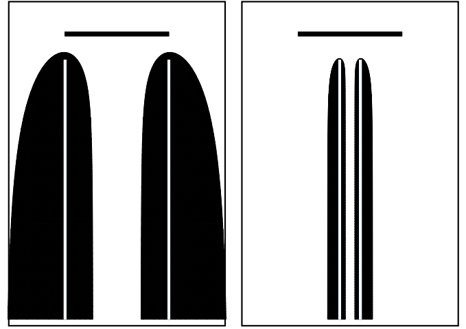
Fig. 1. Line charges of length 100 \mu\text{m} and separation 200 nm (white lines) with constant charge densities of C_V = 1 . The overlaid amplitude images (black outlines) show corresponding \pm 2 V potential surfaces. The left image (scale bar 200 nm) shows the region around the tips. The right image shows a wider area (scale bar 1 \mu\text{m} ).
