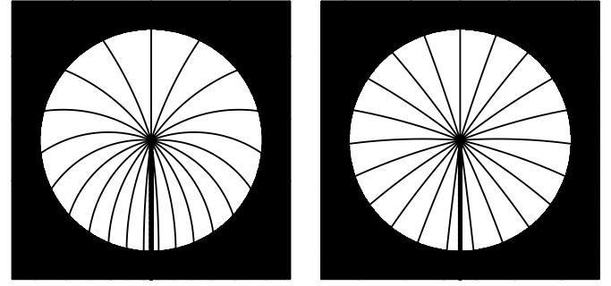
Fig. 3. Equipphase lines of spacing \pi/4 radians and overlaid amplitude image, shown for a 25 \mu\text{m} \times 25 \mu\text{m} field of view. The left image corresponds to line charges of length 20 \mu\text{m} . The right image corresponds to line charges of length 100 \mu\text{m} . A beam-limiting aperture of diameter 20 \mu\text{m} is also shown.
