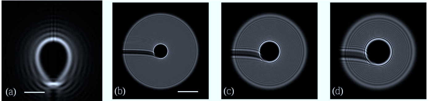
Fig. 7. Simulated images generated for line charges of length 20 \mu\text{m} and a potential difference of 40 V. (a) Fraunhofer diffraction image (scale bar 0.5 \mu\text{m}^{-1} ). (b) – (d) show Fresnel images (scale bar 5 \mu\text{m} ) for defocus values Z of 2, 4 and 6 cm, respectively.
