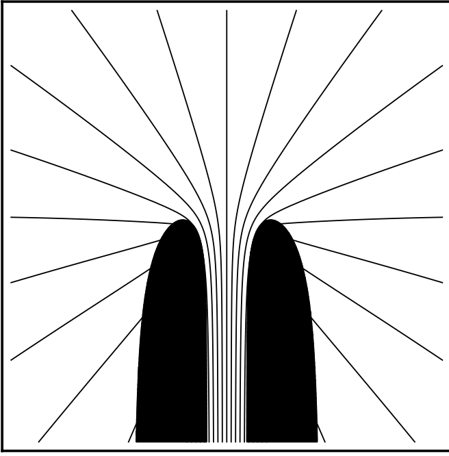
Fig. 2. Equipphase lines of spacing \pi/4 radians and overlaid amplitude image, shown for a 1 \mu\text{m} \times 1 \mu\text{m} field of view, a wire length of 100 \mu\text{m} and a wire separation of 200 \text{ nm} .
