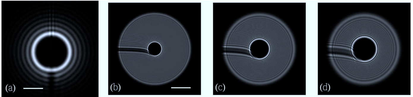
Fig. 6. Simulated images generated for line charges of length 100 \mu\text{m} and a potential difference of 40 V. (a) Fraunhofer diffraction image (scale bar 0.5 \mu\text{m}^{-1} ). (b) – (d) show Fresnel images (scale bar 5 \mu\text{m} ) for defocus values Z of 2, 4 and 6 cm, respectively.
