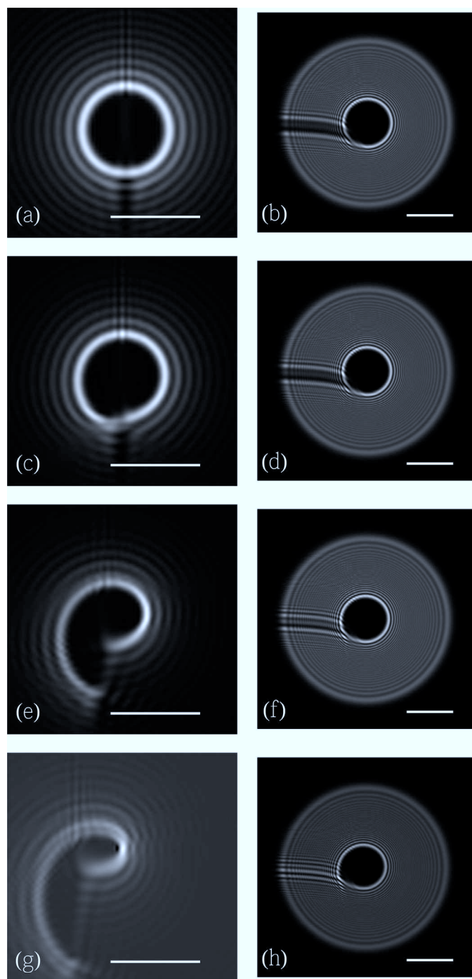
Fig. 8. Simulated Fraunhofer images (left) and Fresnel images (right) generated for line charges of length 100 \mu\text{m} , a potential difference of 40 V and added potentials of (a, b) 0 V, (c, d) 0.01 V, (e, f) 0.05 V and (g, h) 0.1 V. The Fresnel images were calculated for a defocus value Z of 4 cm. The scale bar in the diffraction images (a, c, e, g) is 0.5 \mu\text{m}^{-1} . The scale bar in the Fresnel images (b, d, f, h) is 5 \mu\text{m} .
