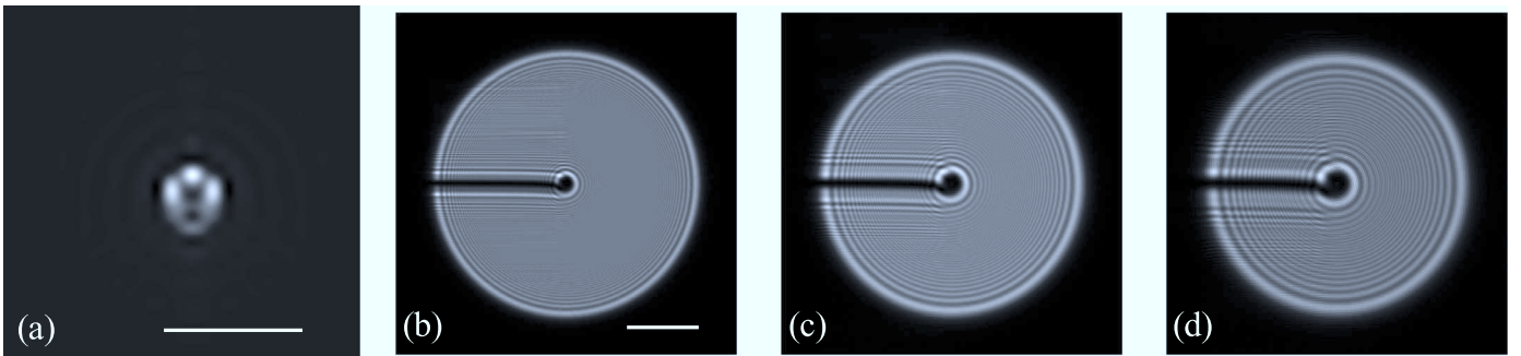
Fig. 4. Simulated images generated for line charges of length 100 \mu\text{m} and a potential difference of 4 \text{ V} . (a) Fraunhofer diffraction image (scale bar 0.5 \mu\text{m}^{-1} ). (b) - (d) show Fresnel images (scale bar 5 \mu\text{m} ) for defocus values Z of 2, 4 and 6 \text{ cm} , respectively.
