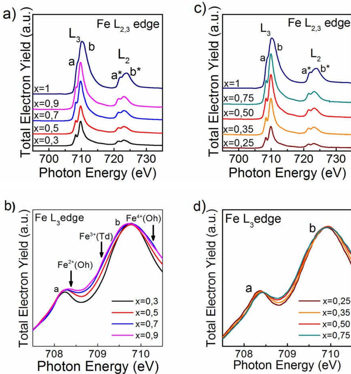
Figure 2. Fe 2p (L 2,3 )- absorption spectra of the SrTi 1-x Fe x O 3-δ (STFO) samples with different content of Fe on B-site of perovskite structure: (a-b) a first group of samples with x: 0.3, 0.5, 0.7 and 0.9 of Fe atoms produced by spray pyrolysis method; (c-d) a second group of samples with x: 0.25, 0.35, 0.50 and 0.75 of Fe
