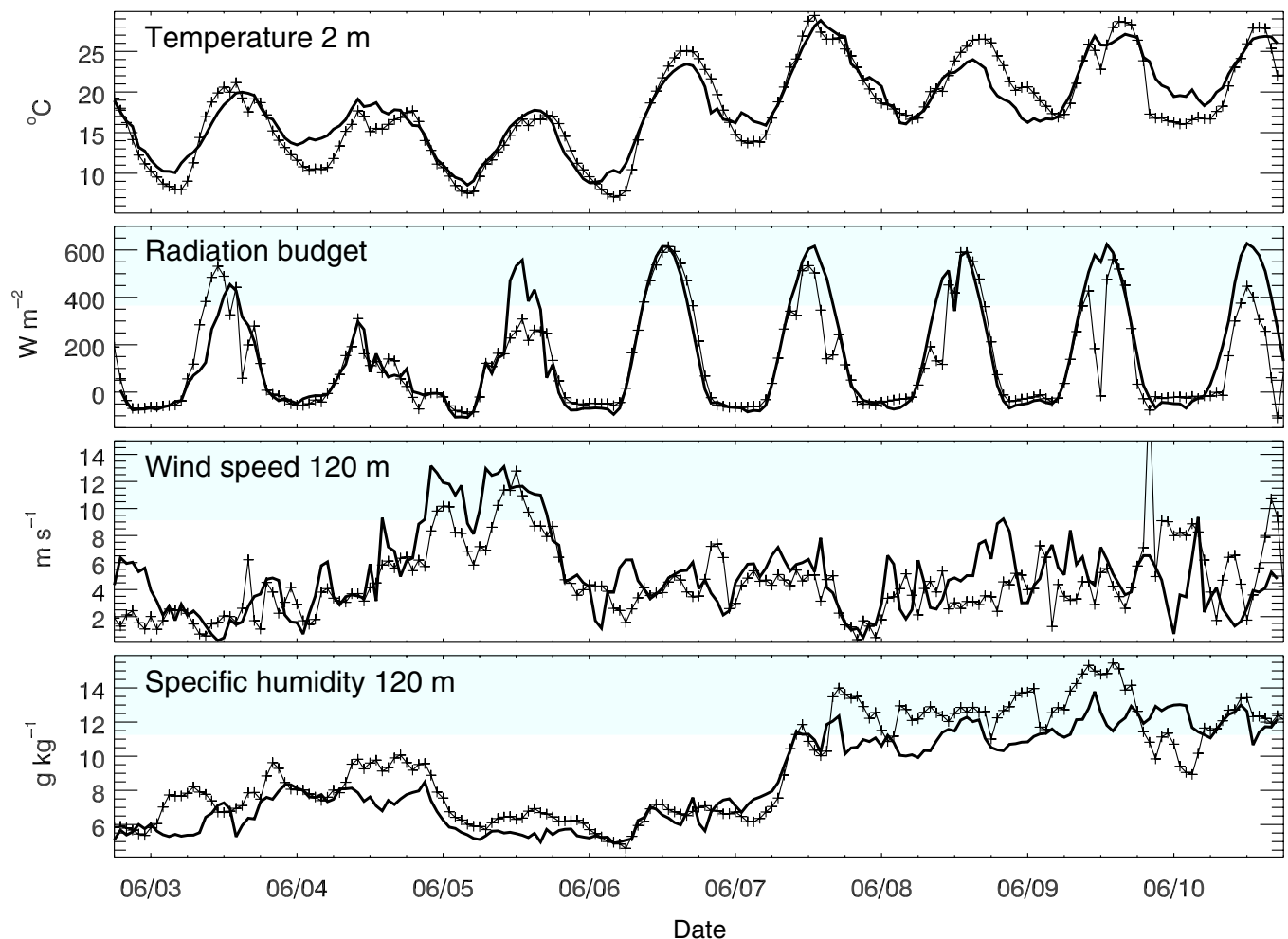
Figure 5. Comparison of simulated (thick solid lines) and observed (crosses) temperature (°C) at 2 m, total radiation budget ( \text{W m}^{-2} ), wind speed ( \text{m s}^{-1} ) and specific humidity ( \text{g kg}^{-1} ) at the Jülich tower between 3 and 10 June 2014.
