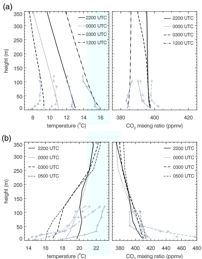
Figure 9. Vertical profiles of temperature (°C) and CO 2 mixing ratios (ppmv) at the Jülich tower at different times of (a) ‘day 1’ (2200 UTC on 4 June to 1200 UTC on 5 June 2014) and (b) ‘day 2’ (2200 UTC on 6 June to 0500 UTC on 7 June 2014). Black lines: simulated profiles, grey lines: observed profiles. The crosses indicate the heights of the tower observations.
