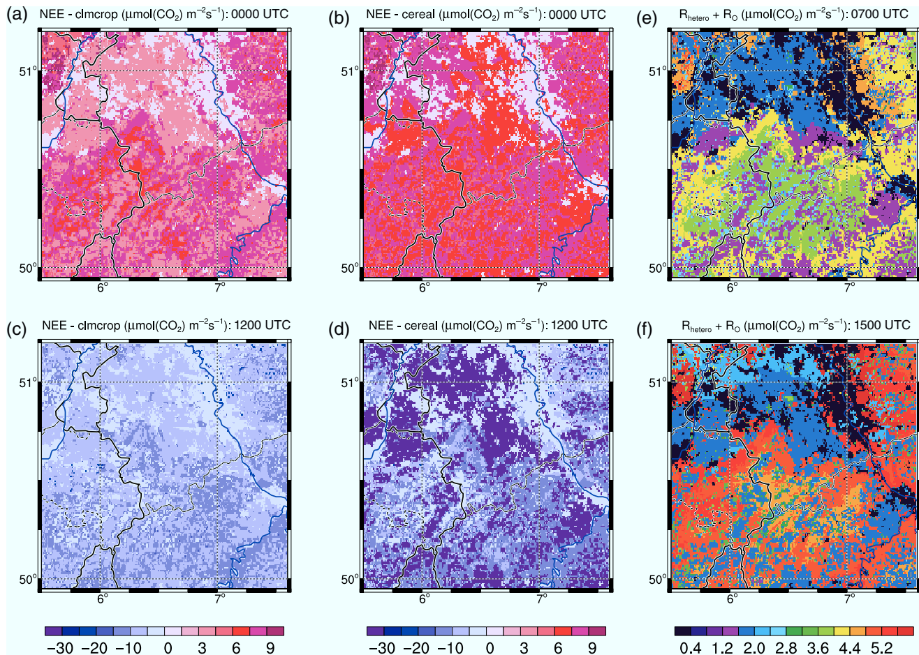
Figure 10. Simulated NEE ( \text{mol}(\text{CO}_2) \text{ m}^{-2} \text{ s}^{-1} ) on 26 May 2012 at (a, b) 0000 UTC and (c, d) 1200 UTC for the (a, c) ‘clmcrop’ and the (b, d) ‘cereal’ simulation. (e, f) show the total heterotrophic respiration ( R_{\text{hetero}} + R_{\text{O}} ) ( \text{mol}(\text{CO}_2) \text{ m}^{-2} \text{ s}^{-1} ) at (e) 0700 UTC and (f) 1500 UTC.
