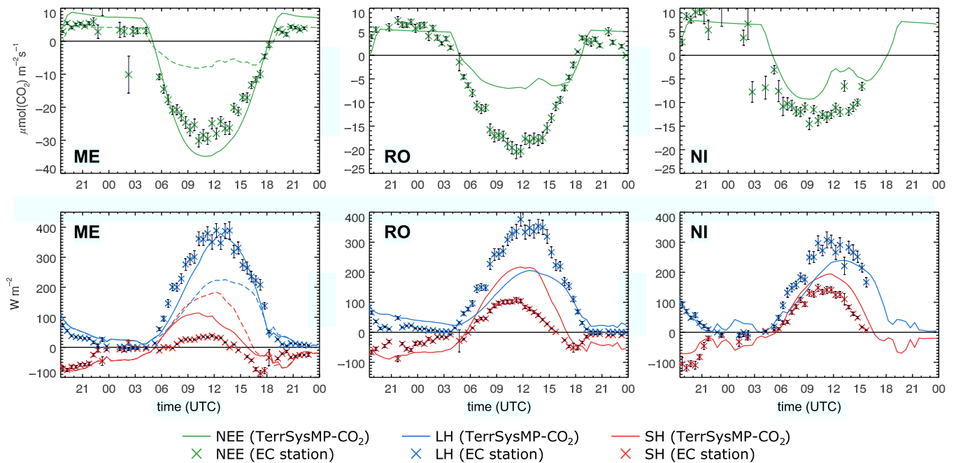
Figure 11. Comparison of simulated NEE ( \mu\text{mol}(\text{CO}_2) \text{m}^{-2} \text{s}^{-1} ), LH and SH fluxes ( \text{W m}^{-2} ) with EC fluxes at Merzenhausen (ME, winter wheat), Rollesbroich (RO, grassland) and Niederzier (NI, grassland) between 1800 UTC on 25 May and 0000 UTC on 27 May 2012. At Merzenhausen the solid lines correspond to the ‘cereal’ simulation and the dashed lines to the ‘clmcrop’ simulation. The error bars denote the random errors of the measurements.
