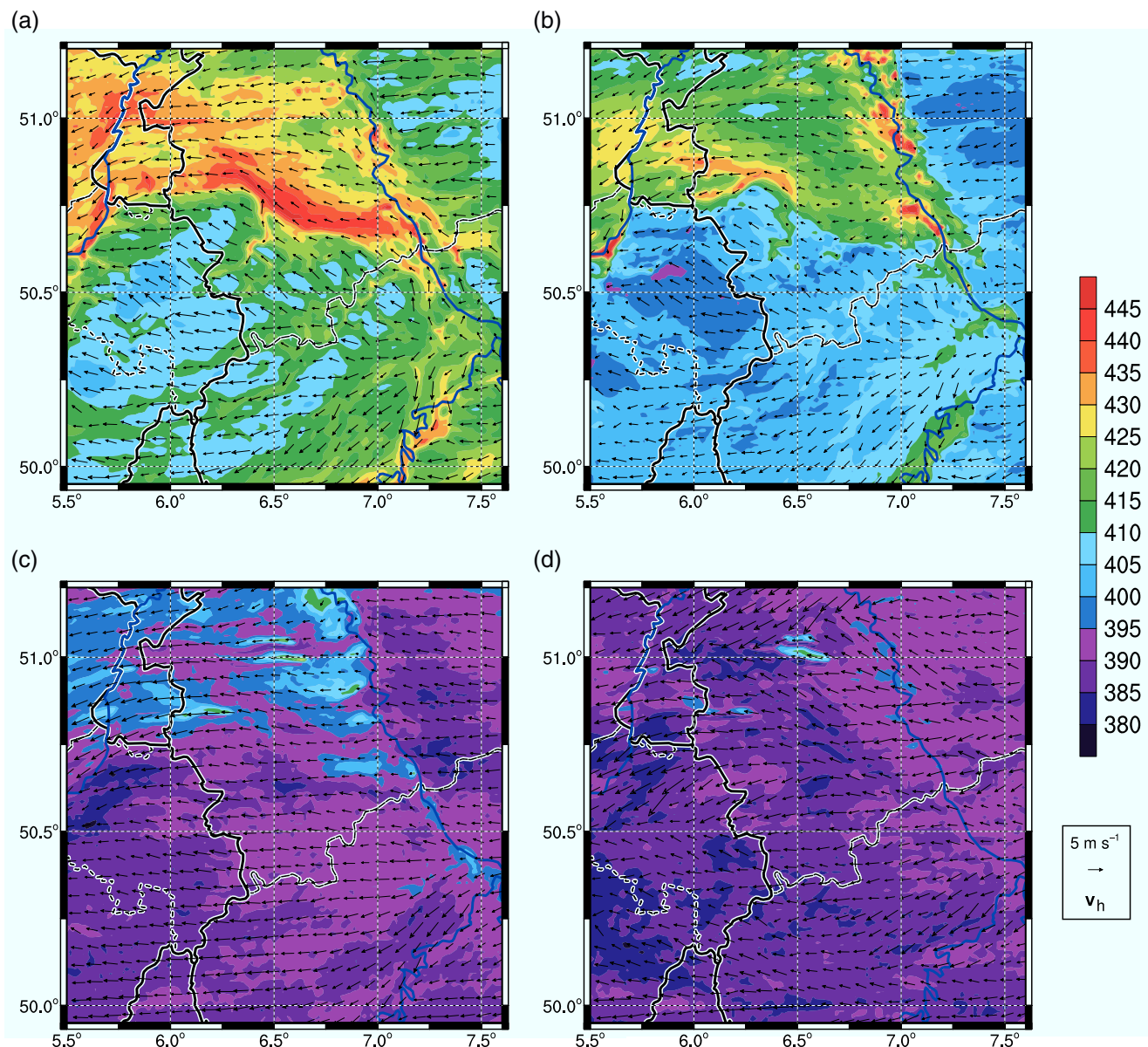
Figure 13. Simulated \text{CO}_2 mixing ratios (ppmv, shading) and horizontal wind ( \text{m s}^{-1} , arrows) at the lowest COSMO level ( \approx 10 m agl) on 26 May 2012 ('cereal' simulation): (a) 0400 UTC, (b) 0600 UTC, (c) 0900 UTC, (d) 1600 UTC.
