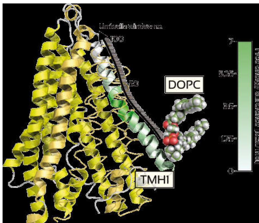
Fig. 3: Free energy difference between spontaneous DOPC flip-flop and DOPC flip-flop along TMH1 in MDR3, with positive values on the color scale indicating a more disfavorable process for spontaneous DOPC flip-flop. The color coding on TMH1 reflects the free energy difference given in the color scale when the head group of DOPC is near the very C \alpha atom. The largest difference is observed in the membrane center.
