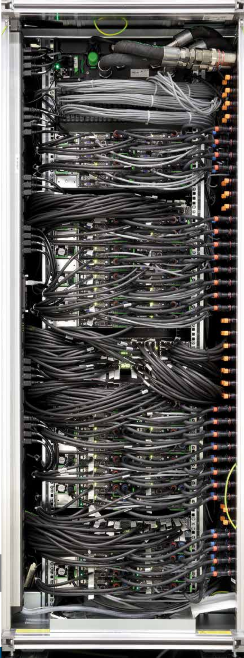
Single QPACE 3 rack with a water manifold at the right side, which is connected to a heat exchanger in the top of the rack.
