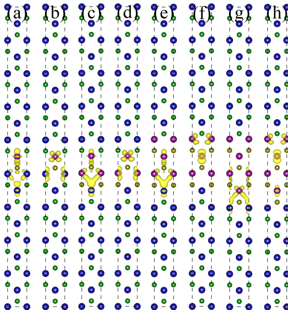
Figure 4. VBM and CBM at the A-point for \text{WS}_2/\text{MoSe}_2/\text{WS}_2 quantum well with different \text{MoSe}_2 thickness of n = 1-4 . (a,c,e,g) represent the VBM, while (b,d,f,h) indicate the CBM. The small spheres are non-metal atoms (S and Se), while big spheres are metal atoms (Mo and W).
