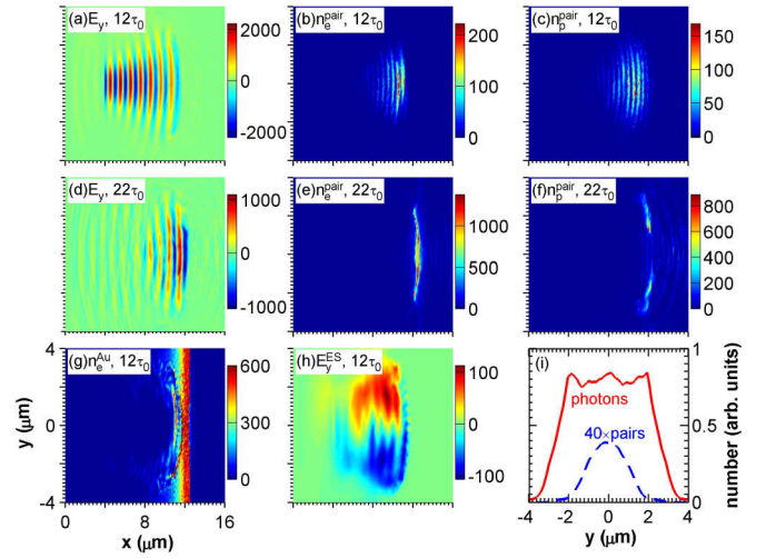
FIG. 3. Snapshots of (a), (d) laser electric fields eE_y/m_e\omega_0 c , (b), (e) pair-plasma electron densities n_e^{\text{pair}}/n_c , (c), (f) positron densities n_p^{\text{pair}}/n_c at different times, (g) Au-target electron density n_e^{\text{Au}}/n_c , and (h) electrostatic field eE_y^{\text{ES}}/m_e\omega_0 c , where the maximum value is suppressed in (g) for clarity. (i) Number of generated photons and pairs vs their transverse position y , where the pair number is scaled by a factor of 40.
