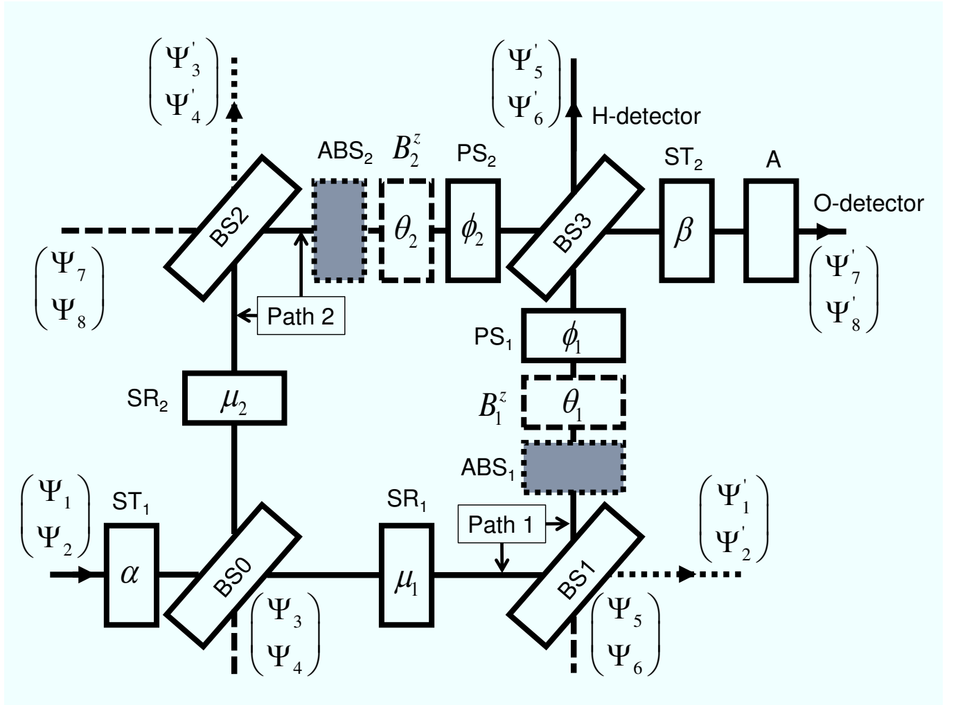
FIG. 5. Schematic diagram of the theoretical model of the Cheshire Cat single-neutron interferometry experiment [10] depicted in Fig. 1. Polarized neutrons with their magnetic moments aligned along the z -axis (defined by a guiding magnetic field, not shown) and oriented in the +z -direction enter the spin turner ( ST_1 ) which rotates the neutron magnetic moment such that it is aligned along the +x direction ( \alpha = \pi/2 ). BS_0, \dots, BS_3 : beam splitters. SR_1 and SR_2 : rotation of the magnetic moment about the z -axis by angles \mu_1 = 0 and \mu_2 = \pi , respectively. ABS_1 and ABS_2 : absorbers with transmissivity T_1 and T_2 which may be present in path 1 or path 2, respectively. B_1^z and B_2^z : local magnetic fields, rotating the magnetic moment by \theta_1 and \theta_2 , respectively. PS_1 and PS_2 : phase shifter causing a phase shift of \phi_1 and \phi_2 on neutrons passing via path 1 and path 2, respectively. ST_2 : spin turner with its magnetic field aligned along the y -axis, rotating the magnetic moment by an angle \beta about the y -axis. A : spin analyzer which passes neutrons with their magnetic moments aligned along the +z -axis only. The two-dimensional vectors (\Psi_{2j-1}, \Psi_{2j})^T and (\Psi'_{2j-1}, \Psi'_{2j})^T with j = 1, \dots, 4 are used in the quantum theoretical description, see Eq. (A1)
