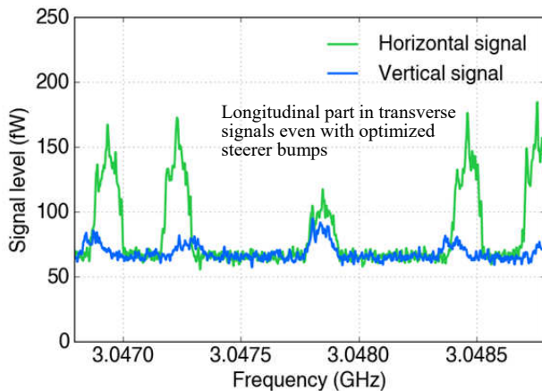
Figure 3: Transverse sidebands with 8 \cdot 10^8 particles.
