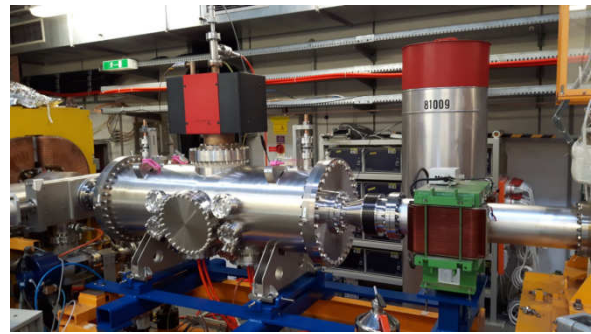
Figure 4: First HESR kicker installed at COSY.
