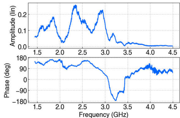
Figure 5: Amplitude (top) and phase (bottom) of system's hardware transfer function.
