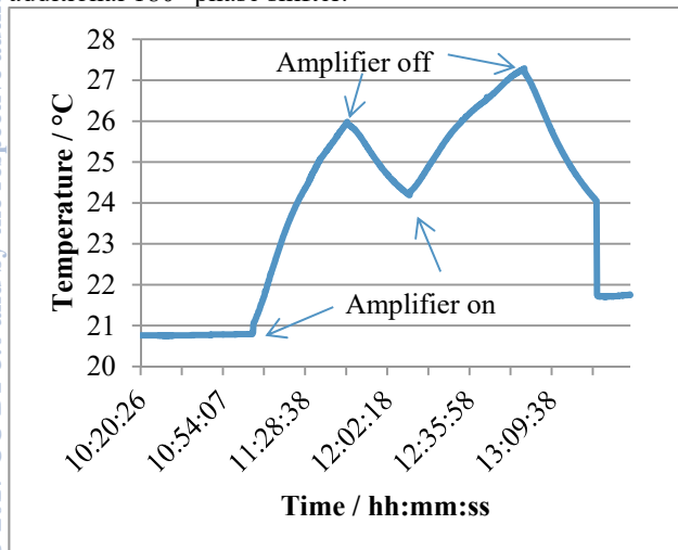
Figure 8: Temperature at combiner-board.
