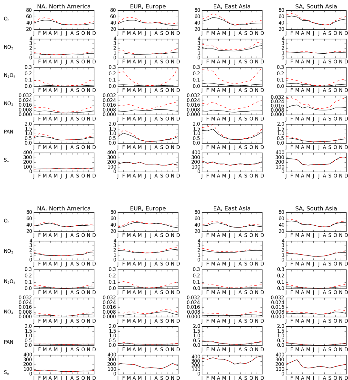
Figure 5. Changes in O_3 , NO_2 , N_2O_5 , NO_3 , PAN and S_a for the base-case (solid black line) and noN2O5 case (dashed red line) for EMEP (top) and ECHAM-HAMMOZ (bottom). Plots show monthly gas phase mixing ratios in ppbv and surface area density in \mu m^2 cm^{-3} for different regions as defined above.
